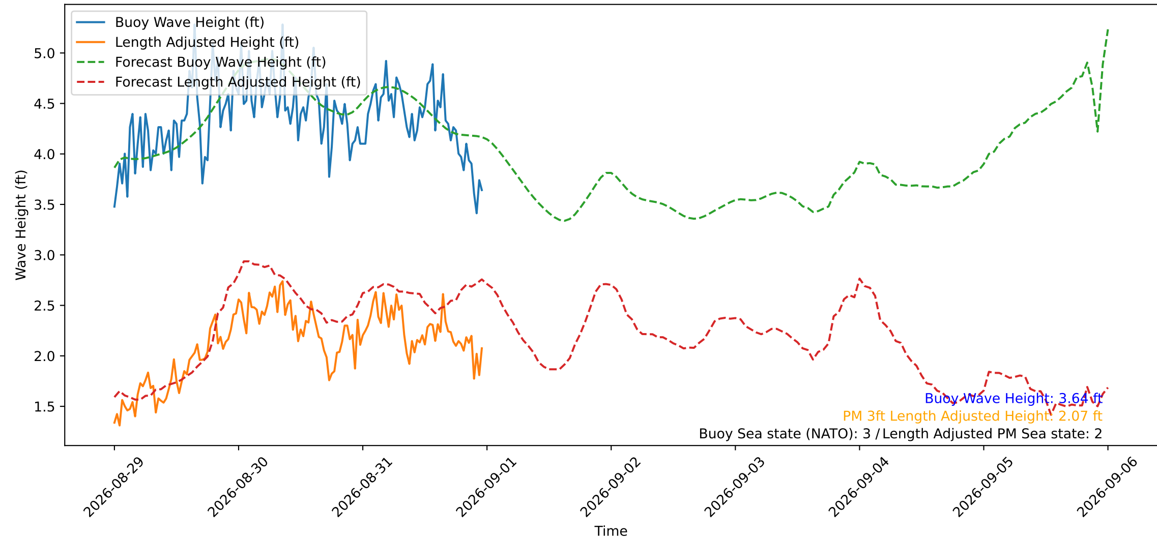
Wave Heights over Time for Oceanside Harbor at 2026-08-31 23:50:30
