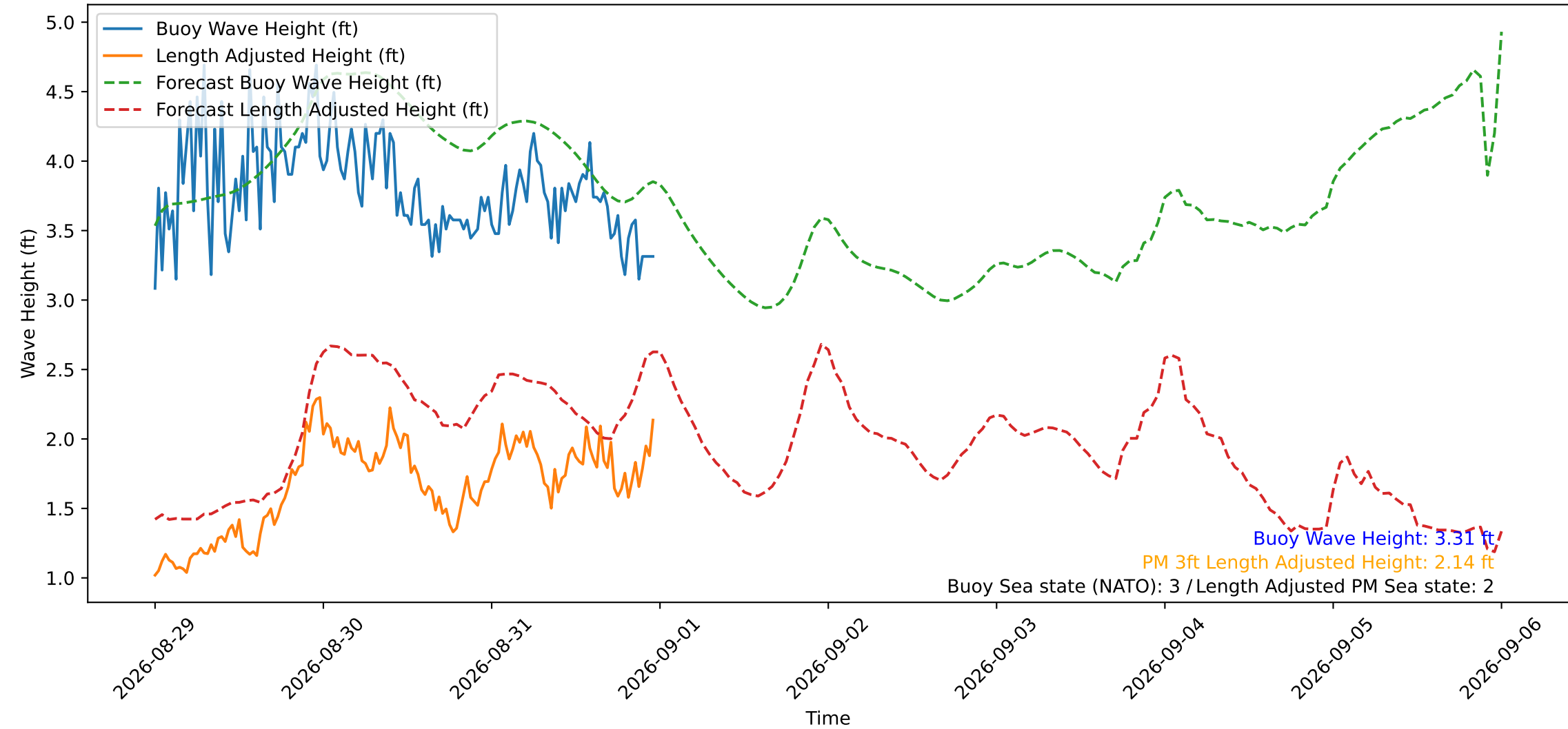
Wave Heights over Time for Red Beach at 2026-08-31 23:50:50
