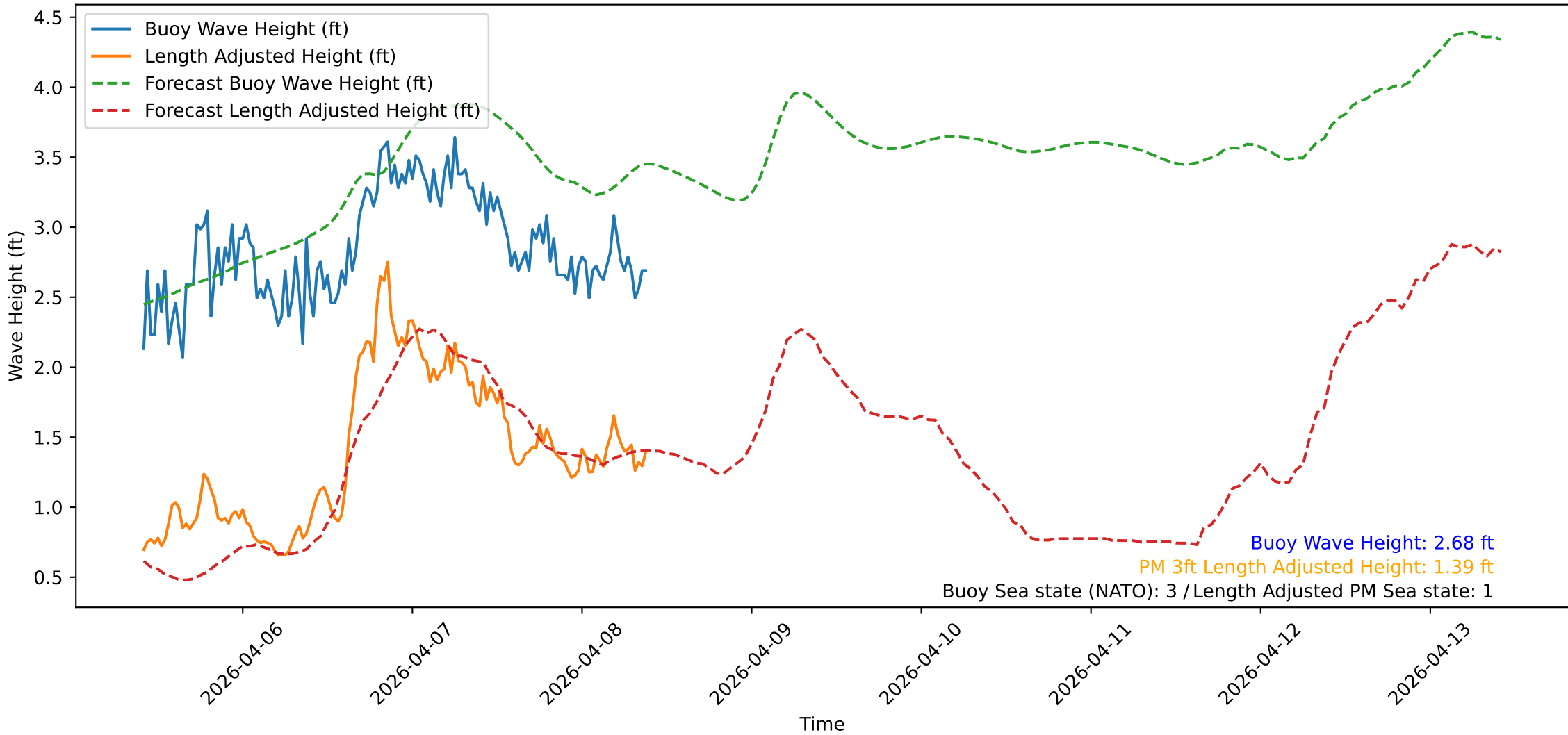
Wave Heights over Time for Oceanside Harbor at 2026-04-08 09:50:31
