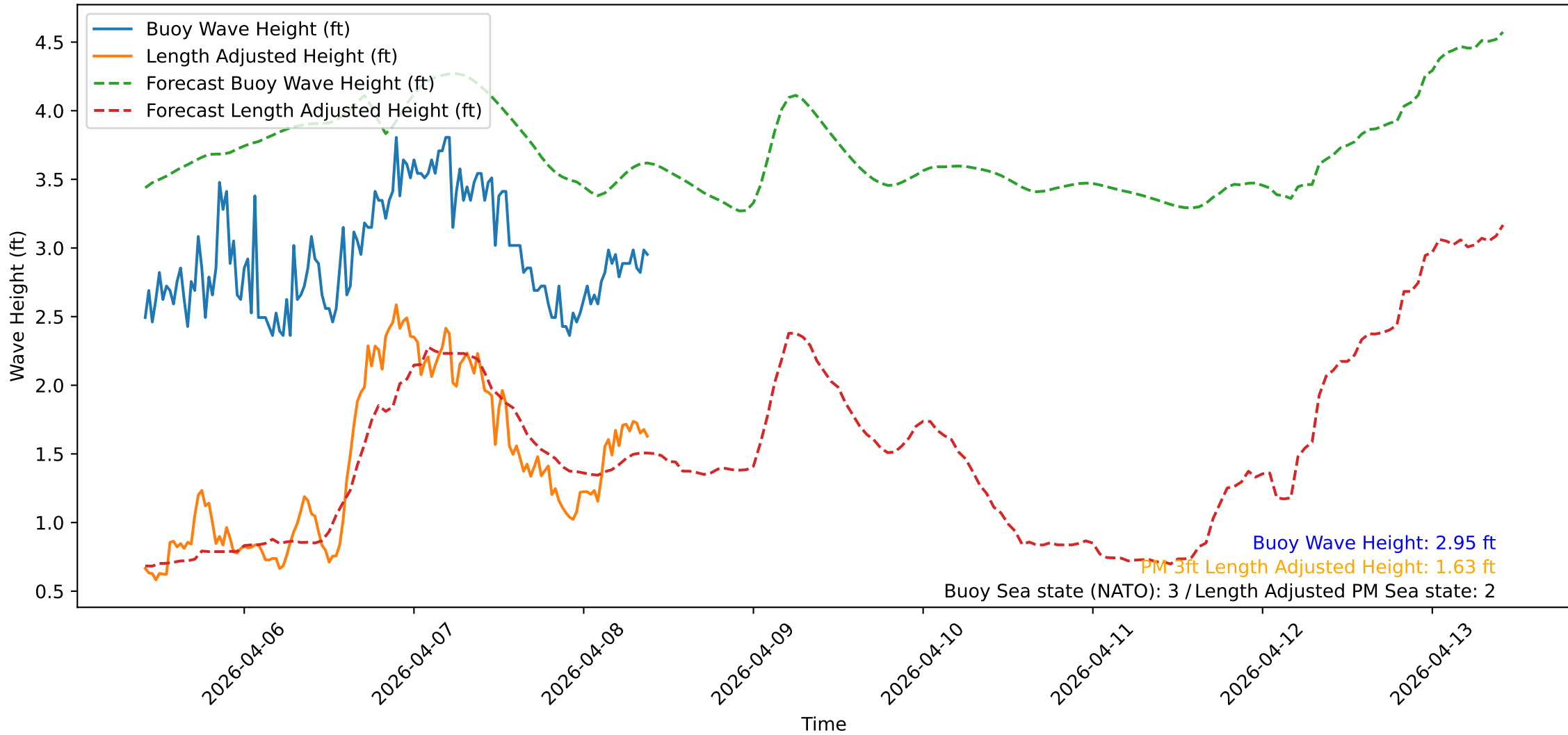
Wave Heights over Time for Green Beach at 2026-04-08 09:51:21
