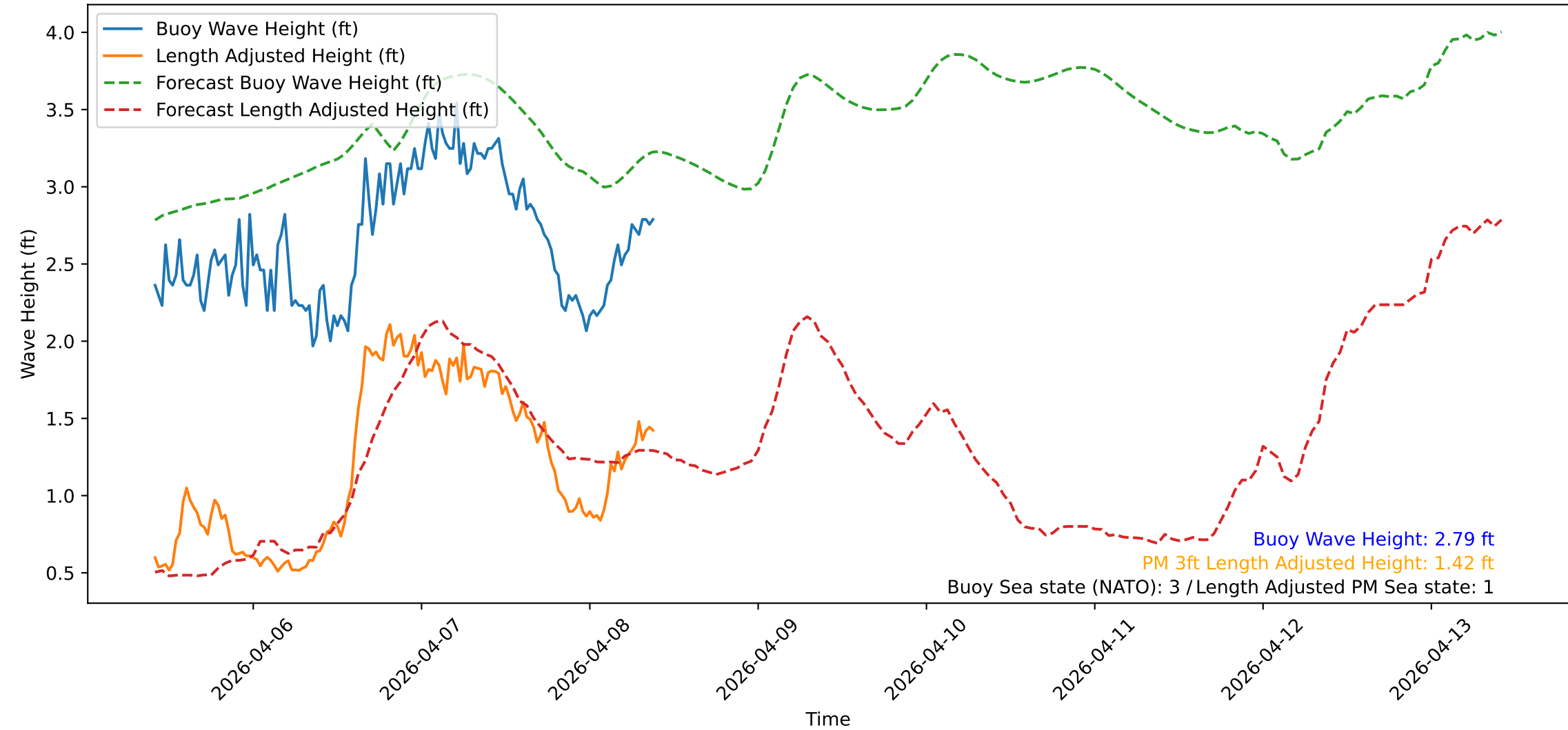
Wave Heights over Time for Red Beach at 2026-04-08 09:50:57
