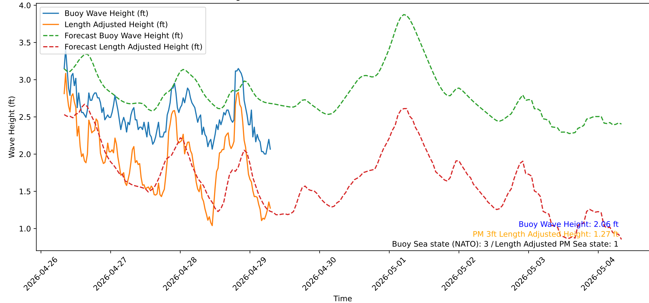
Wave Heights over Time for Green Beach at 2026-04-29 07:51:14
