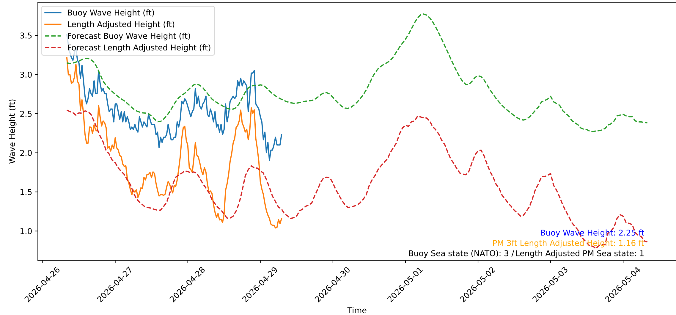
Wave Heights over Time for Oceanside Harbor at 2026-04-29 07:50:31
