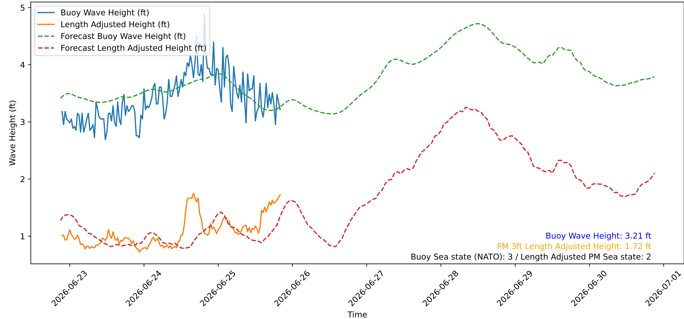
Wave Heights over Time for Oceanside Harbor at 2026-06-25 21:20:25
