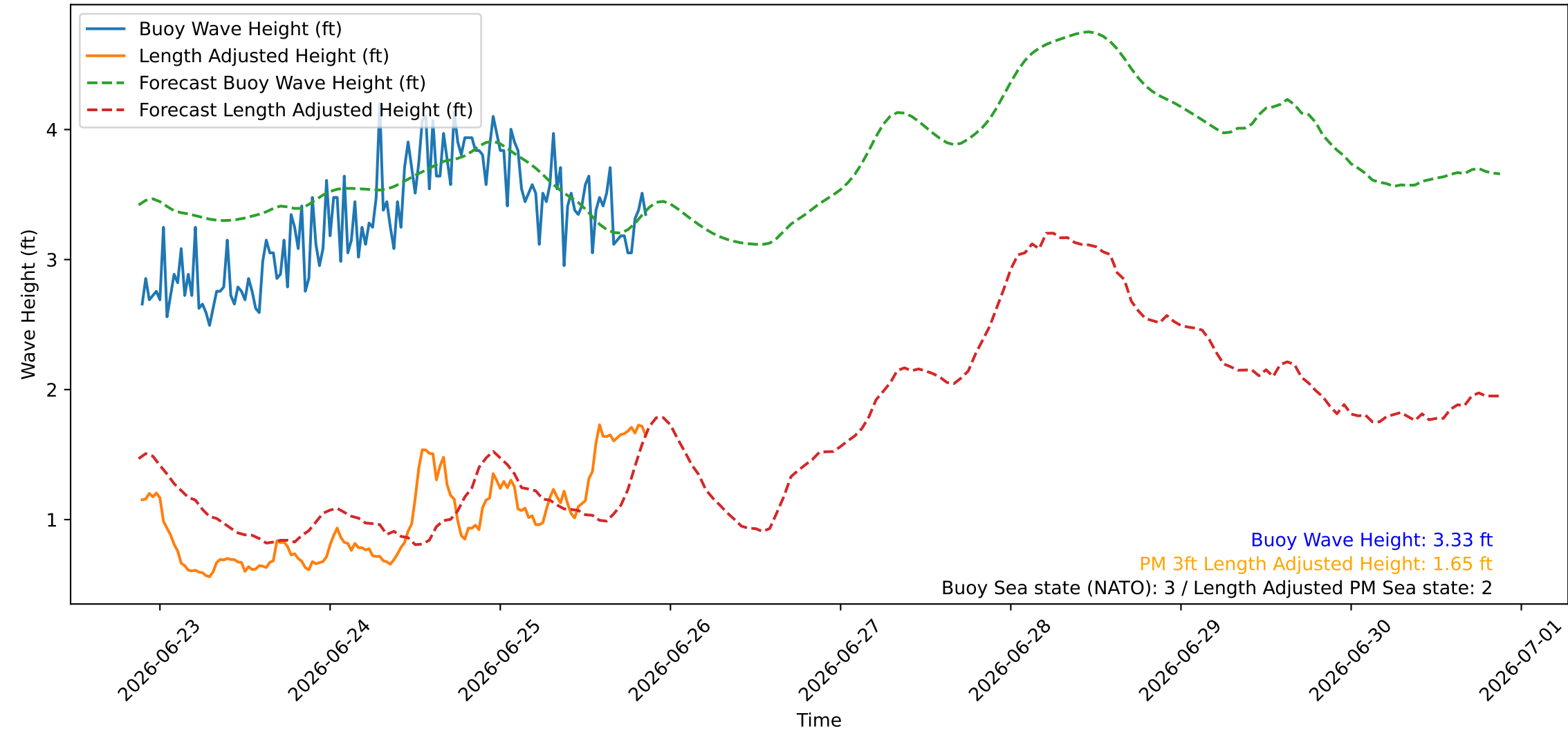
Wave Heights over Time for Green Beach at 2026-06-25 21:21:08
