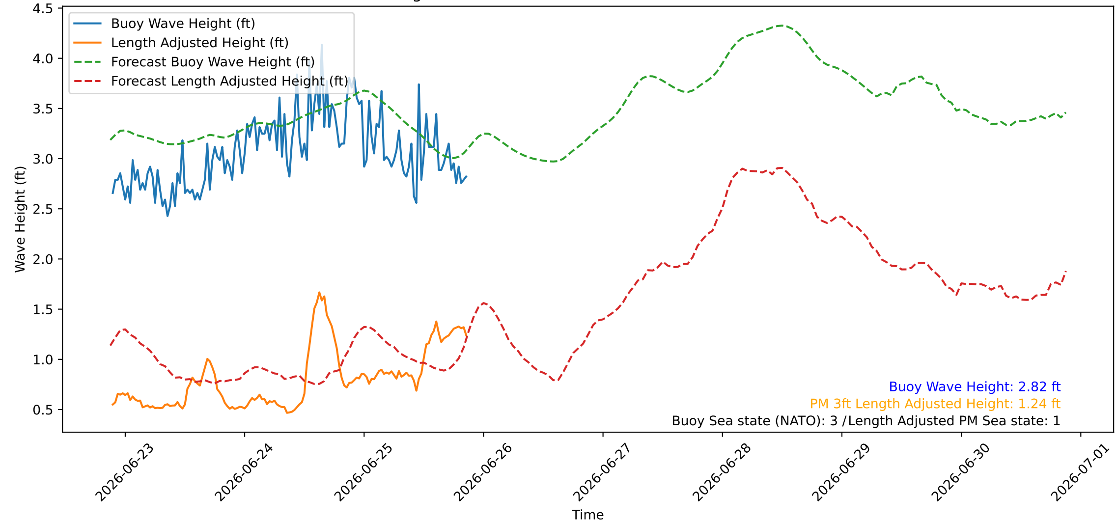
Wave Heights over Time for Red Beach at 2026-06-25 21:20:46
