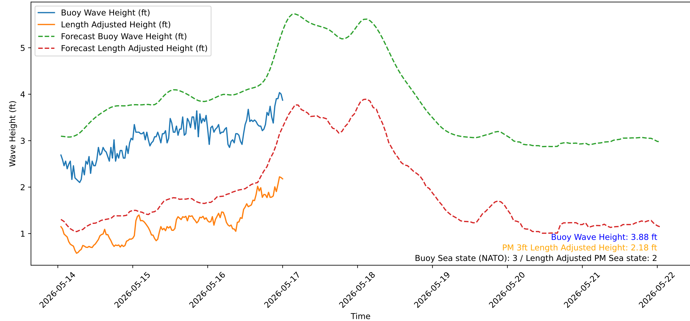
Wave Heights over Time for Green Beach at 2026-05-17 01:01:14
