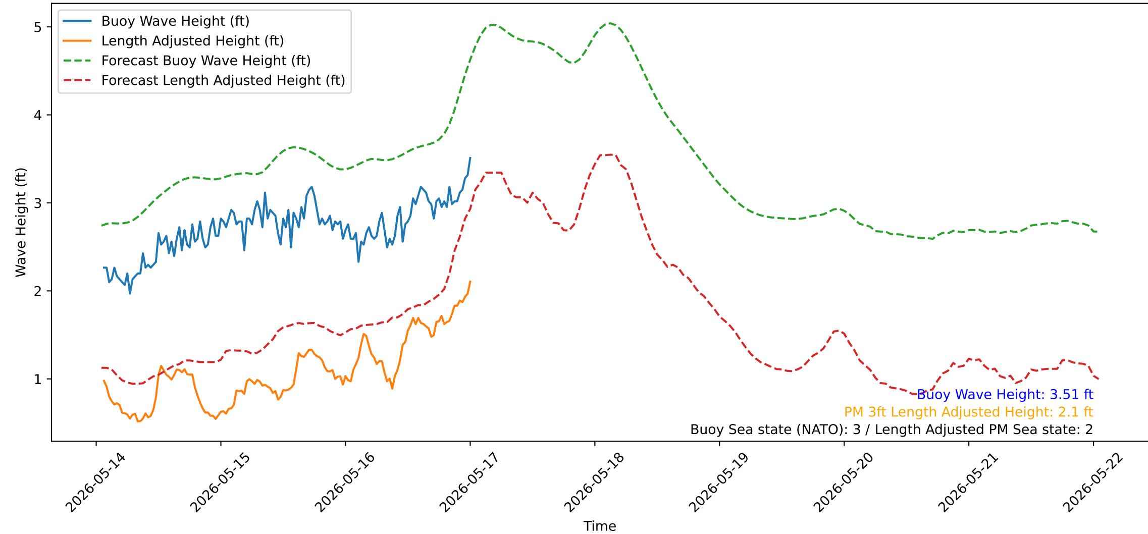
Wave Heights over Time for Red Beach at 2026-05-17 01:00:51
