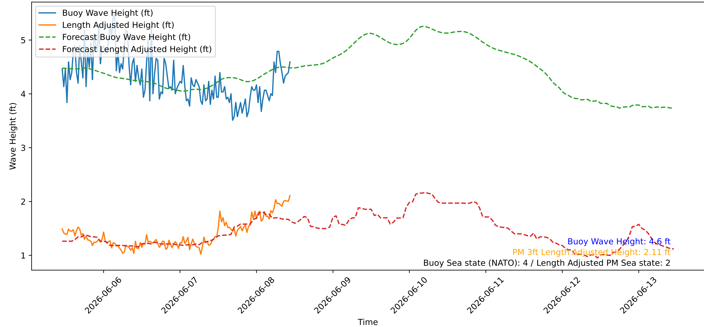
Wave Heights over Time for Oceanside Harbor at 2026-06-08 11:10:26
