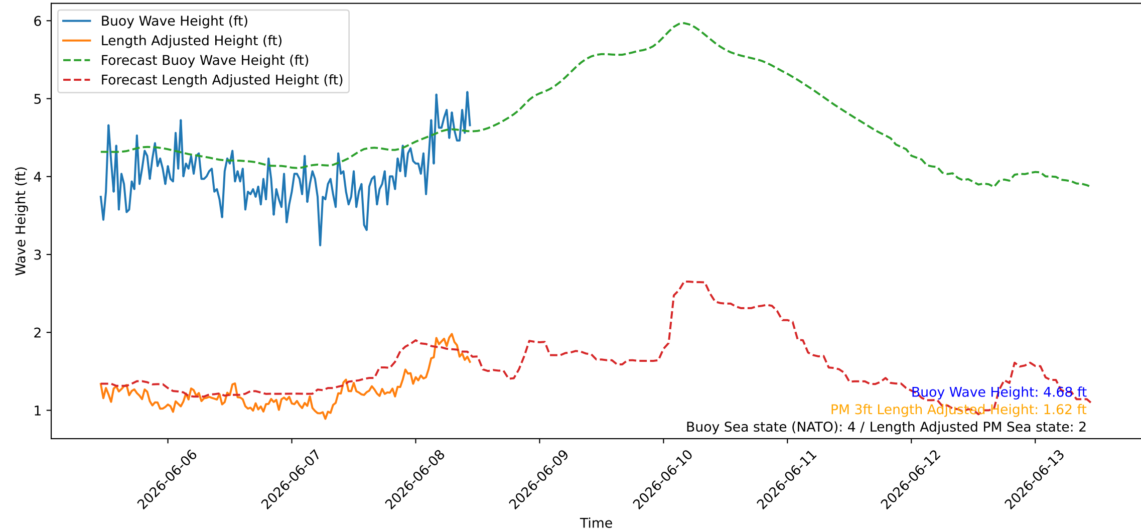
Wave Heights over Time for Green Beach at 2026-06-08 11:11:08
