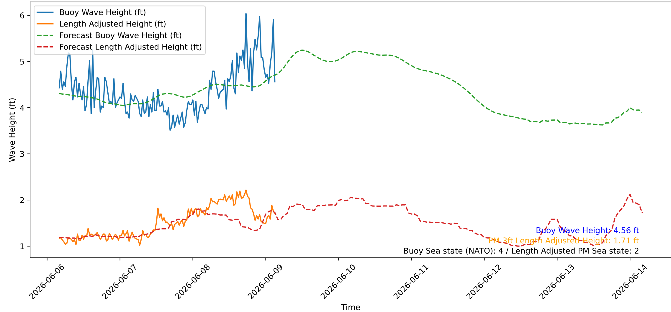
Wave Heights over Time for Oceanside Harbor at 2026-06-09 03:50:27
