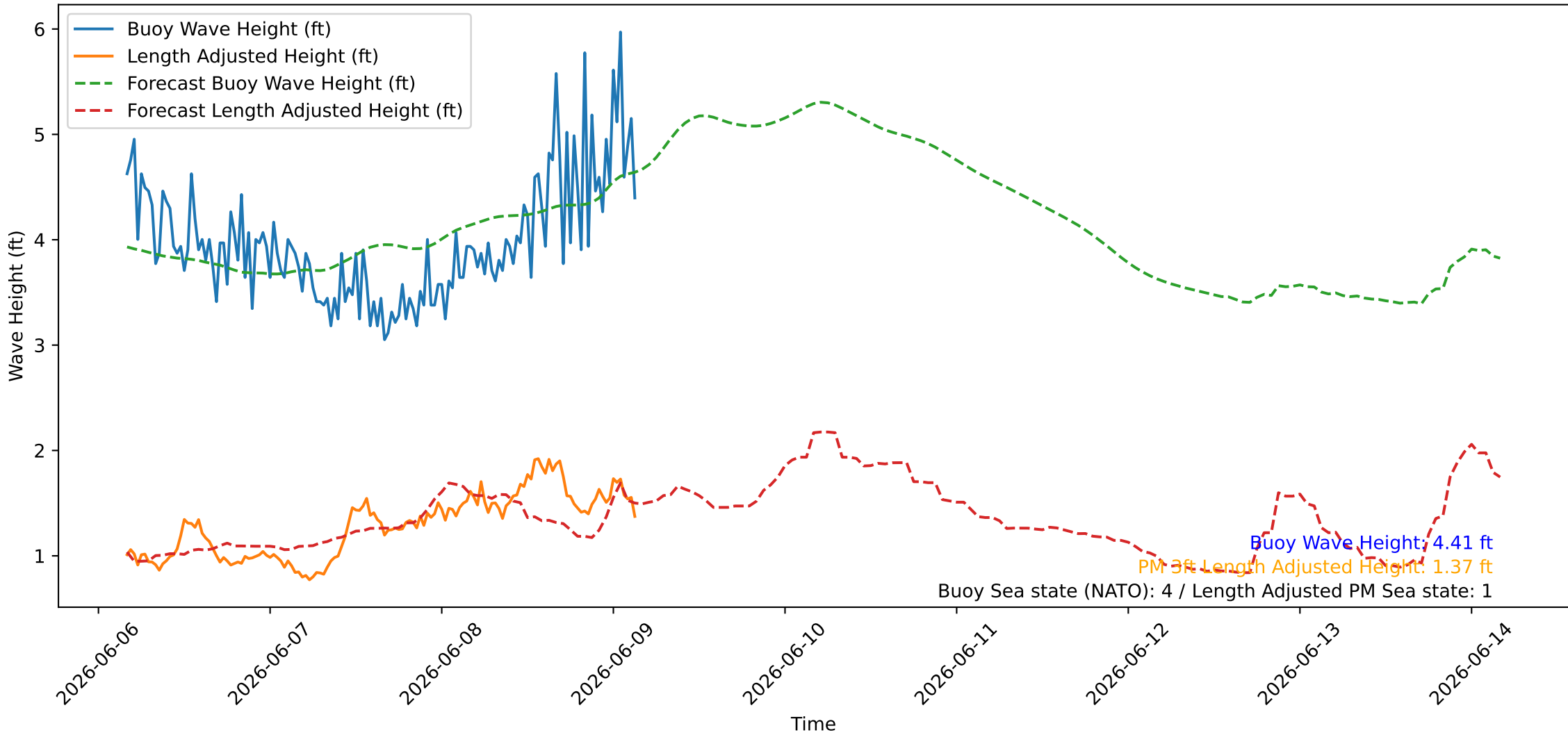
Wave Heights over Time for Red Beach at 2026-06-09 03:50:47
