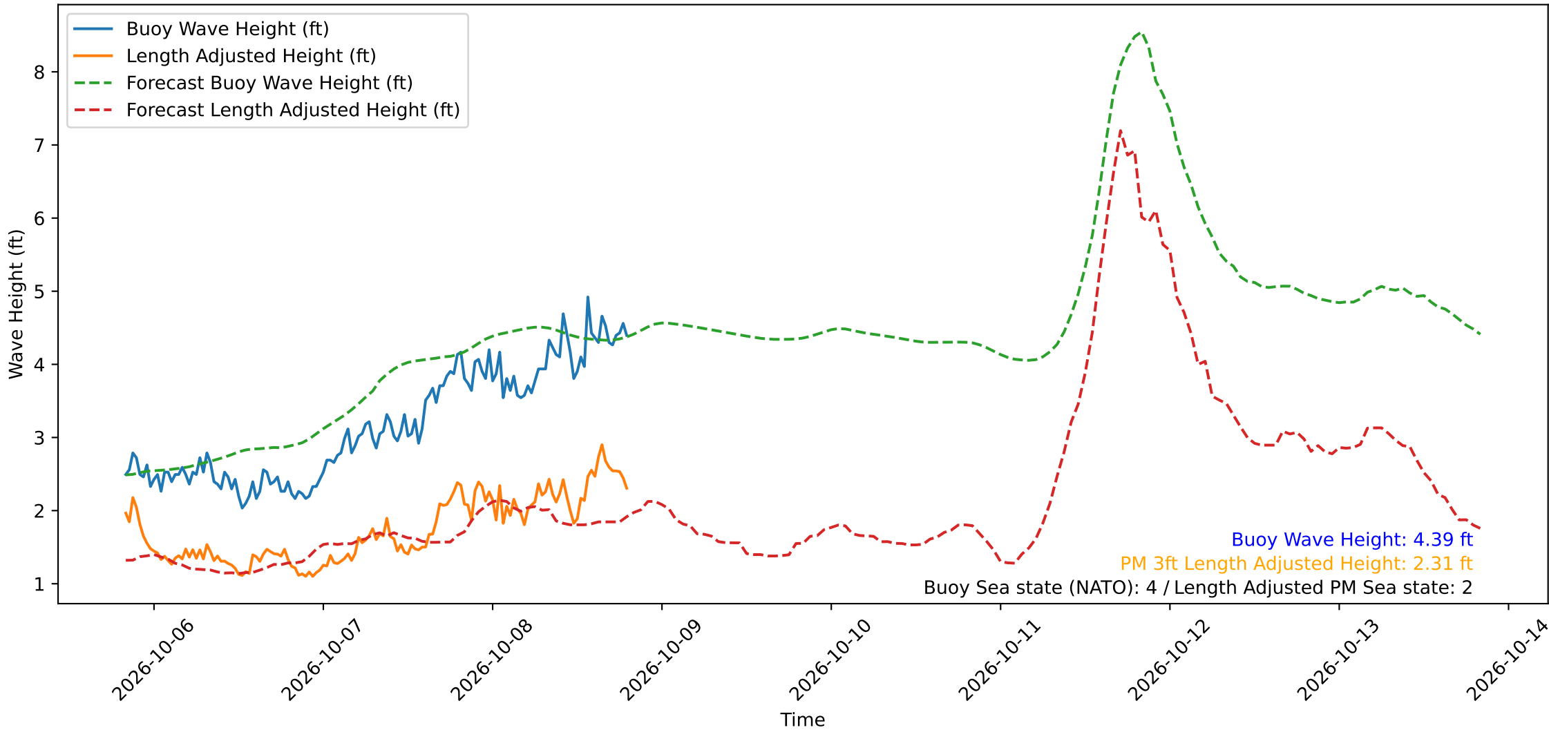
Wave Heights over Time for Oceanside Harbor at 2026-10-08 20:00:29
