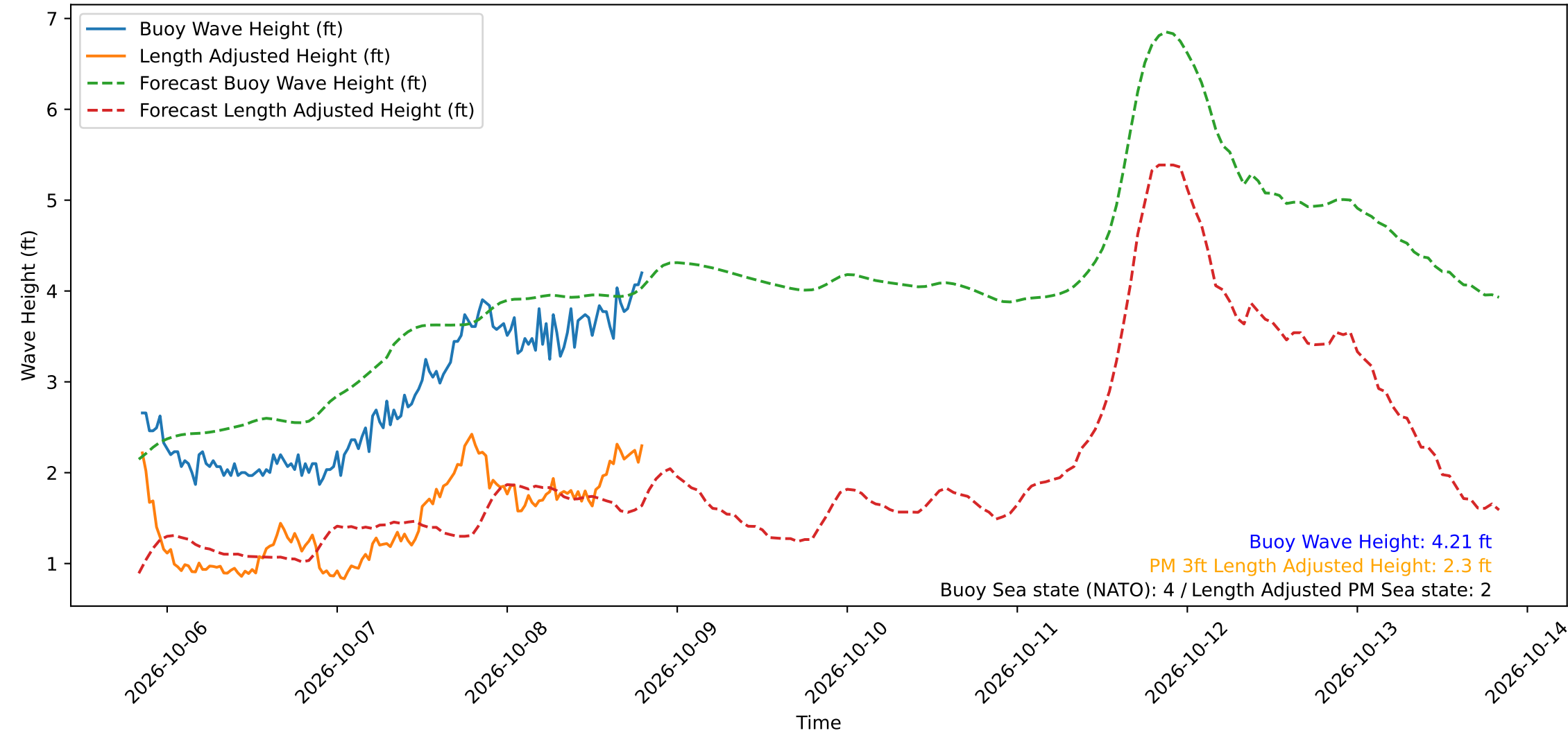
Wave Heights over Time for Red Beach at 2026-10-08 20:00:50
