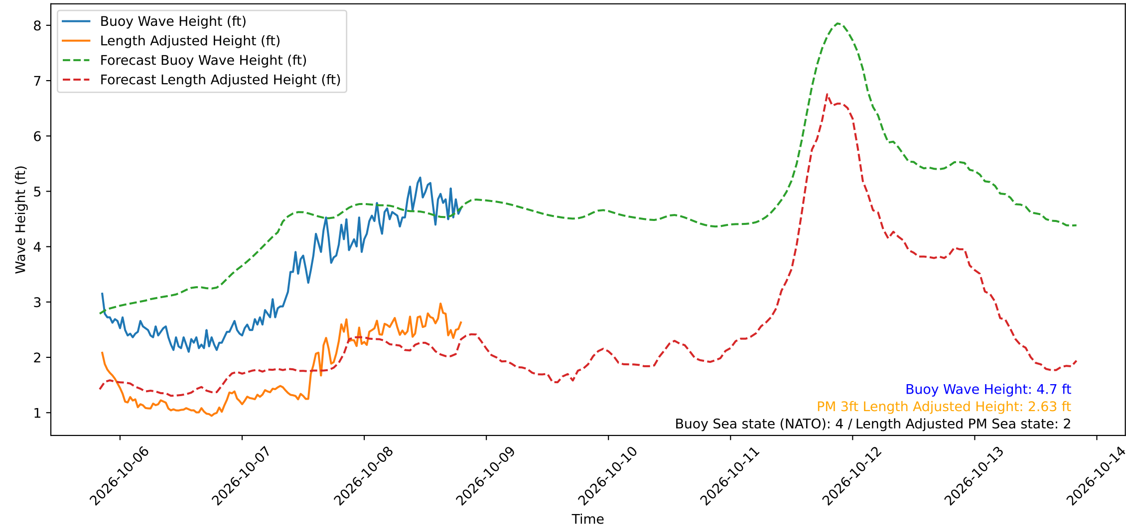
Wave Heights over Time for Green Beach at 2026-10-08 20:01:12
