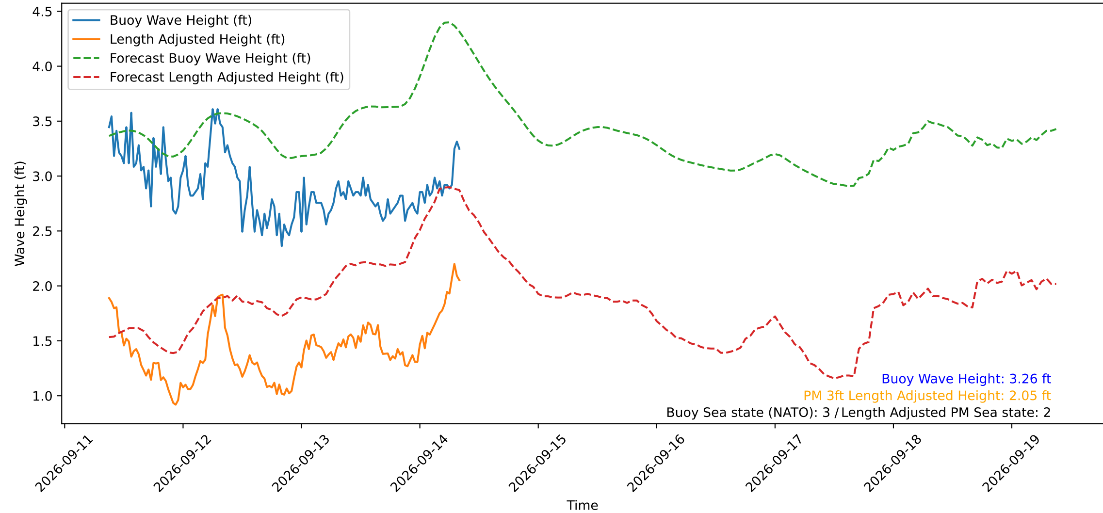
Wave Heights over Time for Green Beach at 2026-09-14 08:51:14
