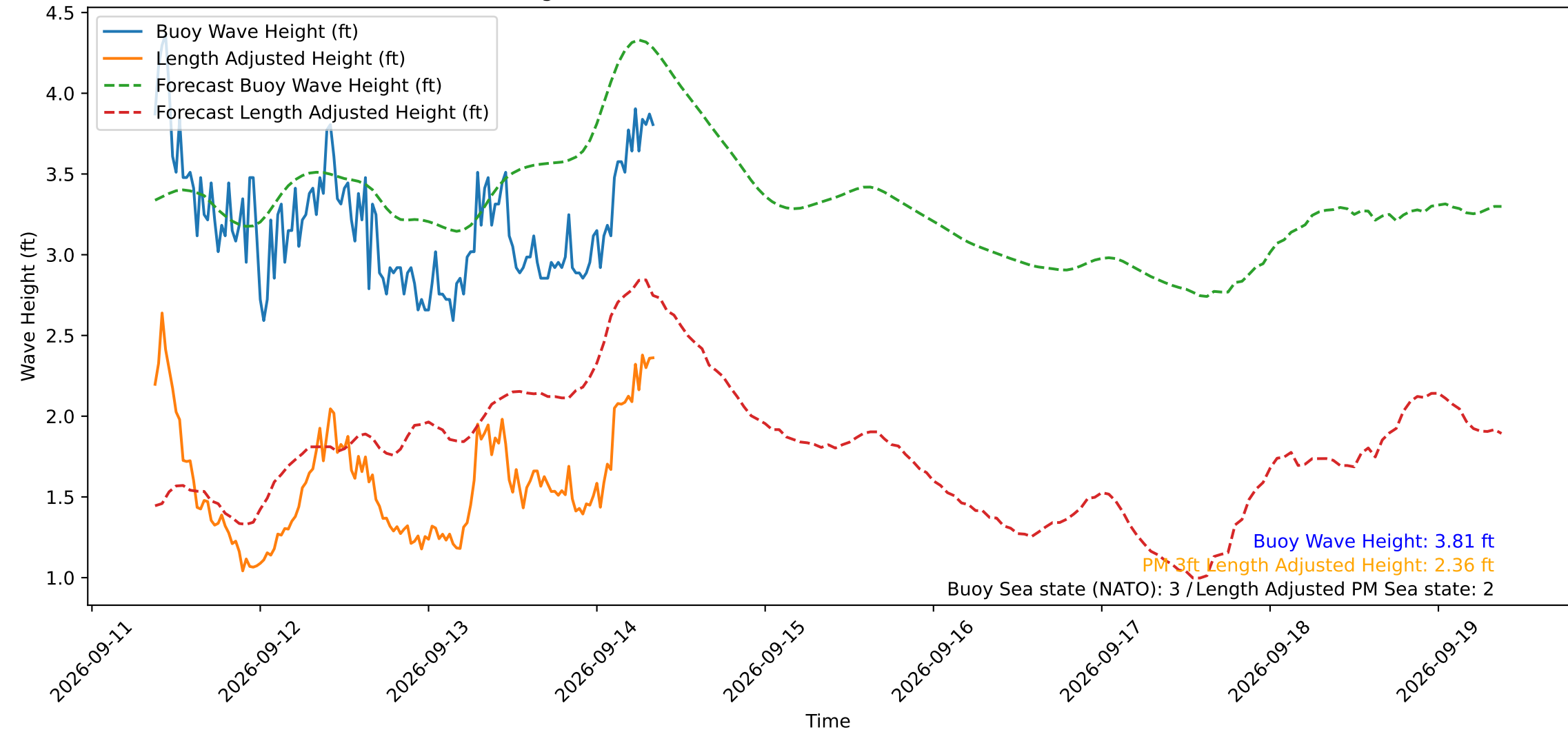
Wave Heights over Time for Oceanside Harbor at 2026-09-14 08:50:29
