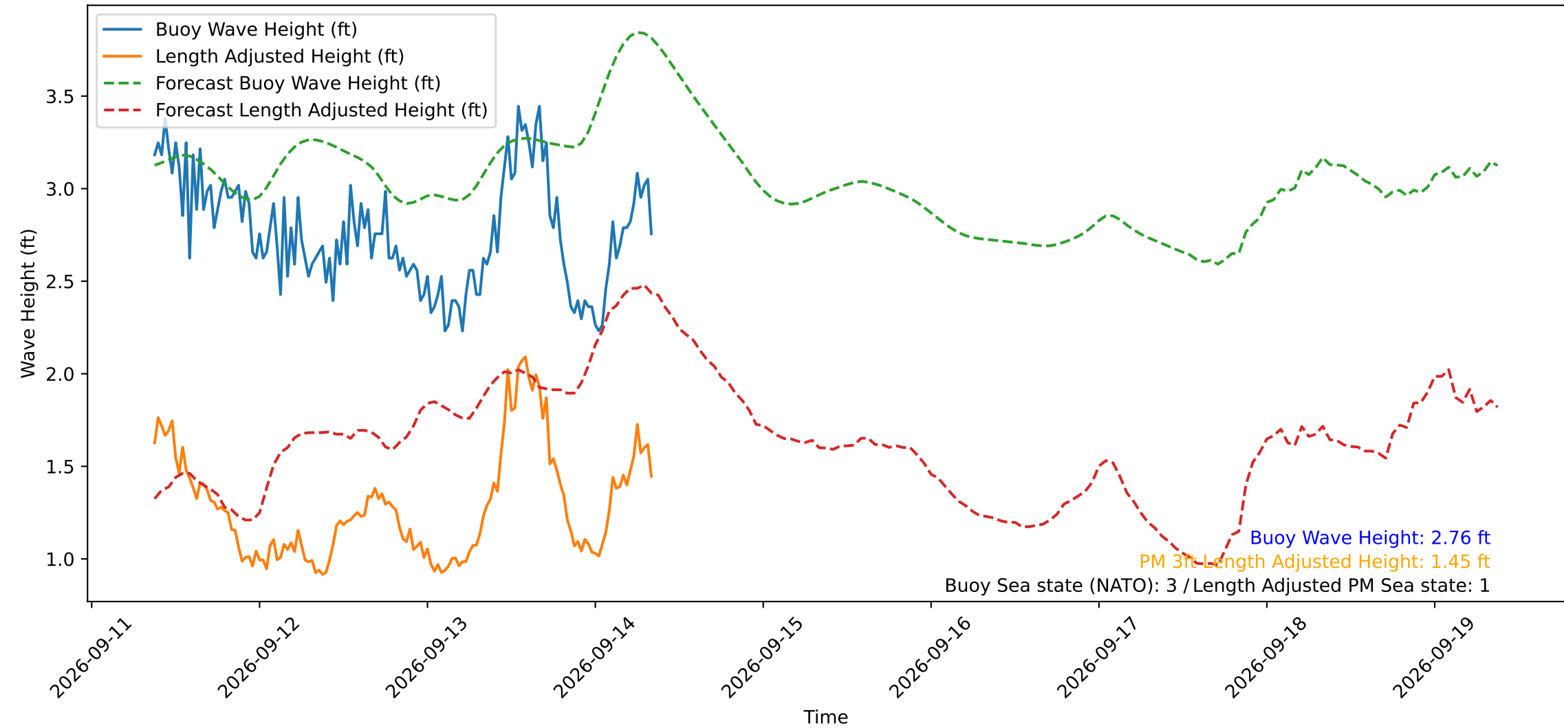
Wave Heights over Time for Red Beach at 2026-09-14 08:50:50
