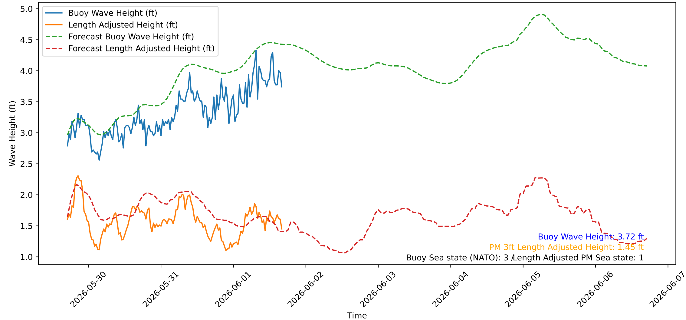
Wave Heights over Time for Green Beach at 2026-06-01 17:01:08
