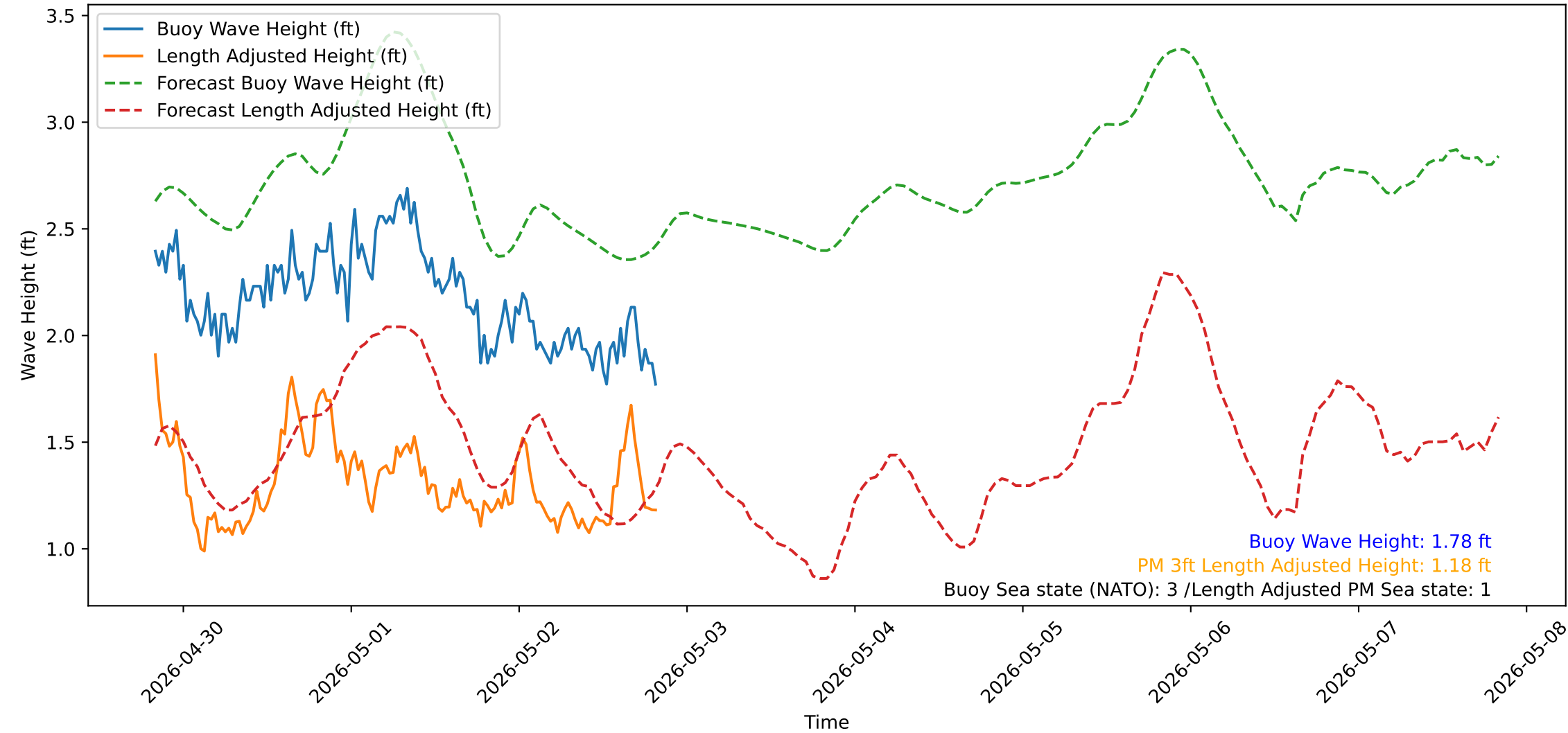
Wave Heights over Time for Oceanside Harbor at 2026-05-02 20:10:31
