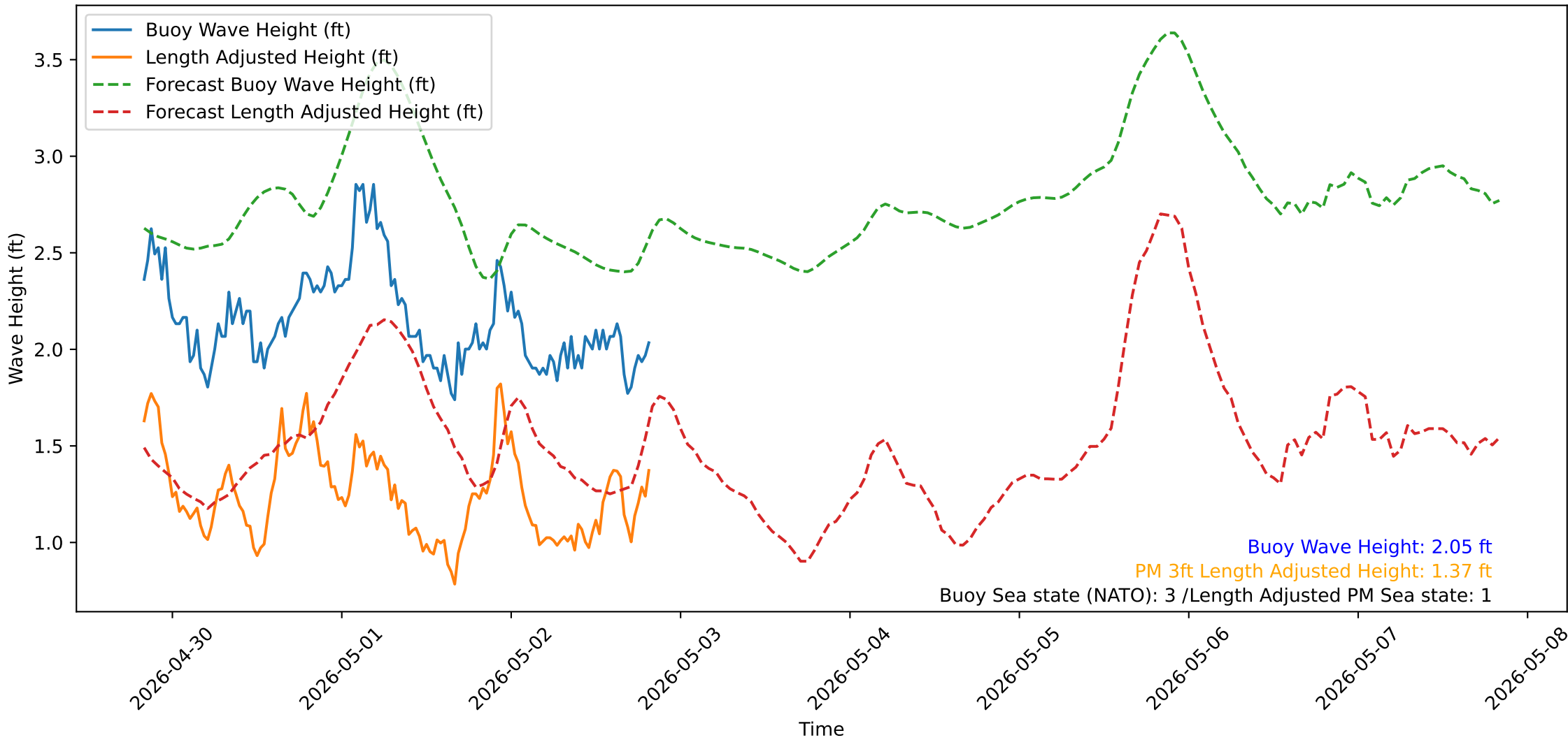
Wave Heights over Time for Green Beach at 2026-05-02 20:11:12
