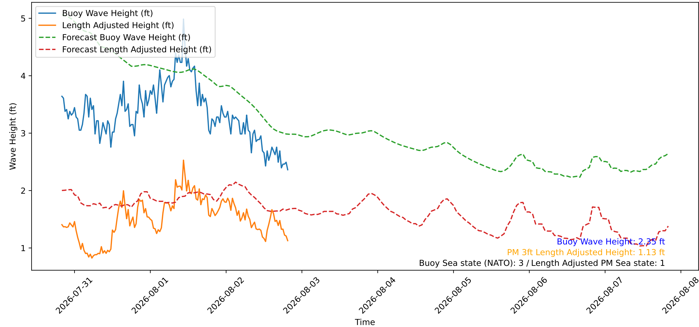
Wave Heights over Time for Green Beach at 2026-08-02 20:11:08
