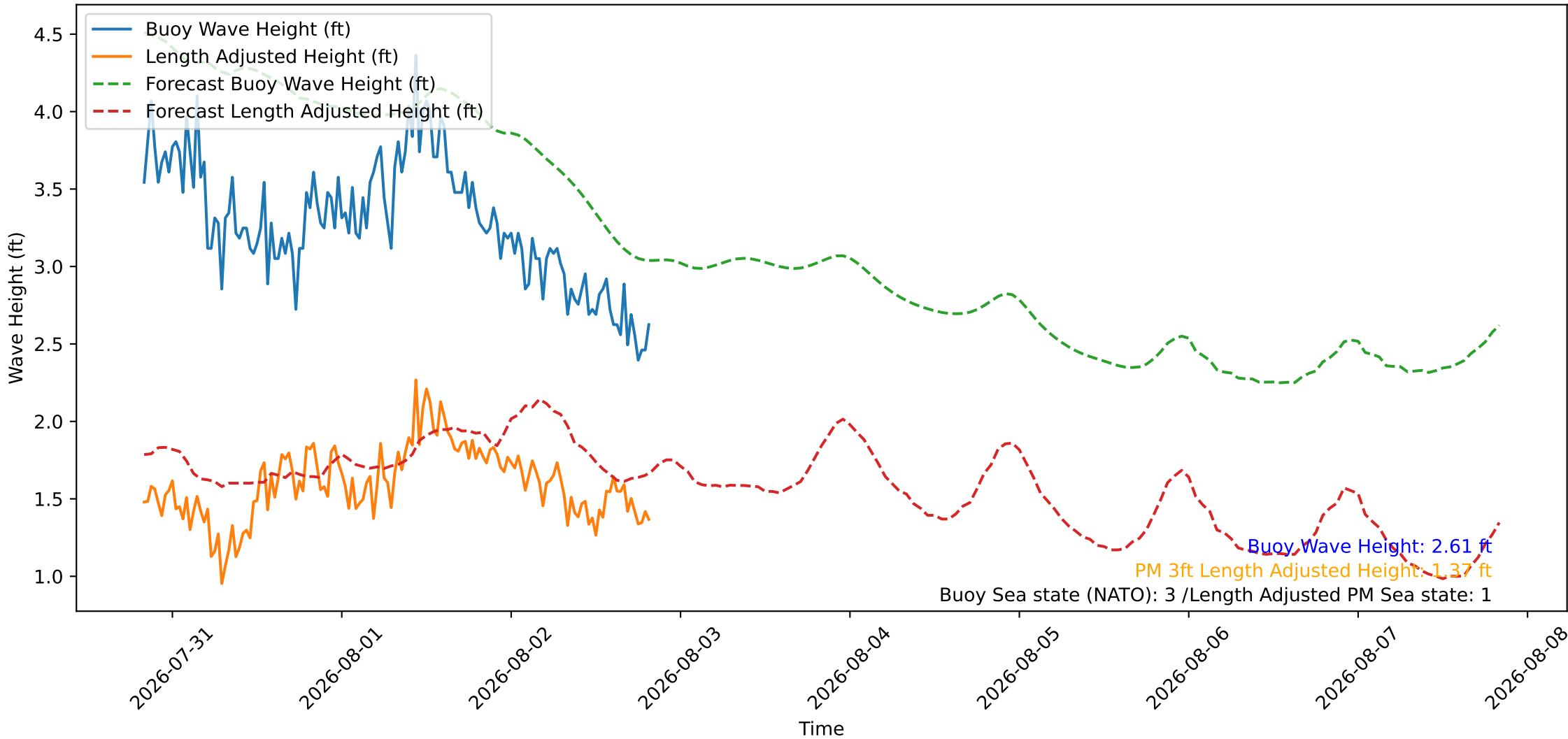
Wave Heights over Time for Oceanside Harbor at 2026-08-02 20:10:26
