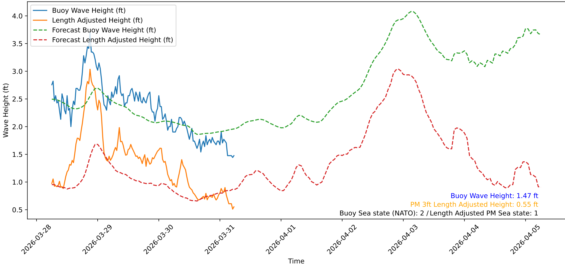
Wave Heights over Time for Green Beach at 2026-03-31 06:11:11
