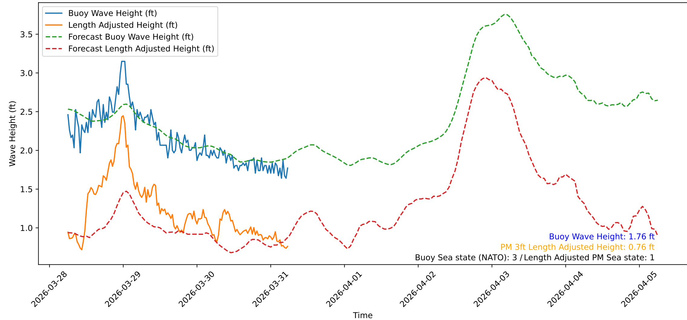
Wave Heights over Time for Oceanside Harbor at 2026-03-31 06:10:32
