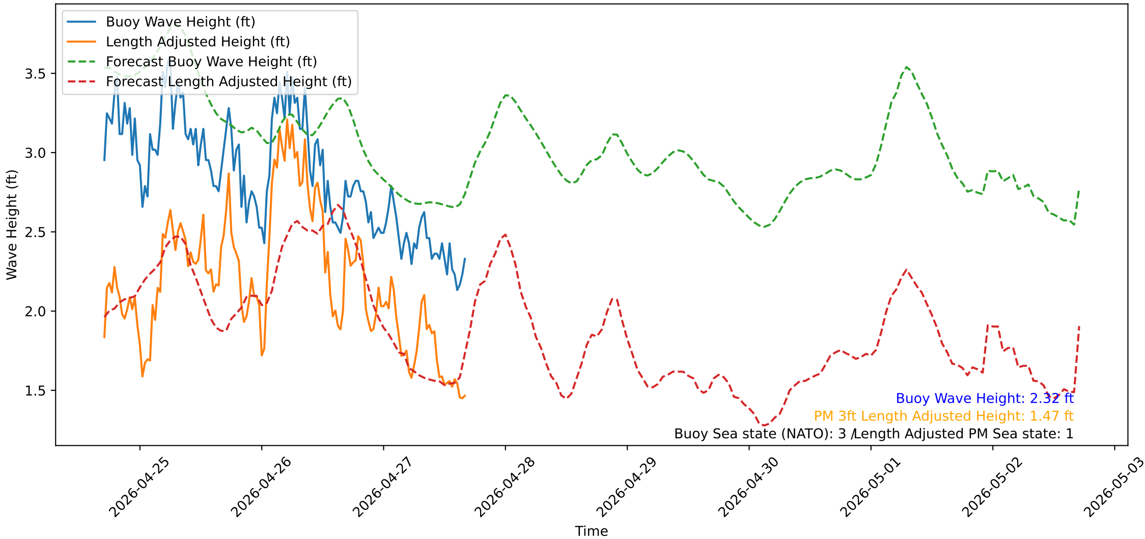
Wave Heights over Time for Green Beach at 2026-04-27 17:01:12
