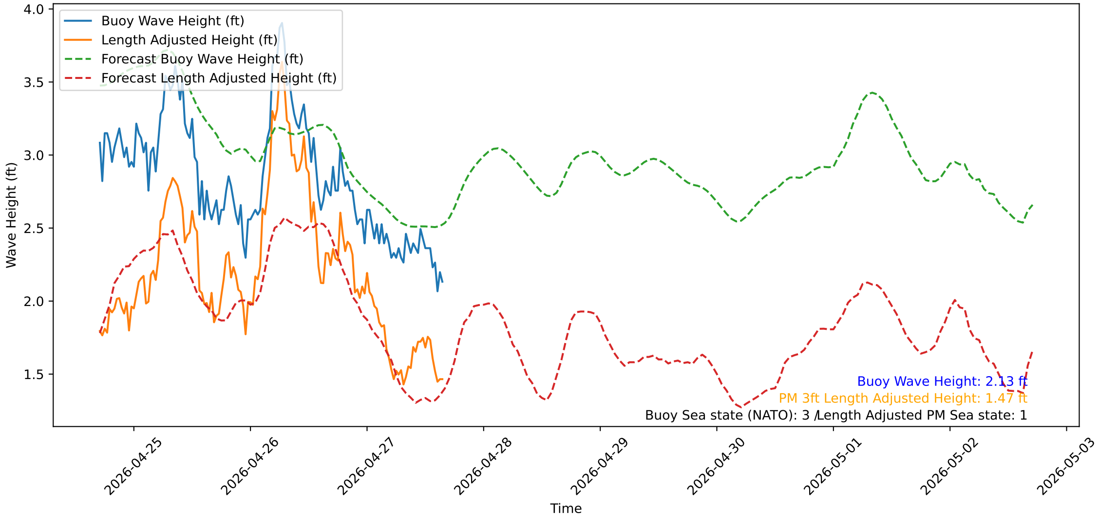
Wave Heights over Time for Oceanside Harbor at 2026-04-27 17:00:31
