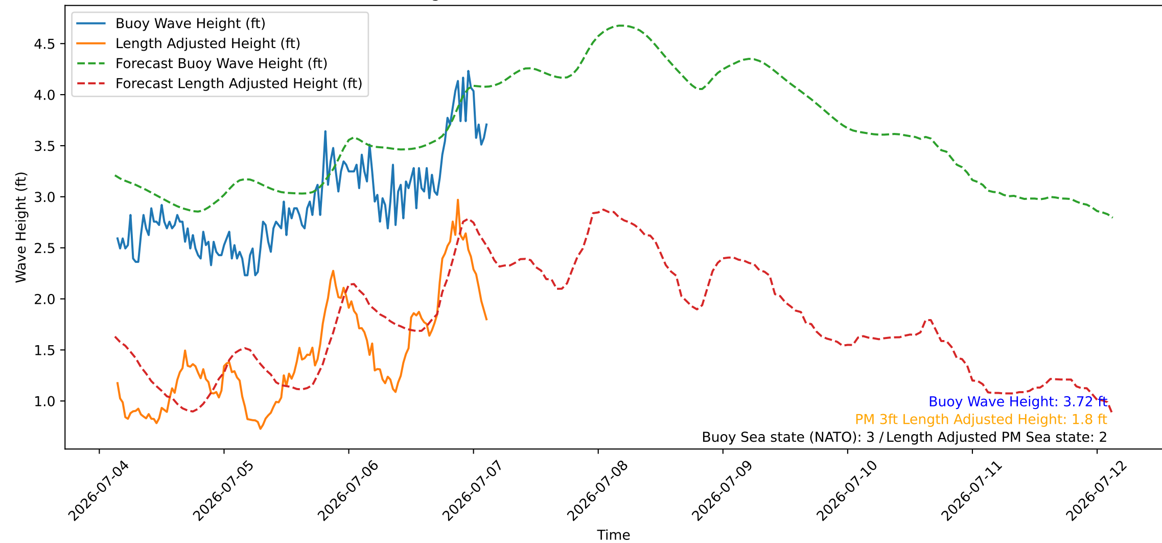
Wave Heights over Time for Red Beach at 2026-07-07 03:10:46
