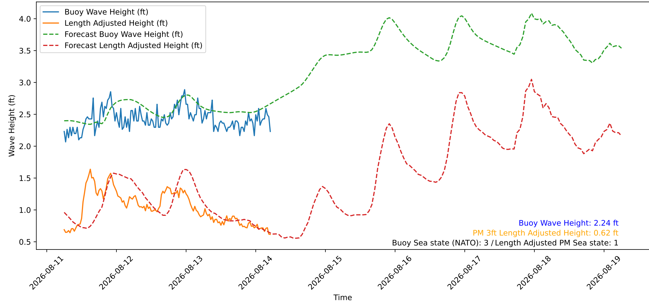
Wave Heights over Time for Red Beach at 2026-08-14 05:40:46
