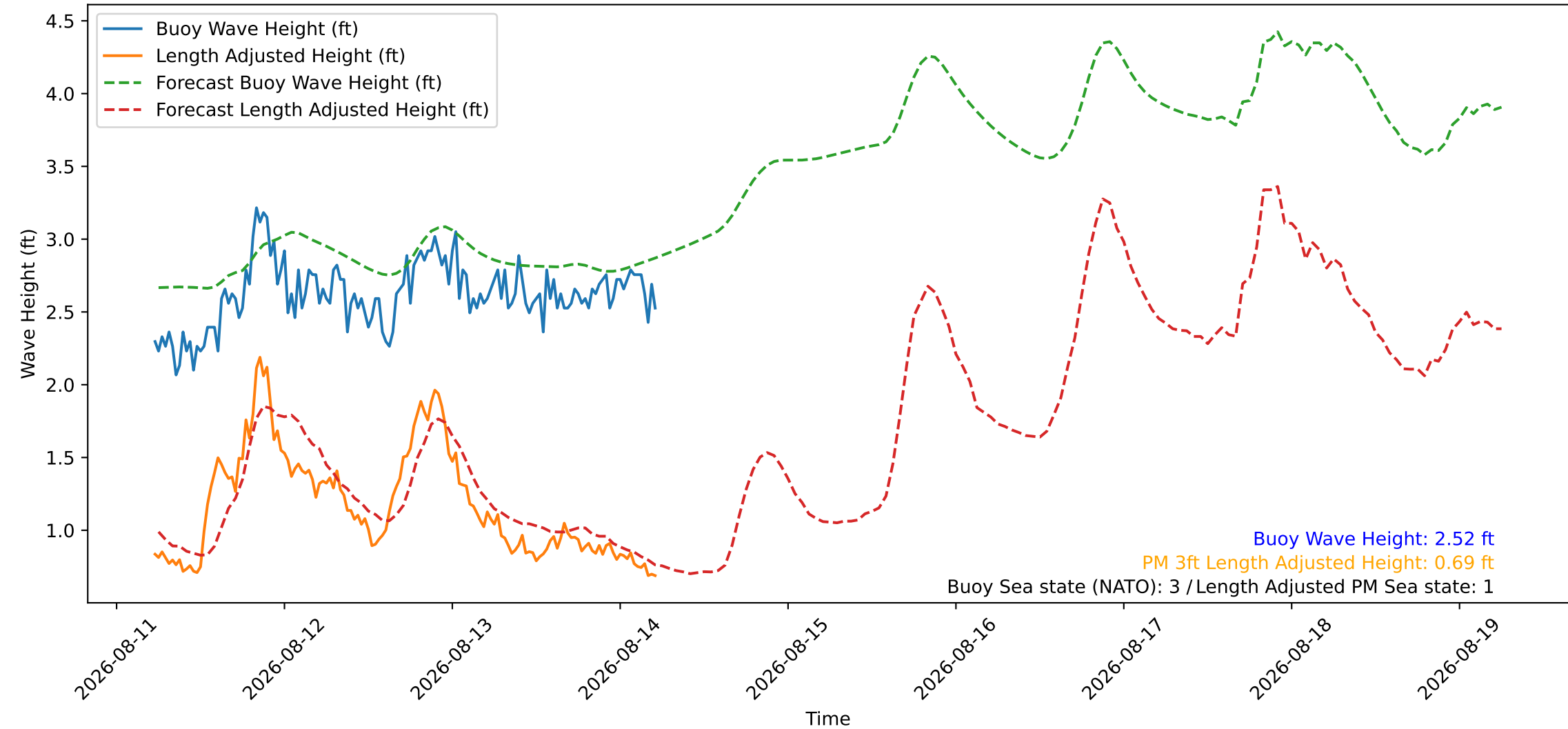
Wave Heights over Time for Green Beach at 2026-08-14 05:41:09
