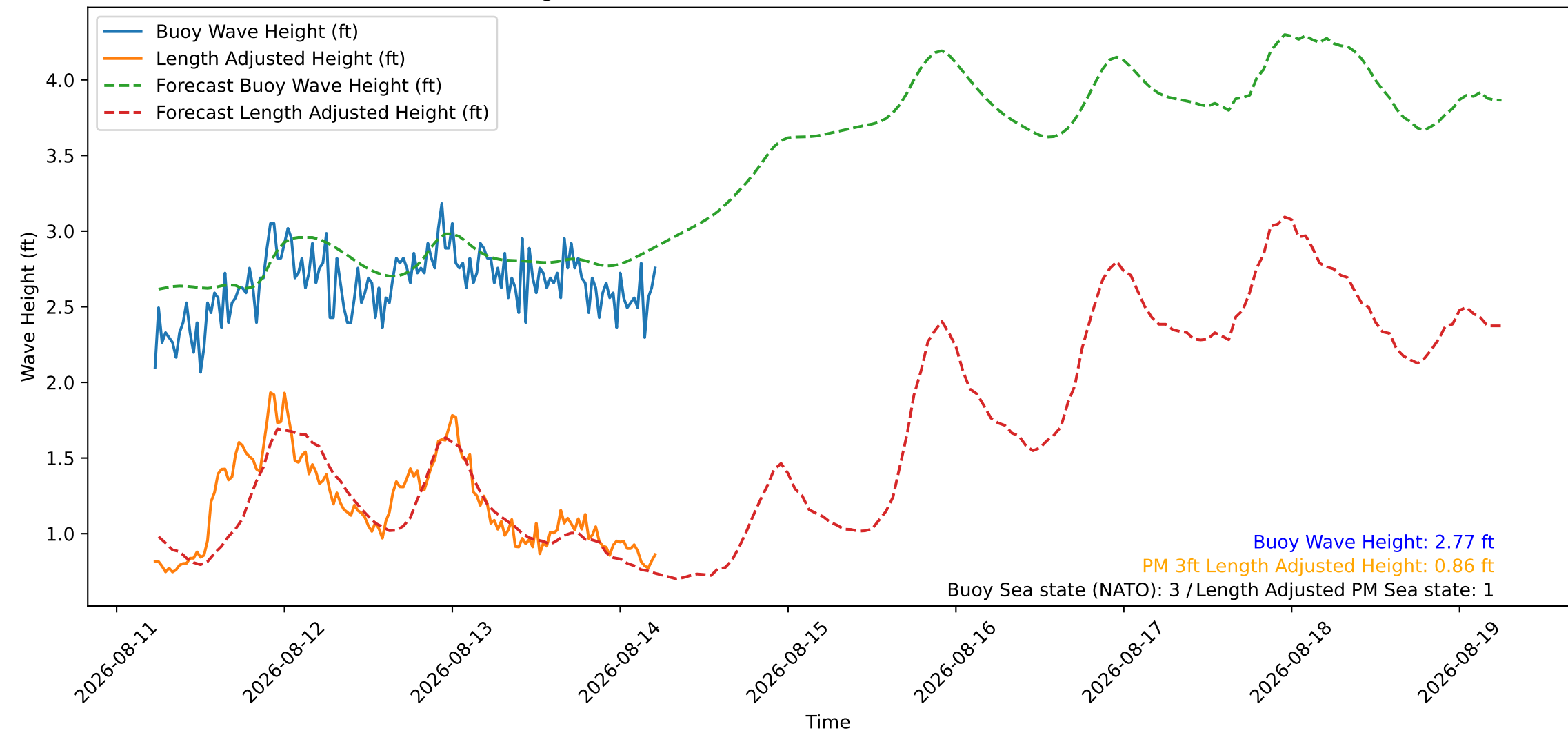
Wave Heights over Time for Oceanside Harbor at 2026-08-14 05:40:26
