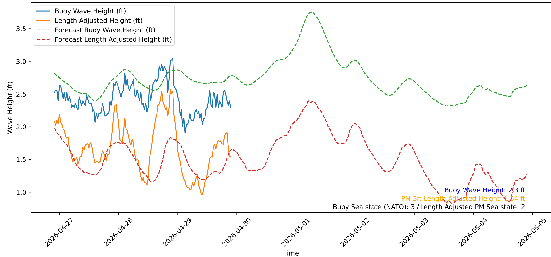
Wave Heights over Time for Oceanside Harbor at 2026-04-29 22:10:31
