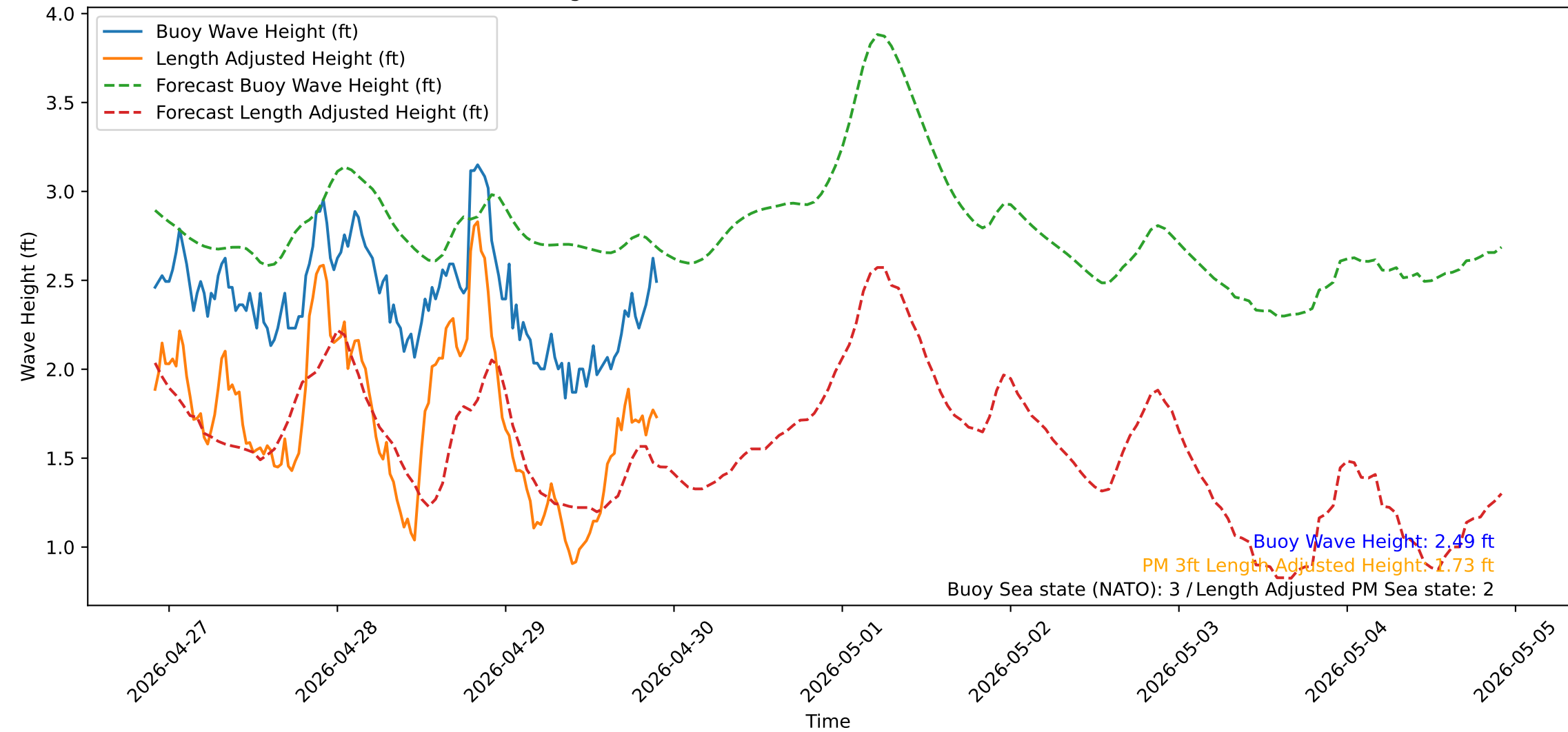
Wave Heights over Time for Green Beach at 2026-04-29 22:11:13
