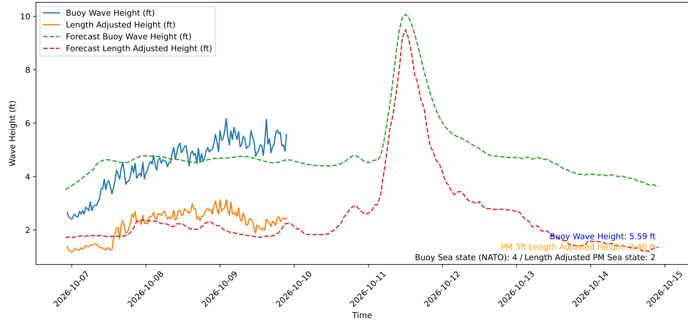
Wave Heights over Time for Green Beach at 2026-10-09 22:11:12
