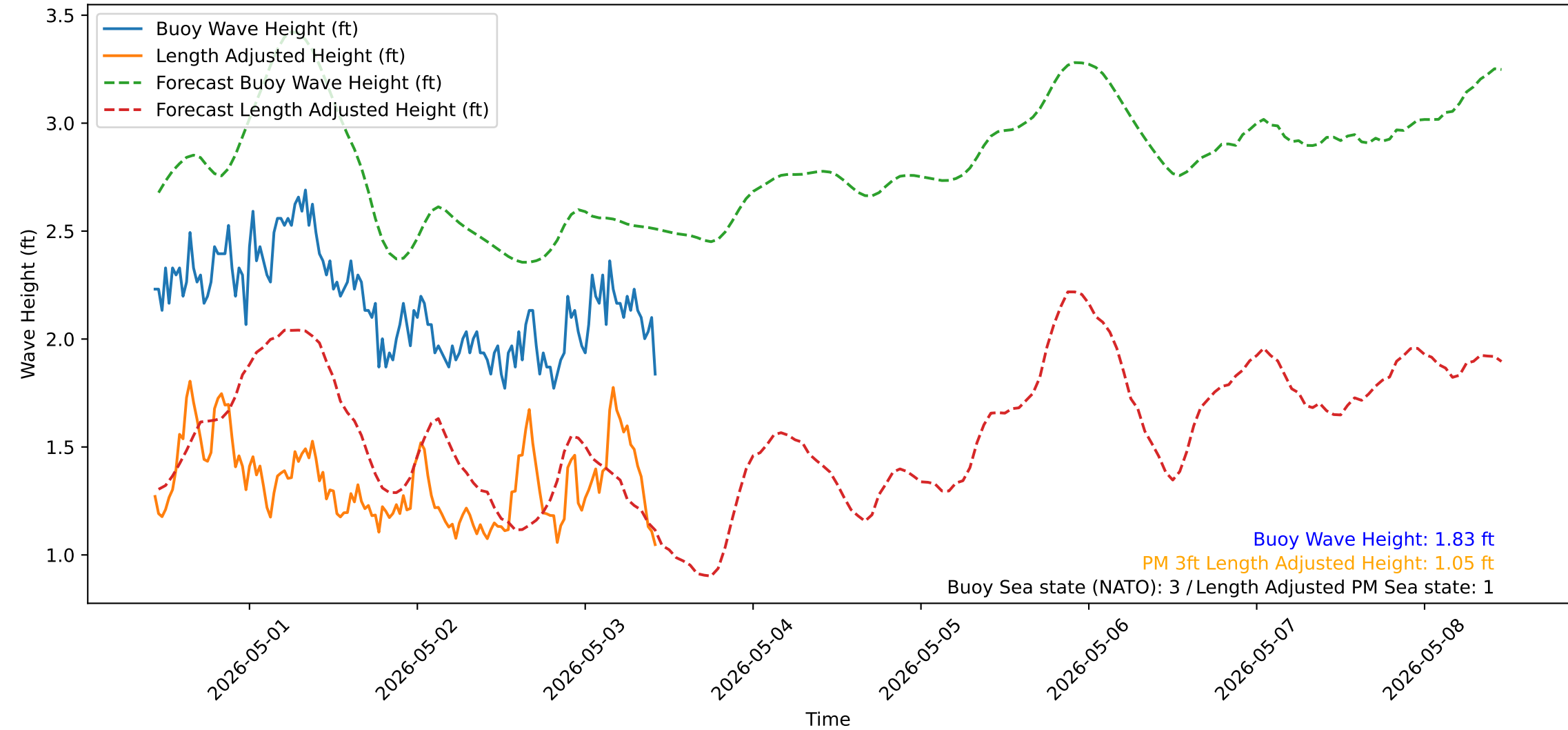
Wave Heights over Time for Oceanside Harbor at 2026-05-03 10:30:31
