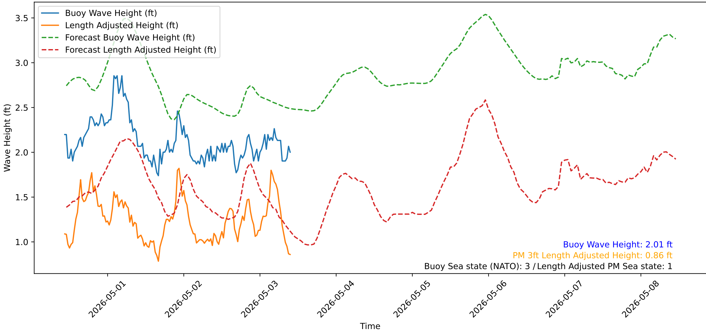
Wave Heights over Time for Green Beach at 2026-05-03 10:31:12
