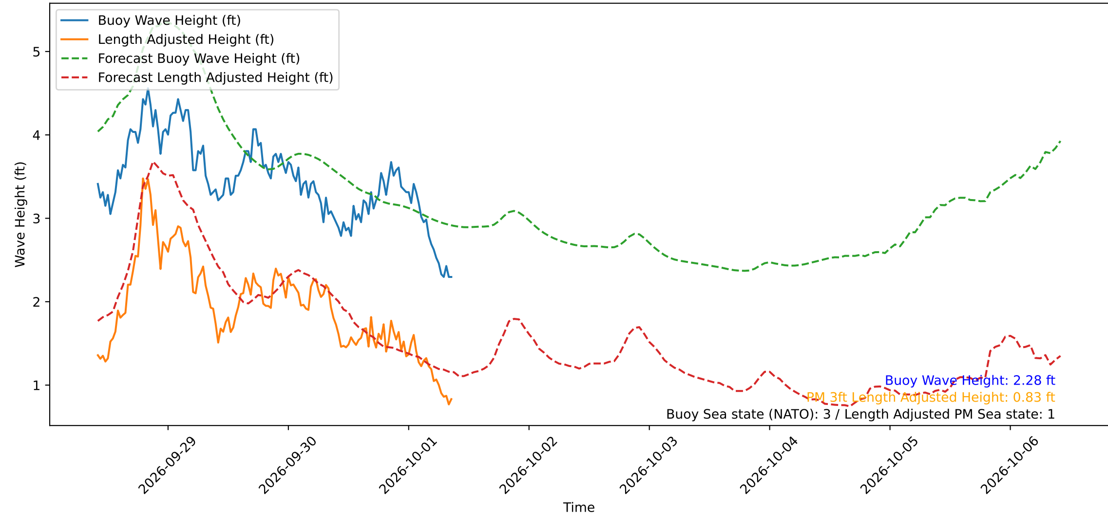
Wave Heights over Time for Green Beach at 2026-10-01 09:31:13
