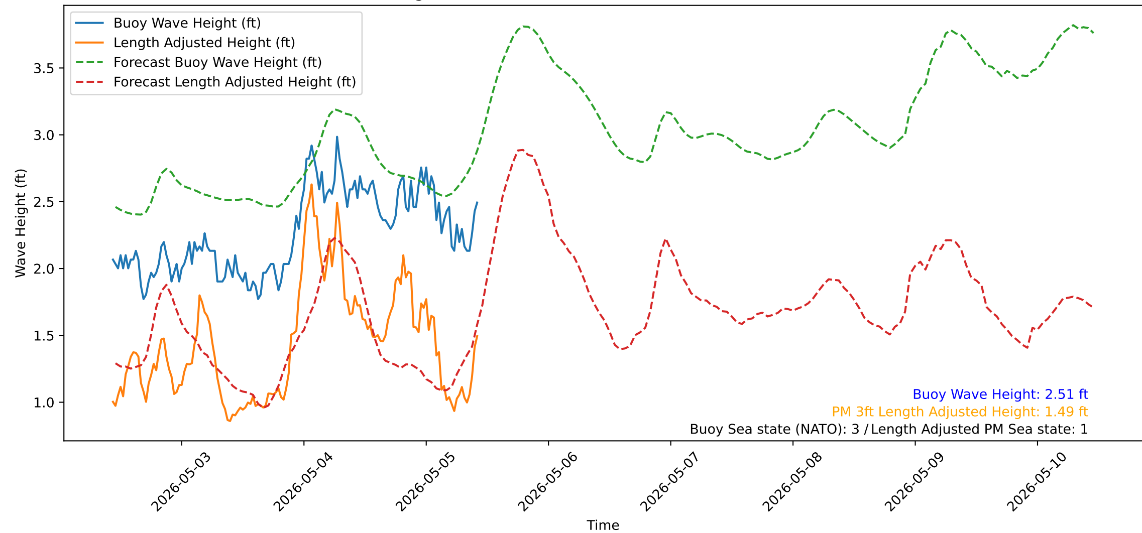
Wave Heights over Time for Green Beach at 2026-05-05 10:41:13
