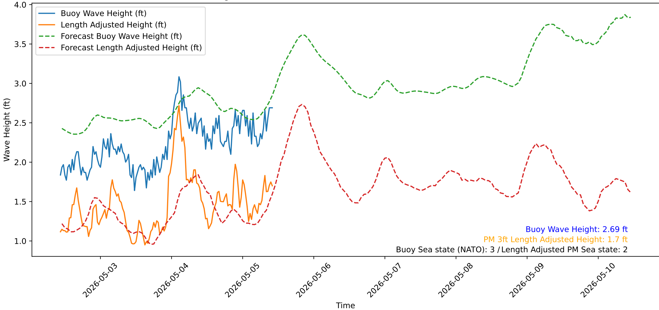
Wave Heights over Time for Oceanside Harbor at 2026-05-05 10:40:31
