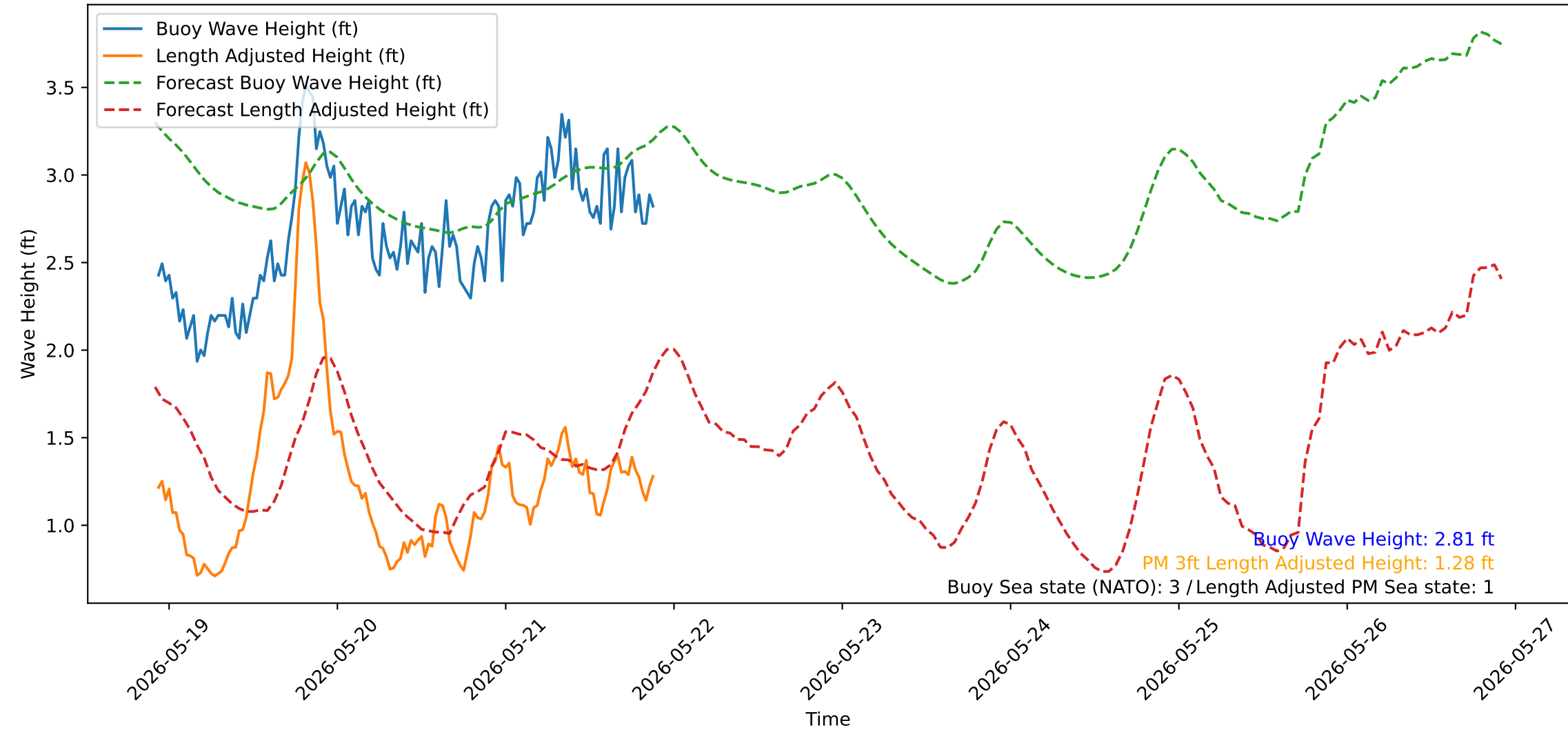
Wave Heights over Time for Red Beach at 2026-05-21 22:20:52
