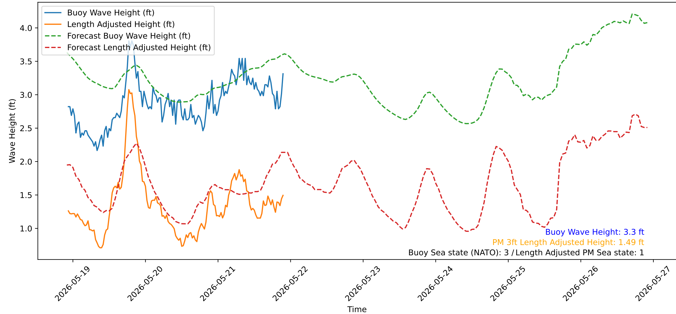
Wave Heights over Time for Green Beach at 2026-05-21 22:21:14
