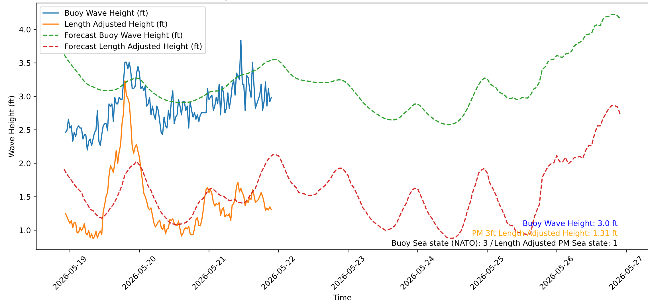
Wave Heights over Time for Oceanside Harbor at 2026-05-21 22:20:31
