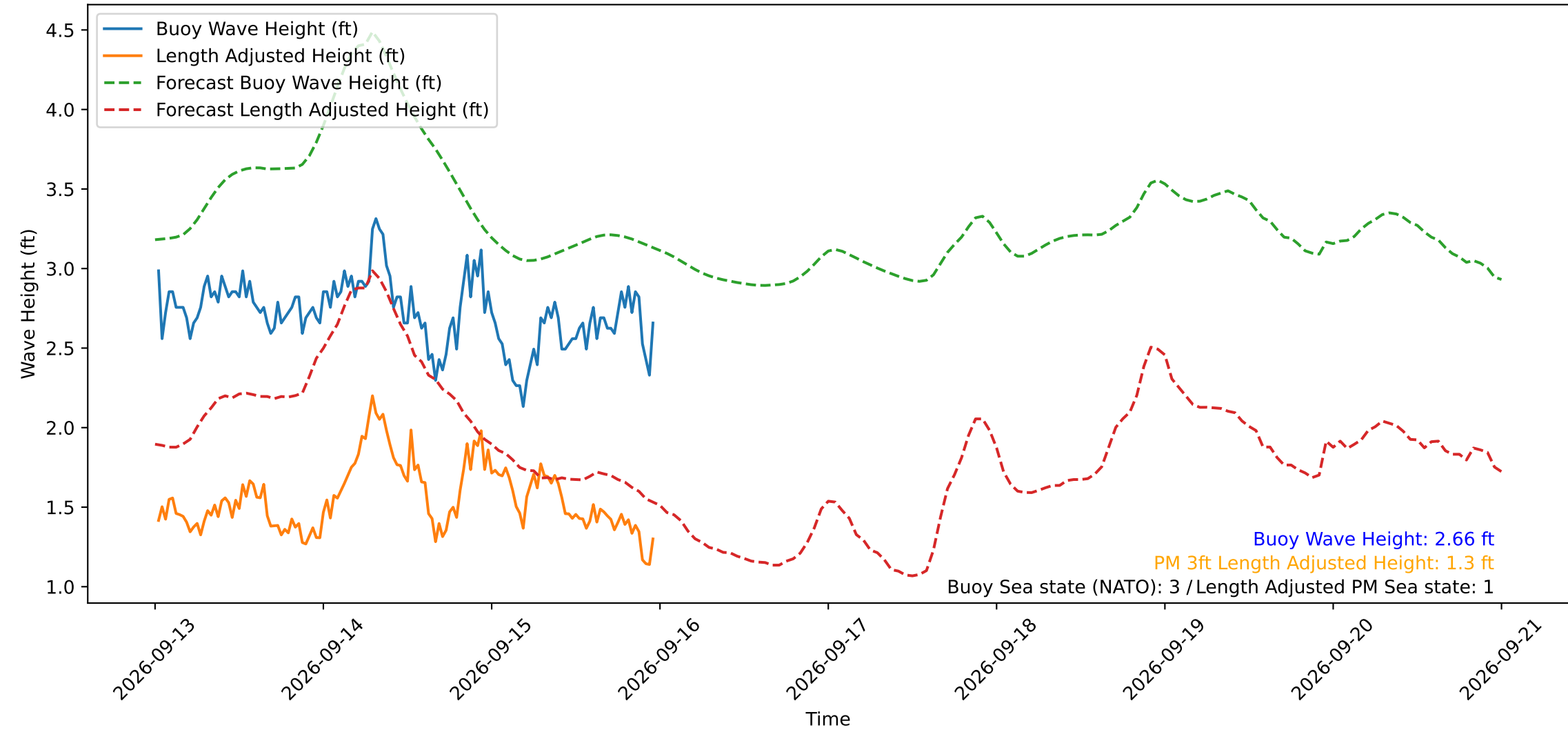
Wave Heights over Time for Green Beach at 2026-09-16 00:21:14
