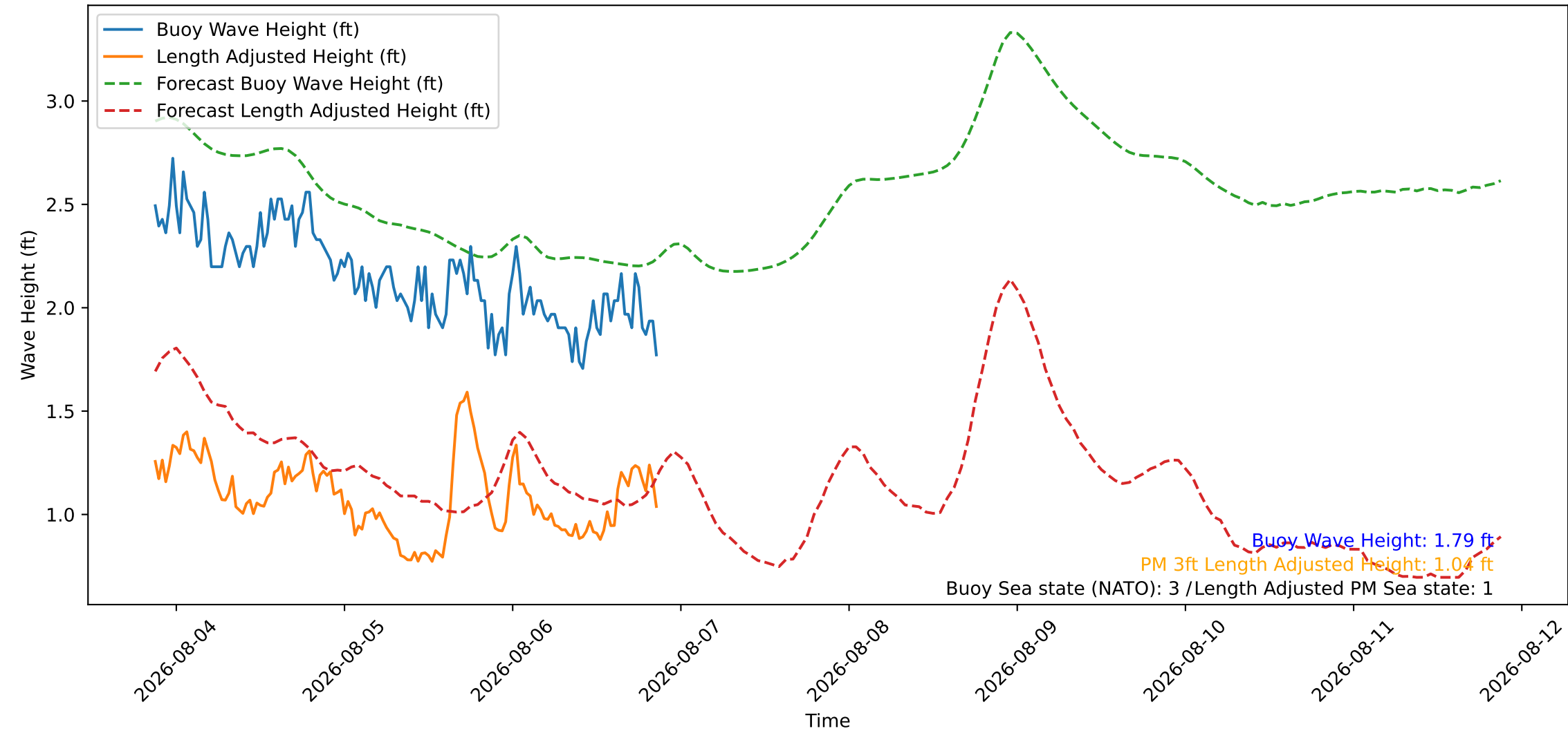
Wave Heights over Time for Oceanside Harbor at 2026-08-06 21:10:25
