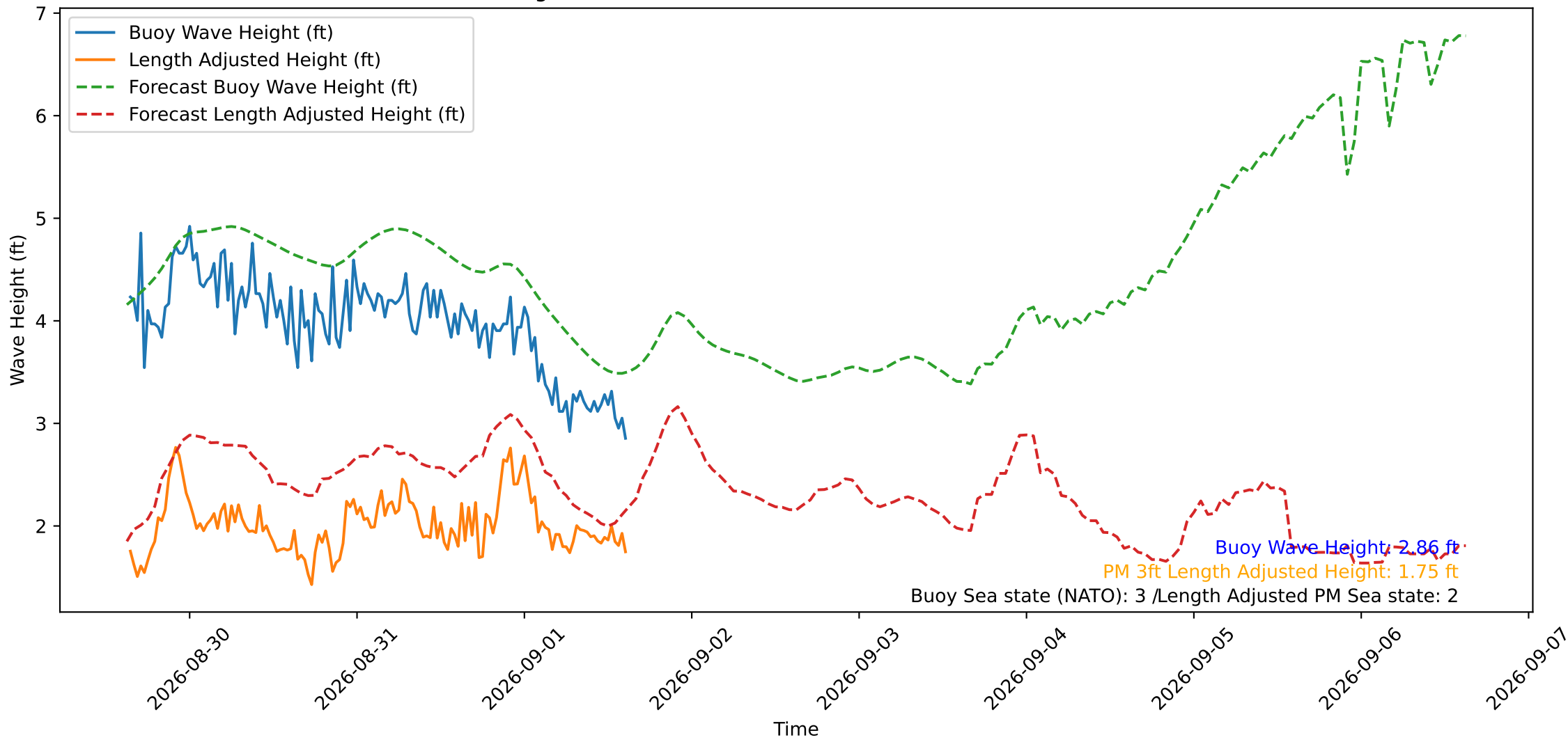
Wave Heights over Time for Green Beach at 2026-09-01 15:11:12
