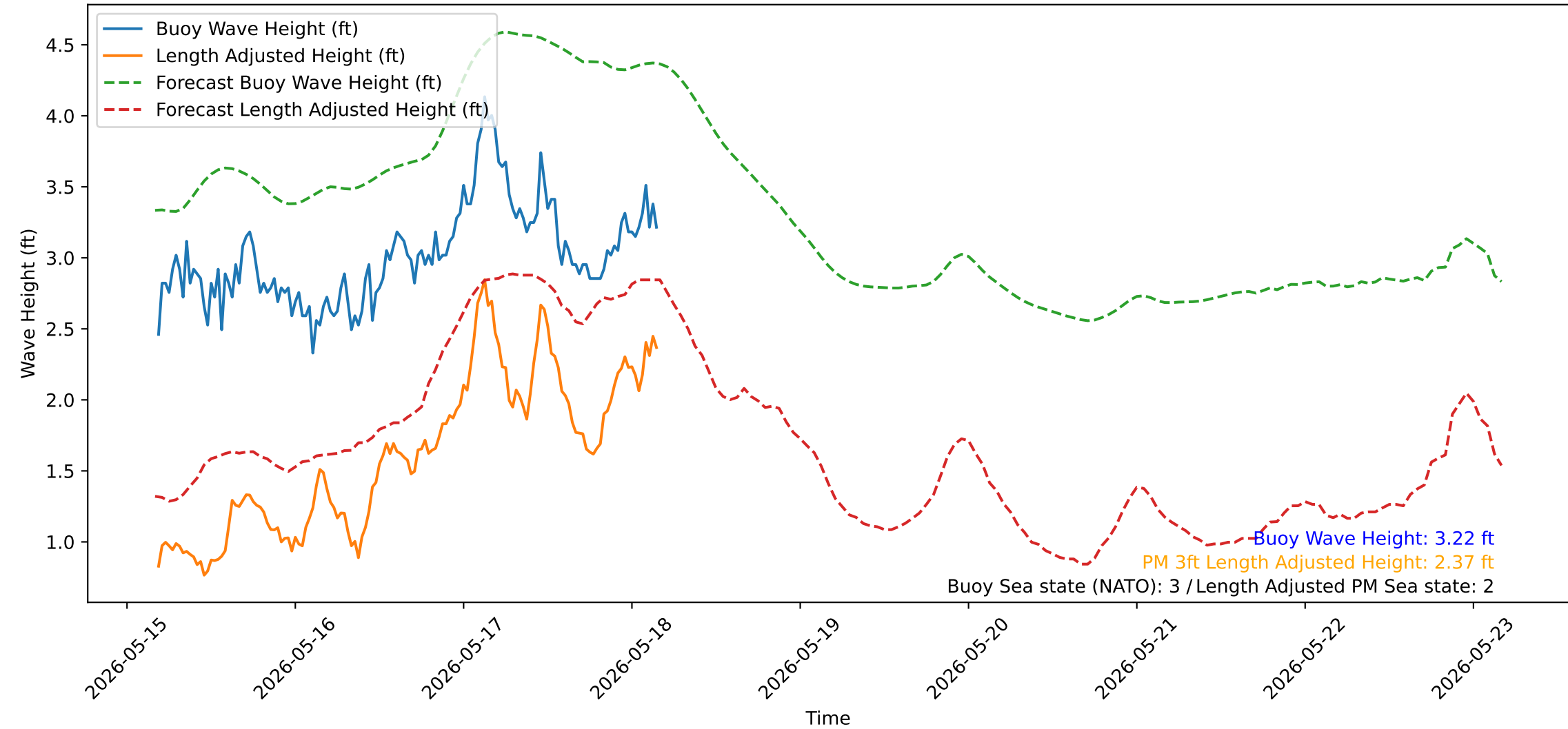
Wave Heights over Time for Red Beach at 2026-05-18 04:10:50
