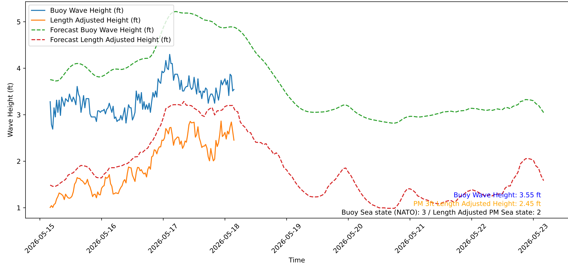
Wave Heights over Time for Oceanside Harbor at 2026-05-18 04:10:31
