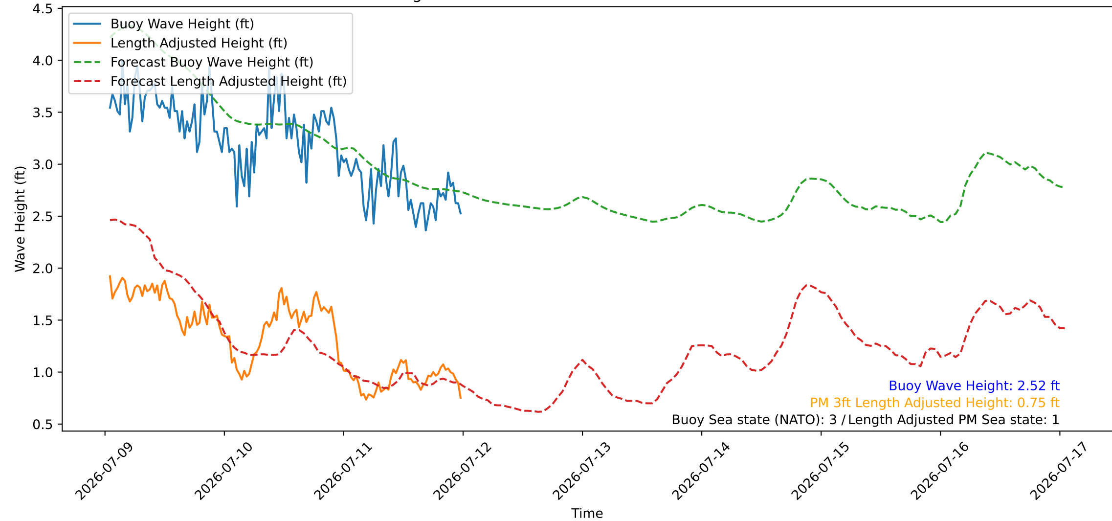
Wave Heights over Time for Red Beach at 2026-07-12 00:30:44
