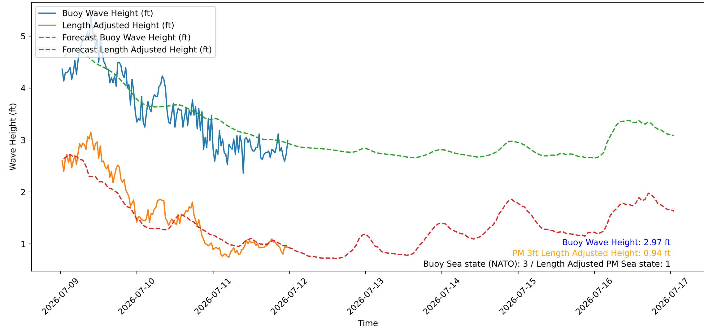
Wave Heights over Time for Oceanside Harbor at 2026-07-12 00:30:26
