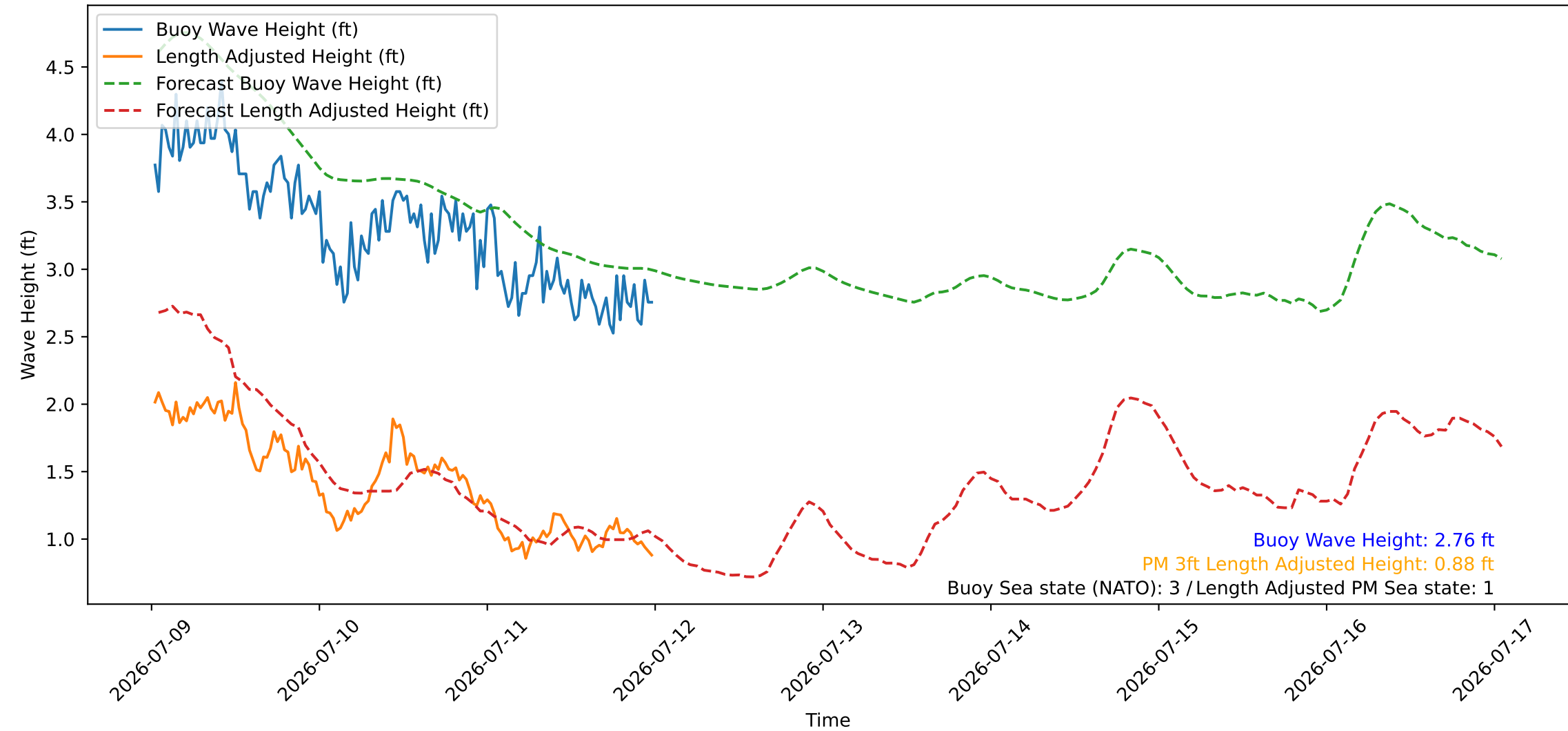
Wave Heights over Time for Green Beach at 2026-07-12 00:31:07
