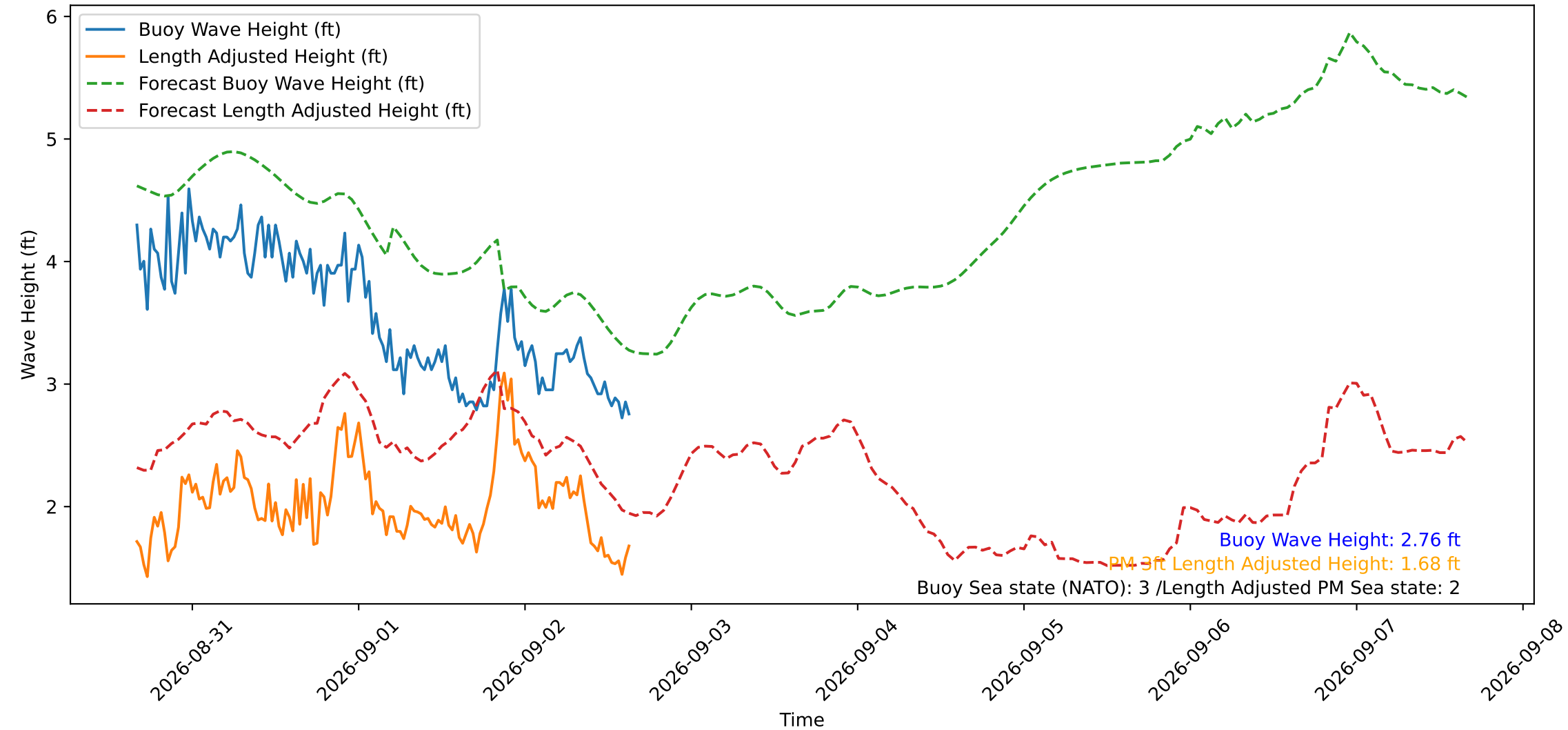
Wave Heights over Time for Green Beach at 2026-09-02 15:51:15
