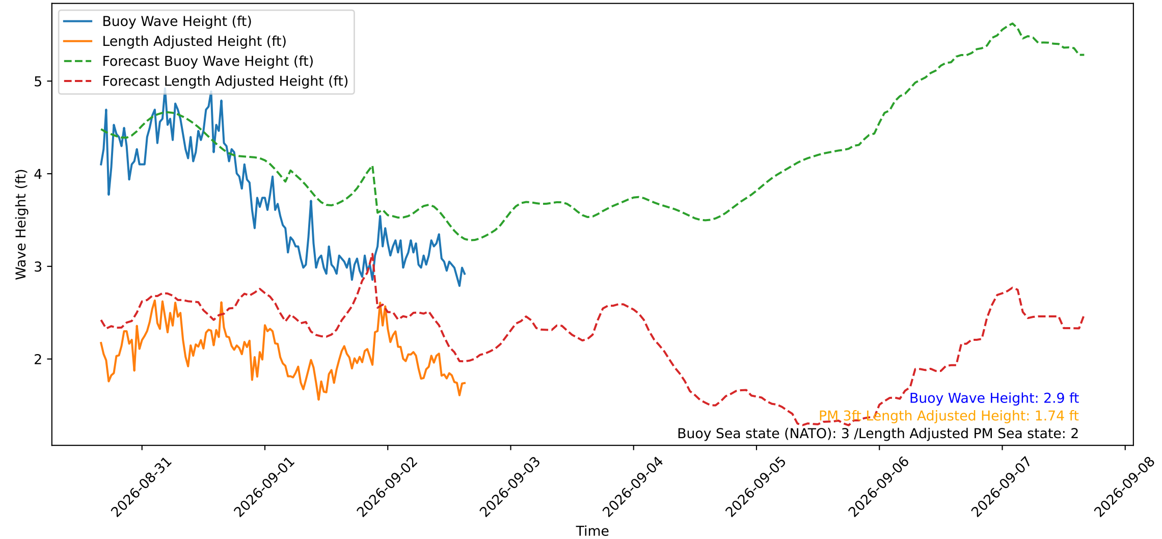
Wave Heights over Time for Oceanside Harbor at 2026-09-02 15:50:29
