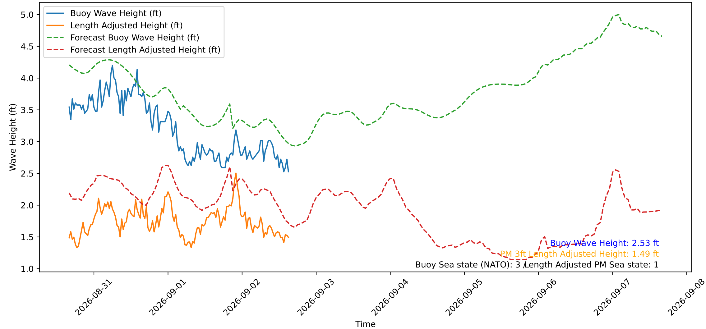
Wave Heights over Time for Red Beach at 2026-09-02 15:50:51
