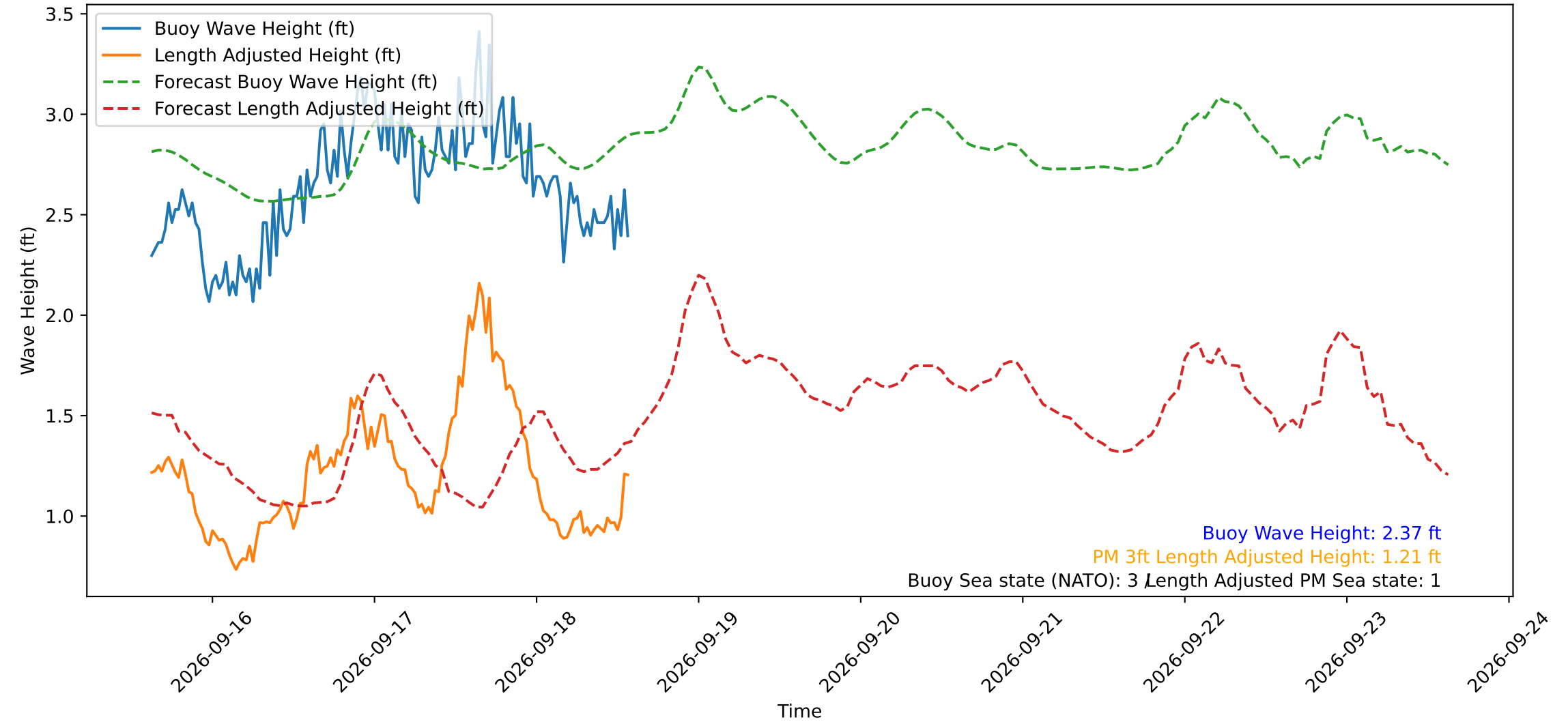
Wave Heights over Time for Red Beach at 2026-09-18 14:50:51
