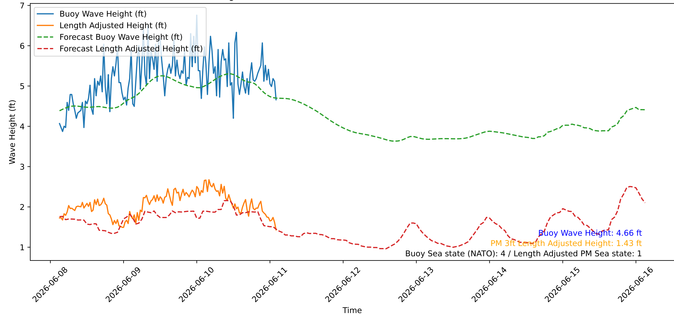
Wave Heights over Time for Oceanside Harbor at 2026-06-11 02:50:26
