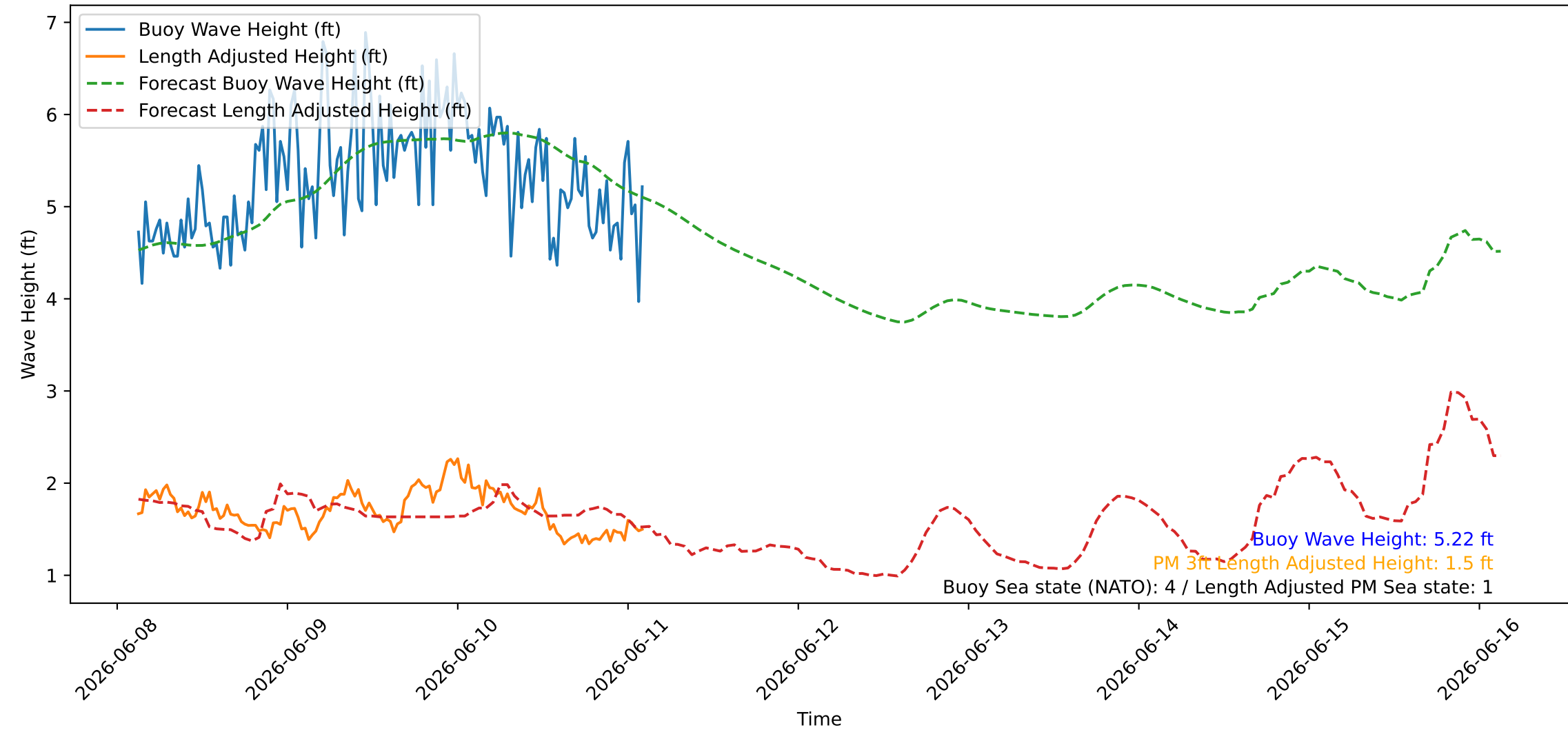
Wave Heights over Time for Green Beach at 2026-06-11 02:51:11
