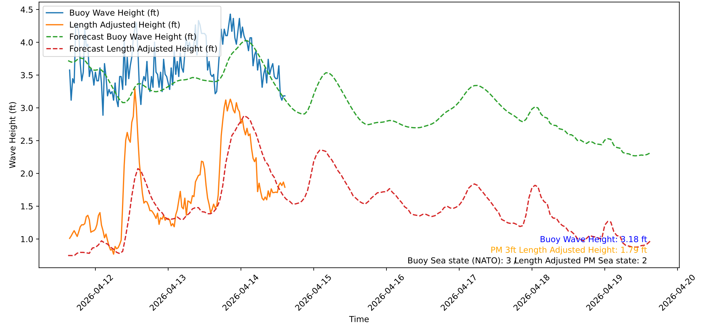
Wave Heights over Time for Red Beach at 2026-04-14 15:10:51
