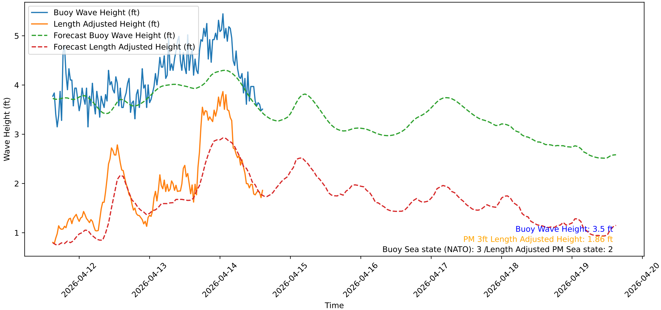
Wave Heights over Time for Oceanside Harbor at 2026-04-14 15:10:31
