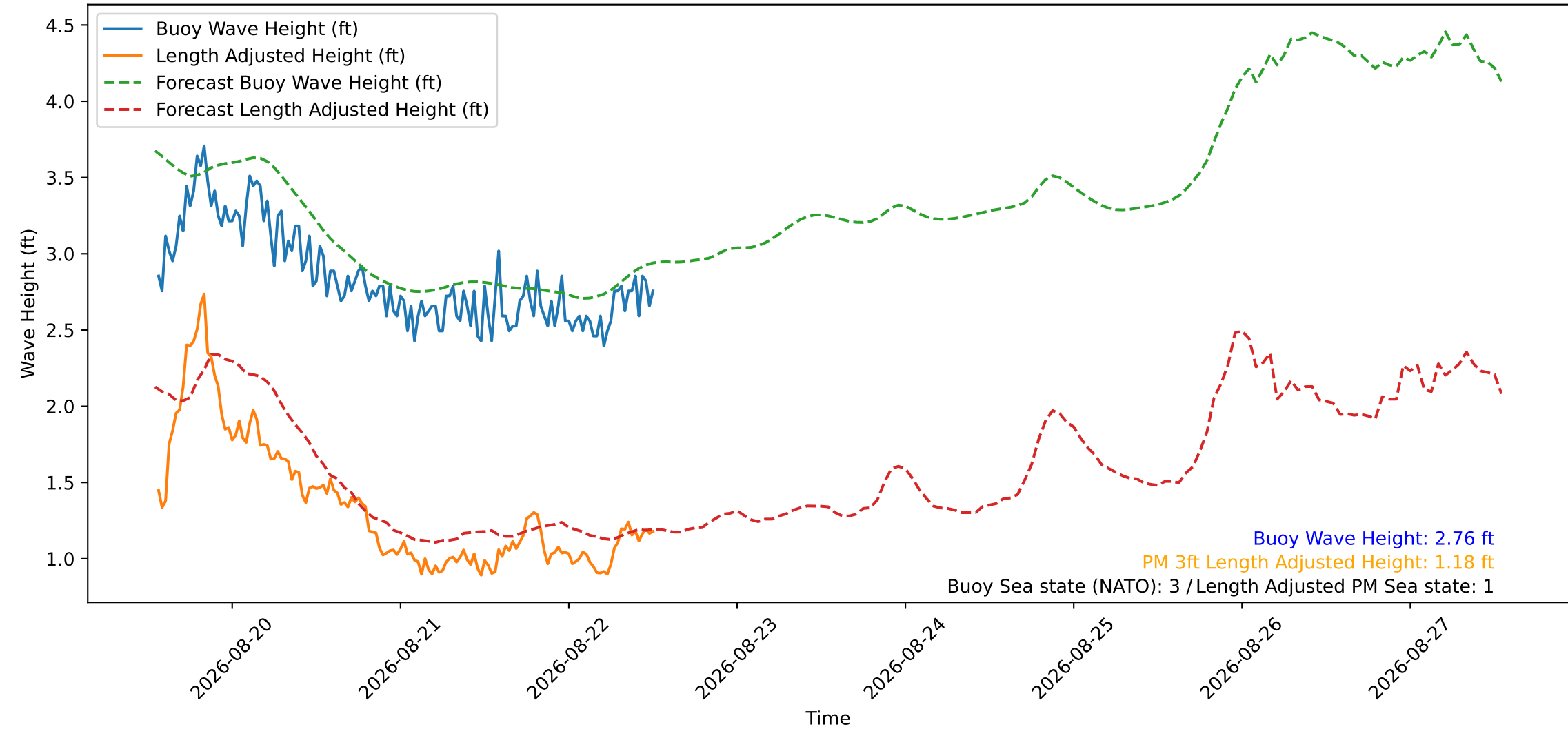
Wave Heights over Time for Green Beach at 2026-08-22 13:01:11
