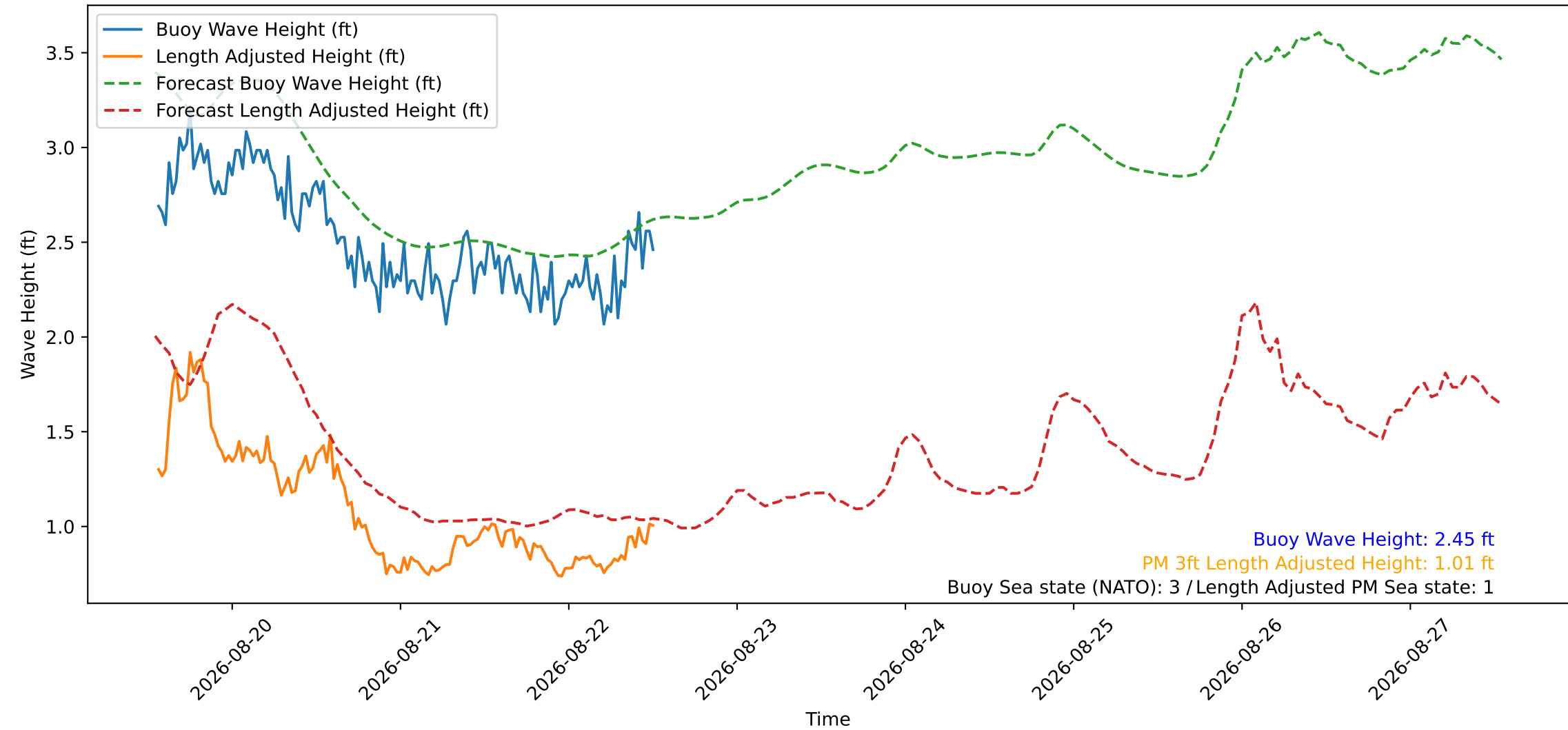
Wave Heights over Time for Red Beach at 2026-08-22 13:00:49
