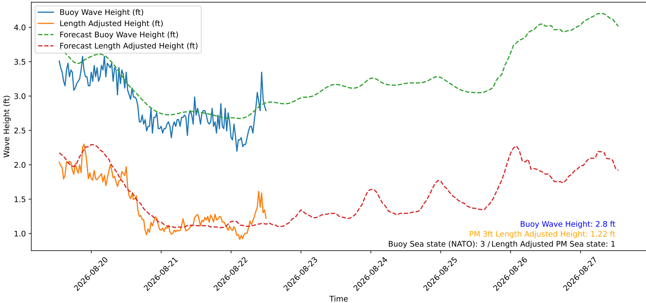
Wave Heights over Time for Oceanside Harbor at 2026-08-22 13:00:29
