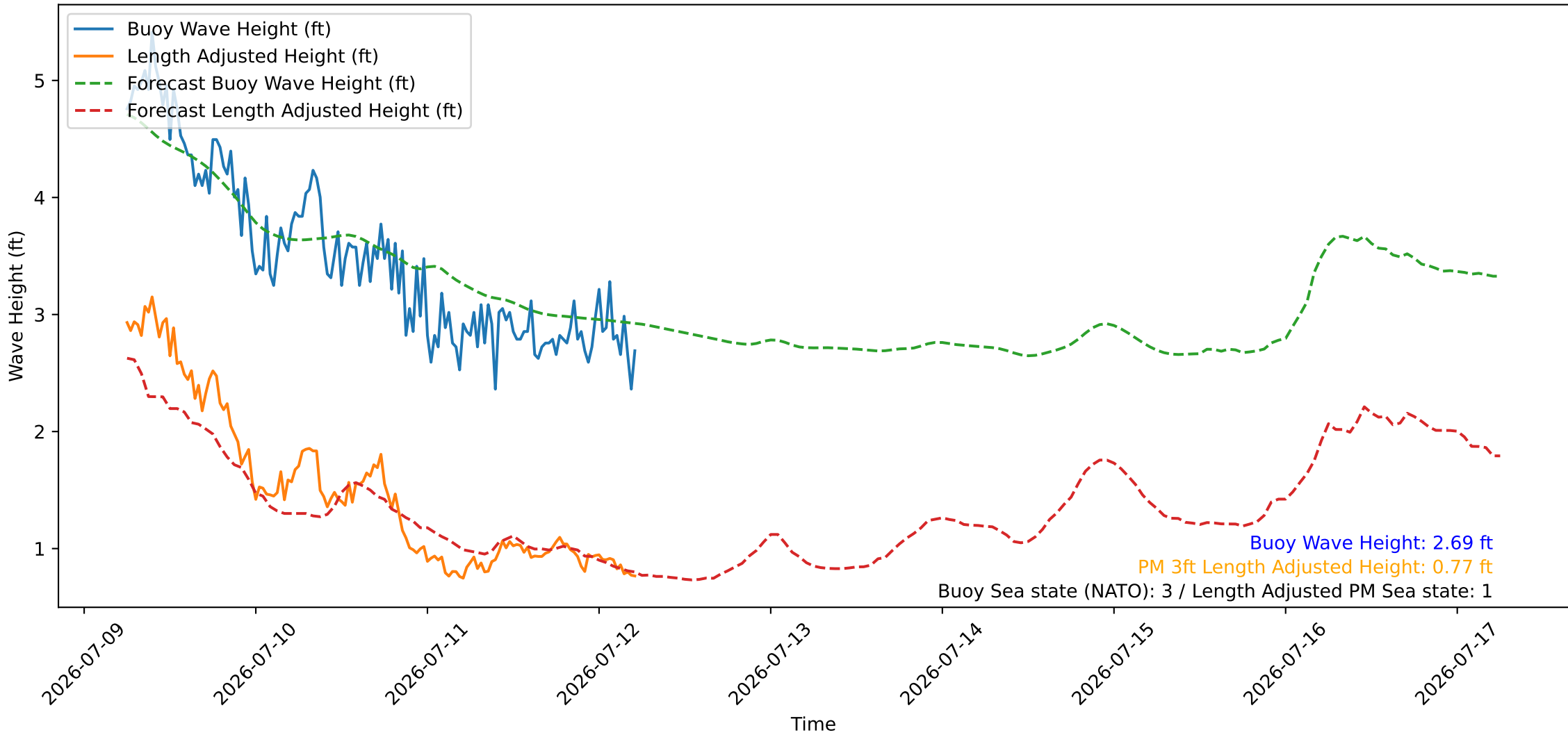
Wave Heights over Time for Oceanside Harbor at 2026-07-12 05:50:26
