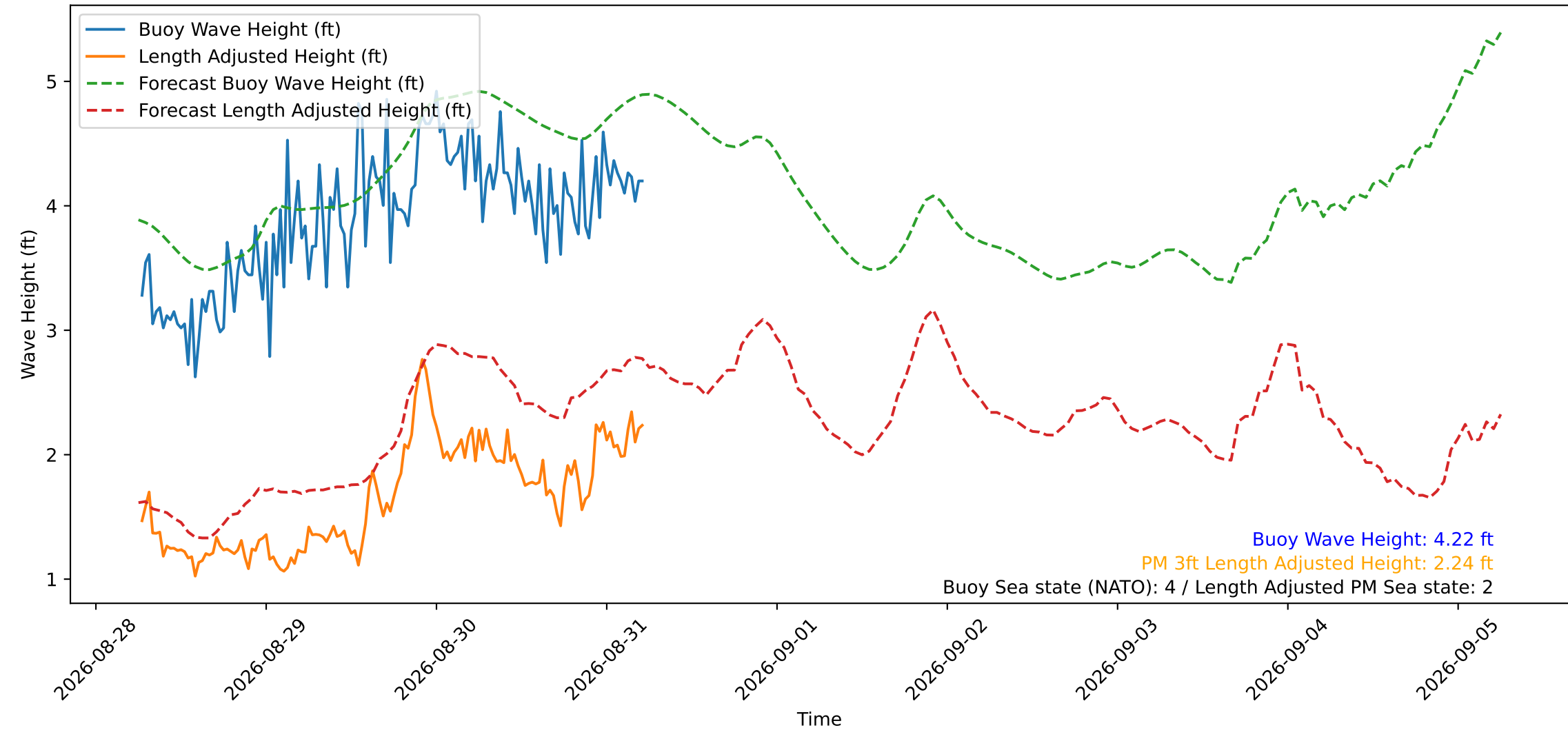
Wave Heights over Time for Green Beach at 2026-08-31 06:01:12
