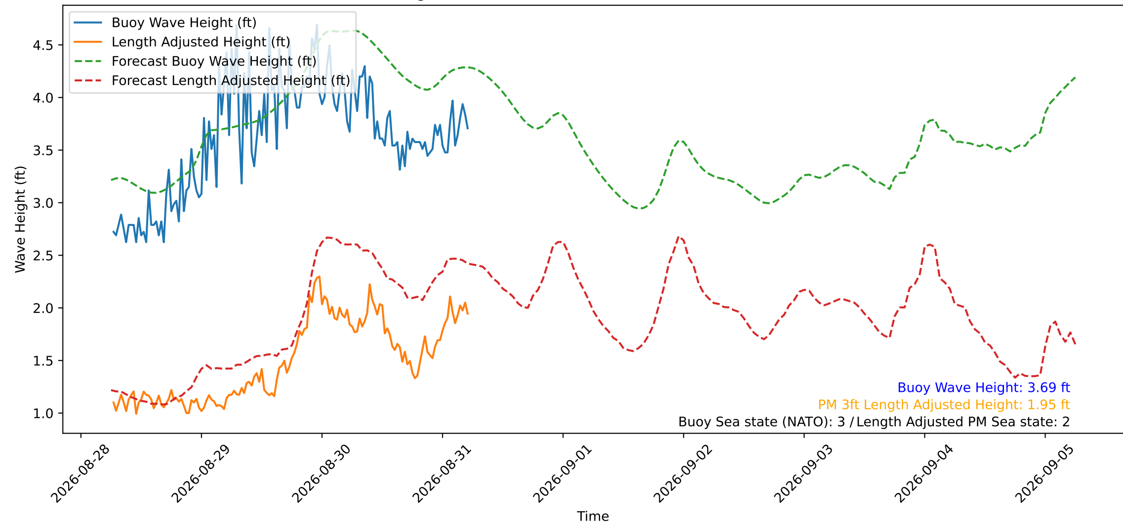
Wave Heights over Time for Red Beach at 2026-08-31 06:00:49
