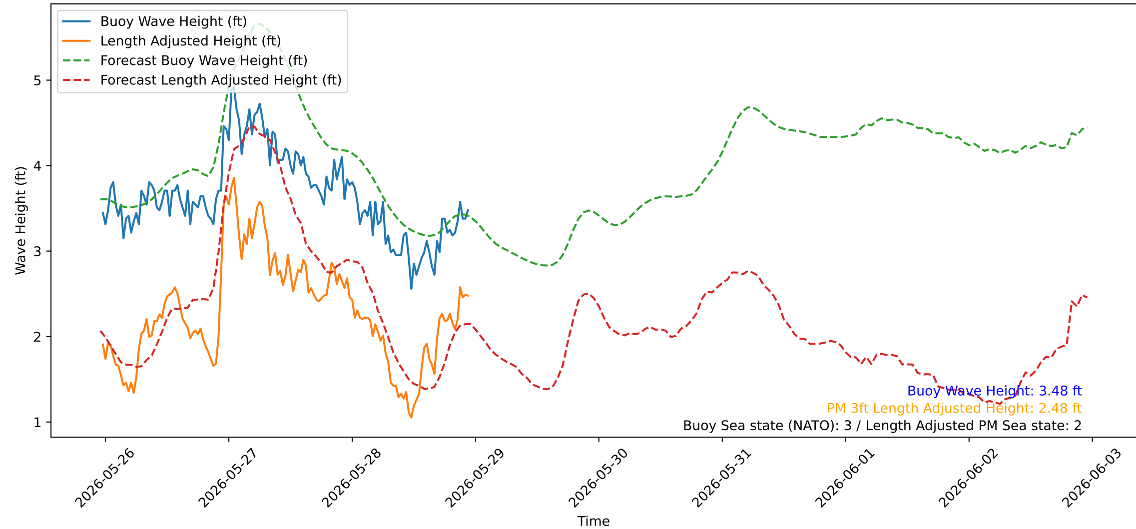
Wave Heights over Time for Green Beach at 2026-05-28 23:21:03
