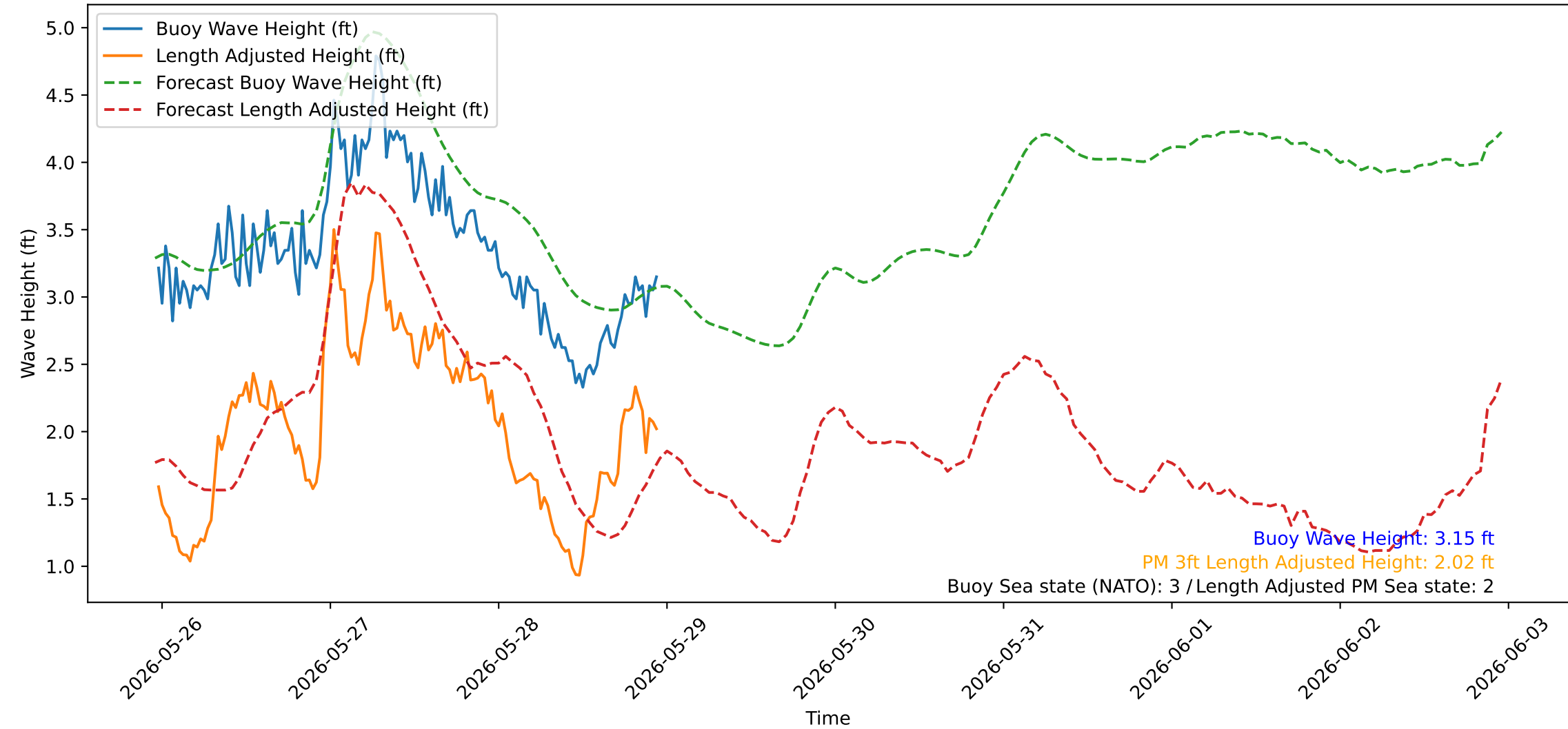
Wave Heights over Time for Red Beach at 2026-05-28 23:20:40
