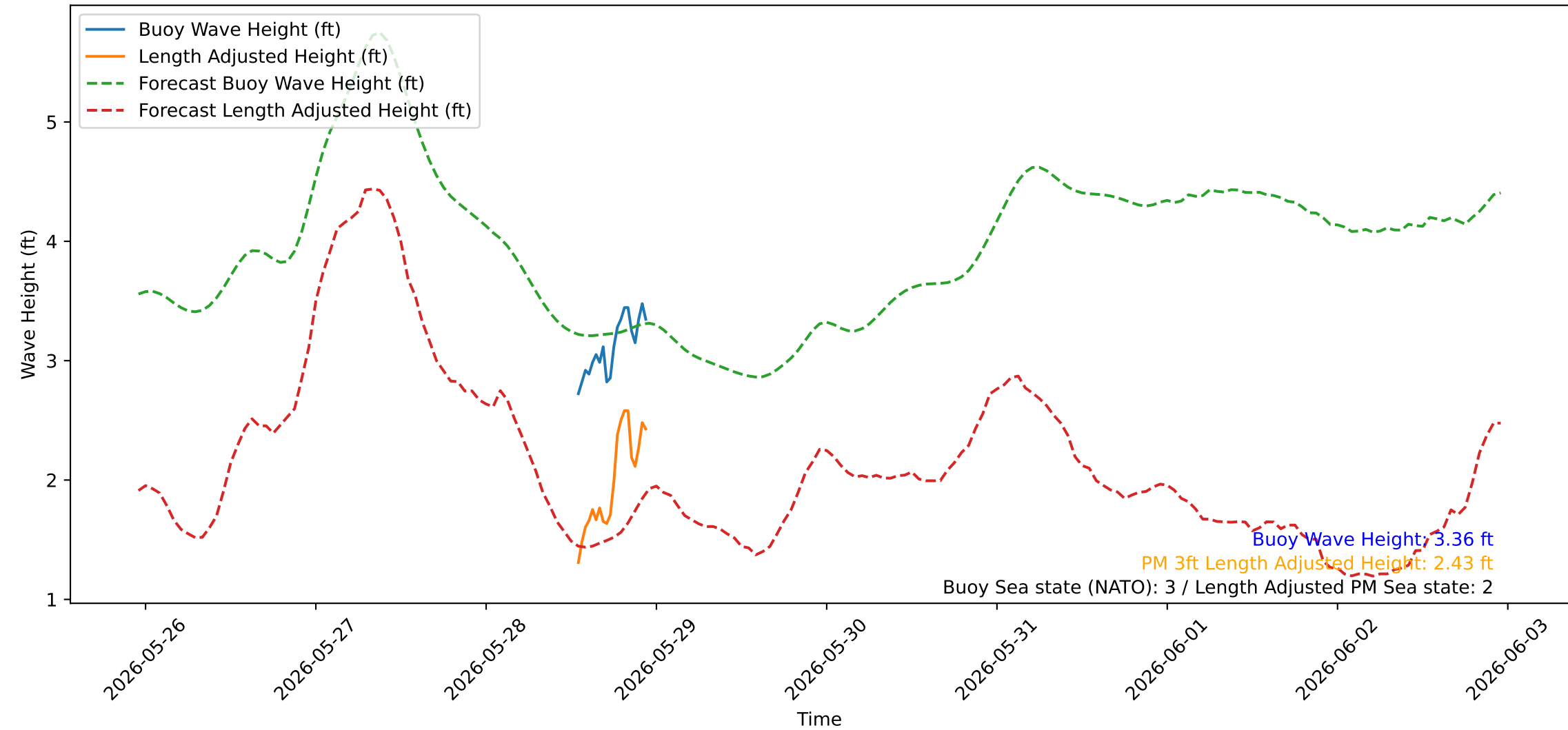
Wave Heights over Time for Oceanside Harbor at 2026-05-28 23:20:20
