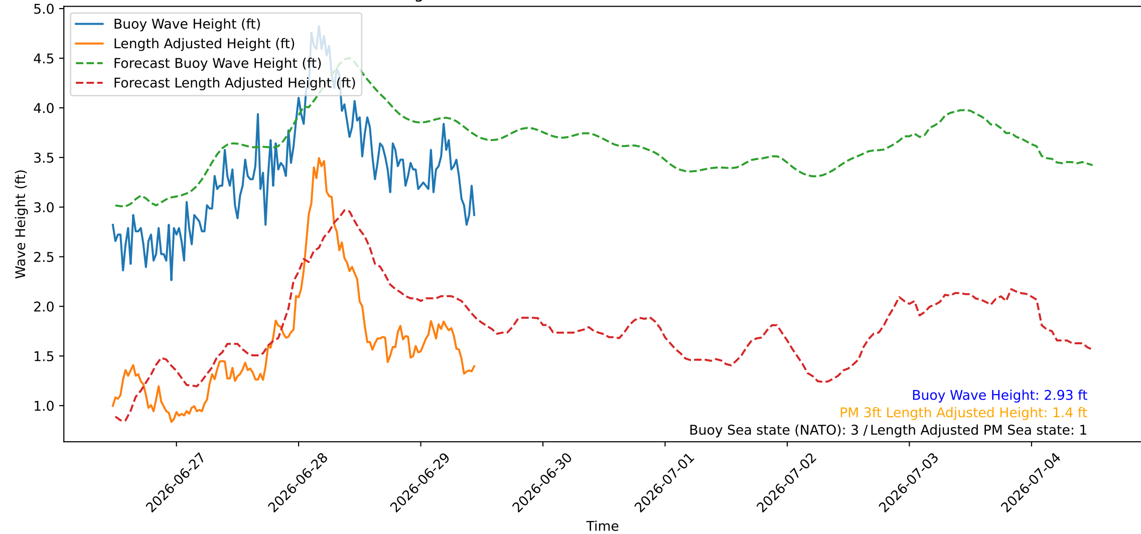
Wave Heights over Time for Green Beach at 2026-06-29 11:31:07
