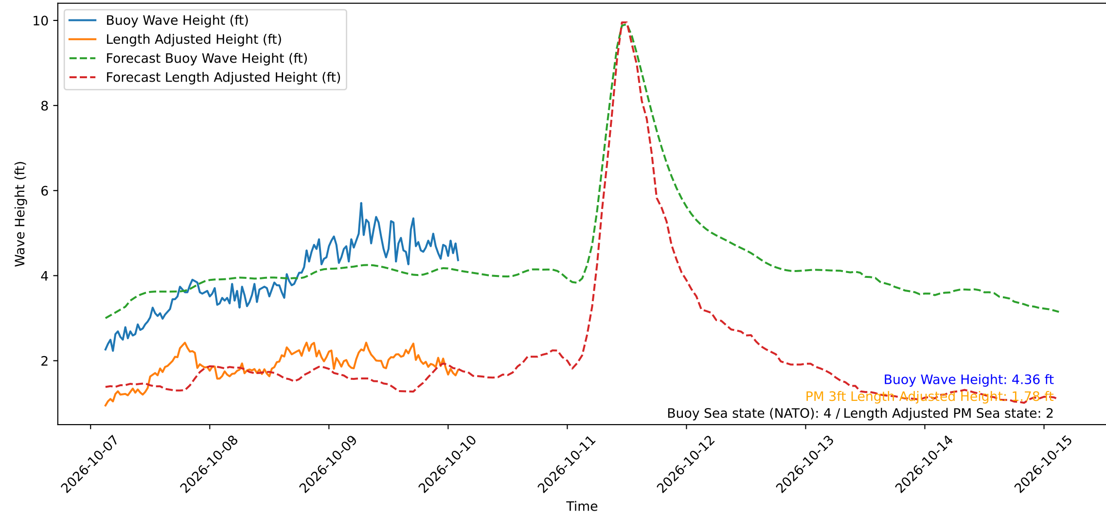
Wave Heights over Time for Red Beach at 2026-10-10 02:50:50
