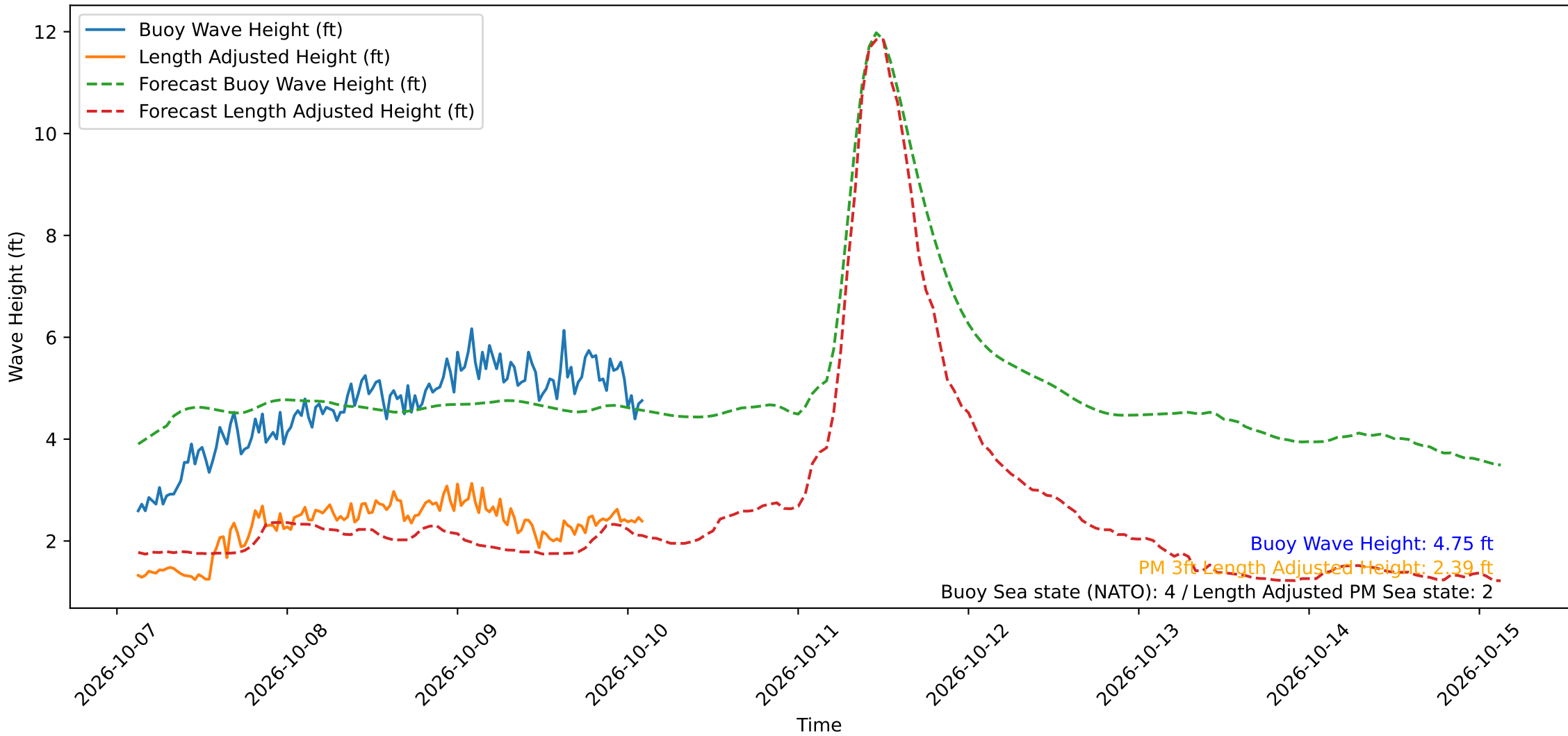
Wave Heights over Time for Green Beach at 2026-10-10 02:51:14
