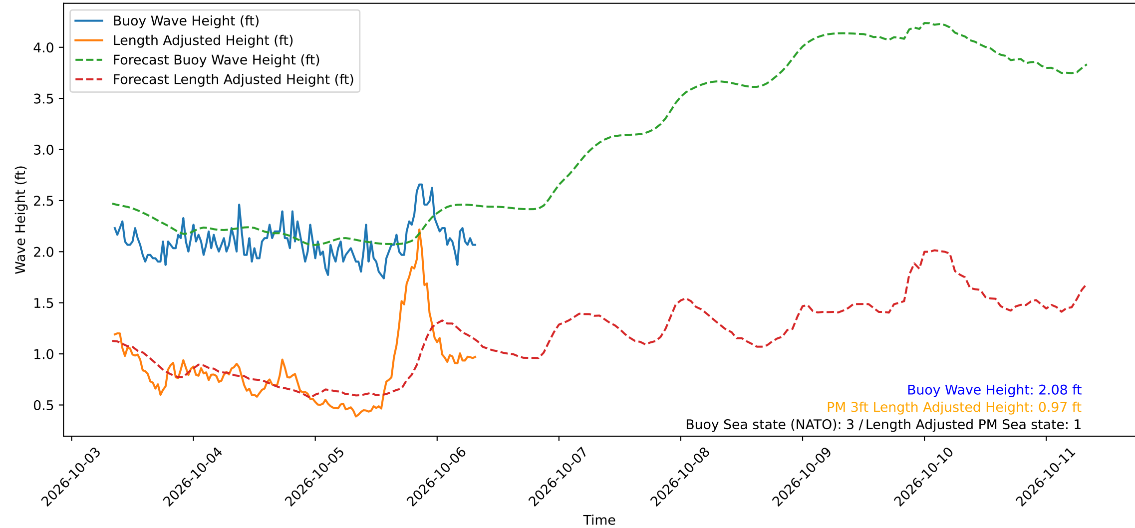
Wave Heights over Time for Red Beach at 2026-10-06 08:10:50
