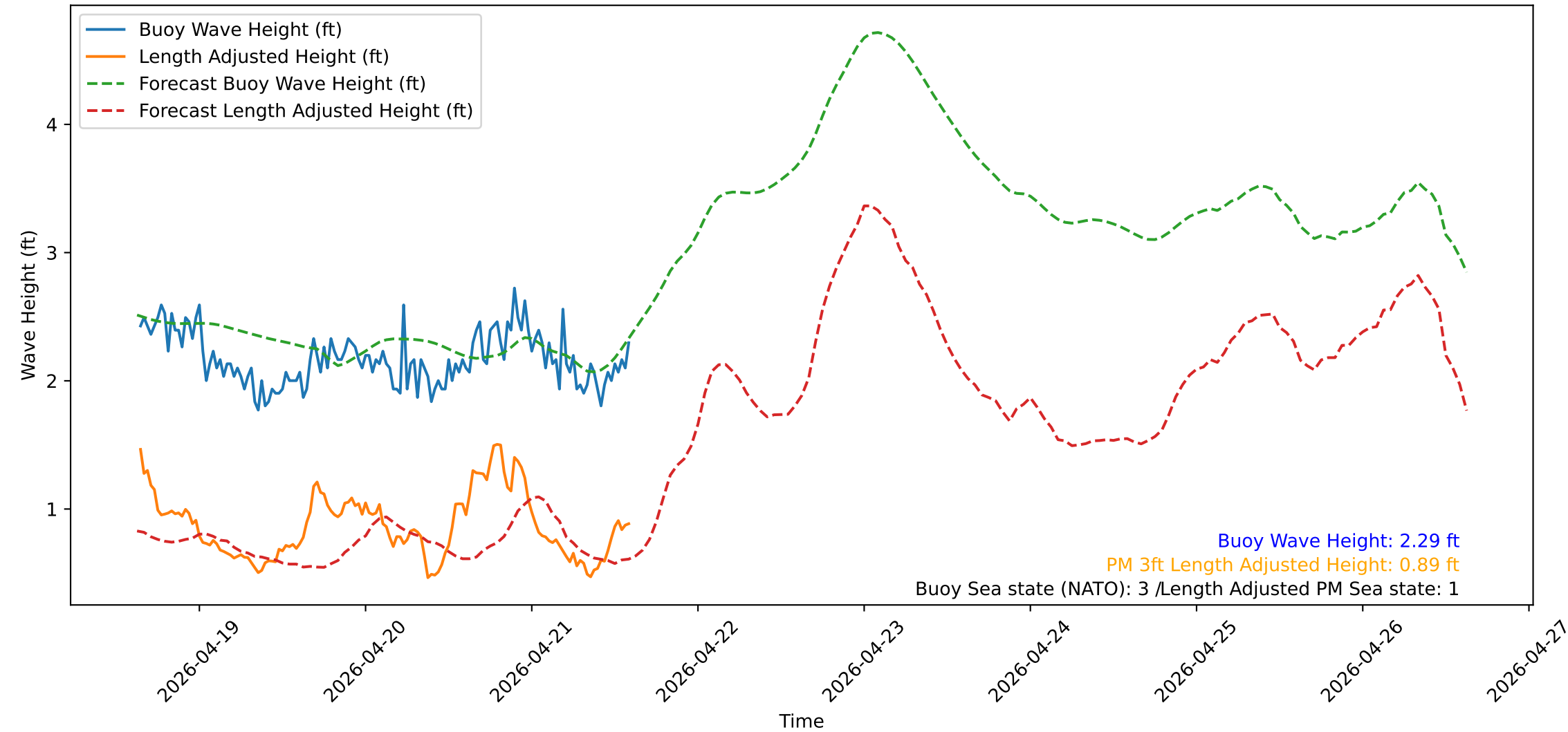
Wave Heights over Time for Red Beach at 2026-04-21 15:10:50
