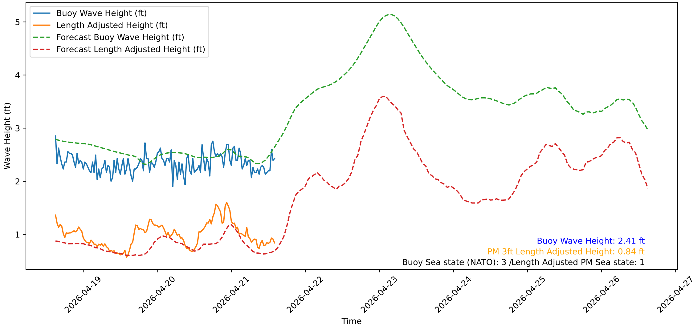
Wave Heights over Time for Oceanside Harbor at 2026-04-21 15:10:31
