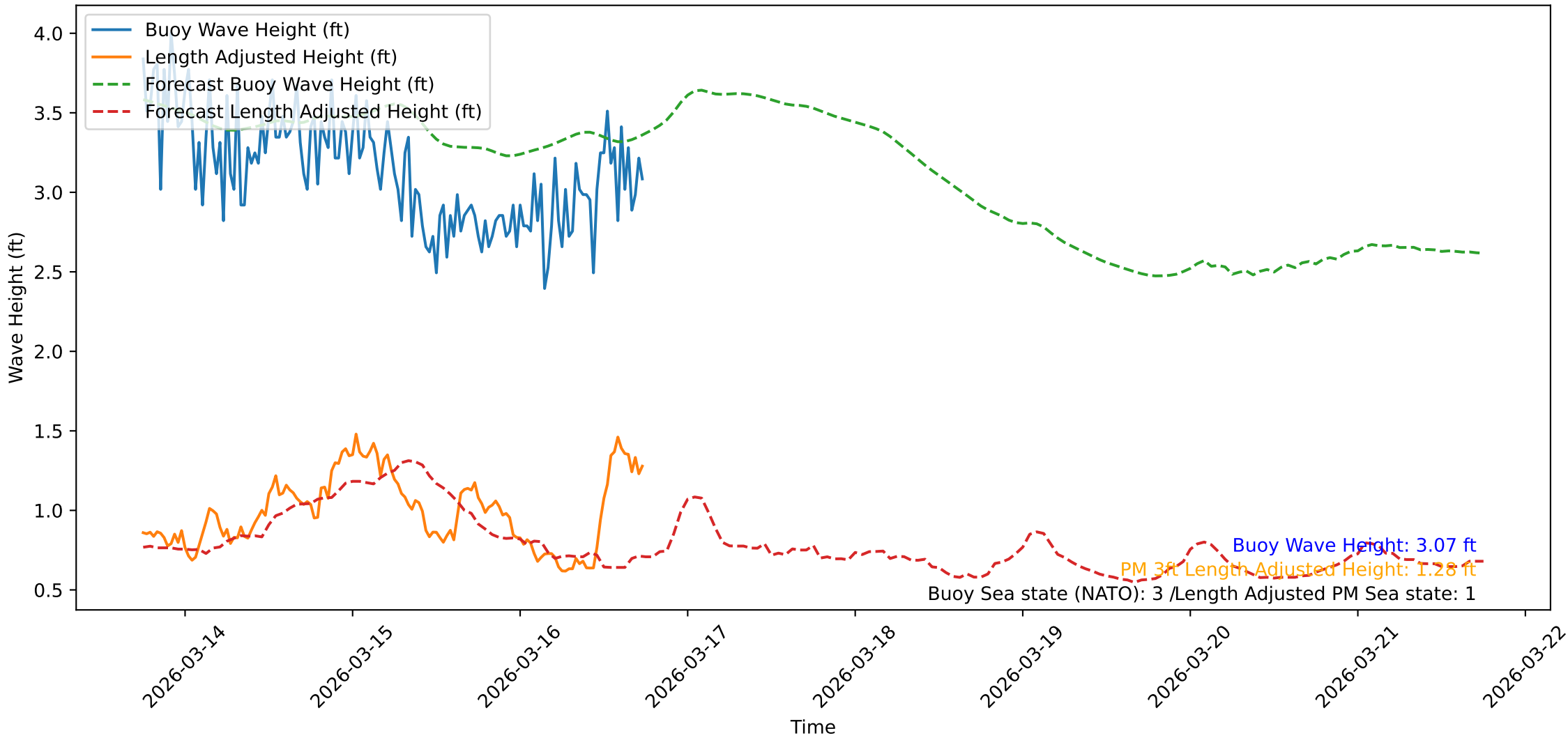
Wave Heights over Time for Oceanside Harbor at 2026-03-16 18:10:43
