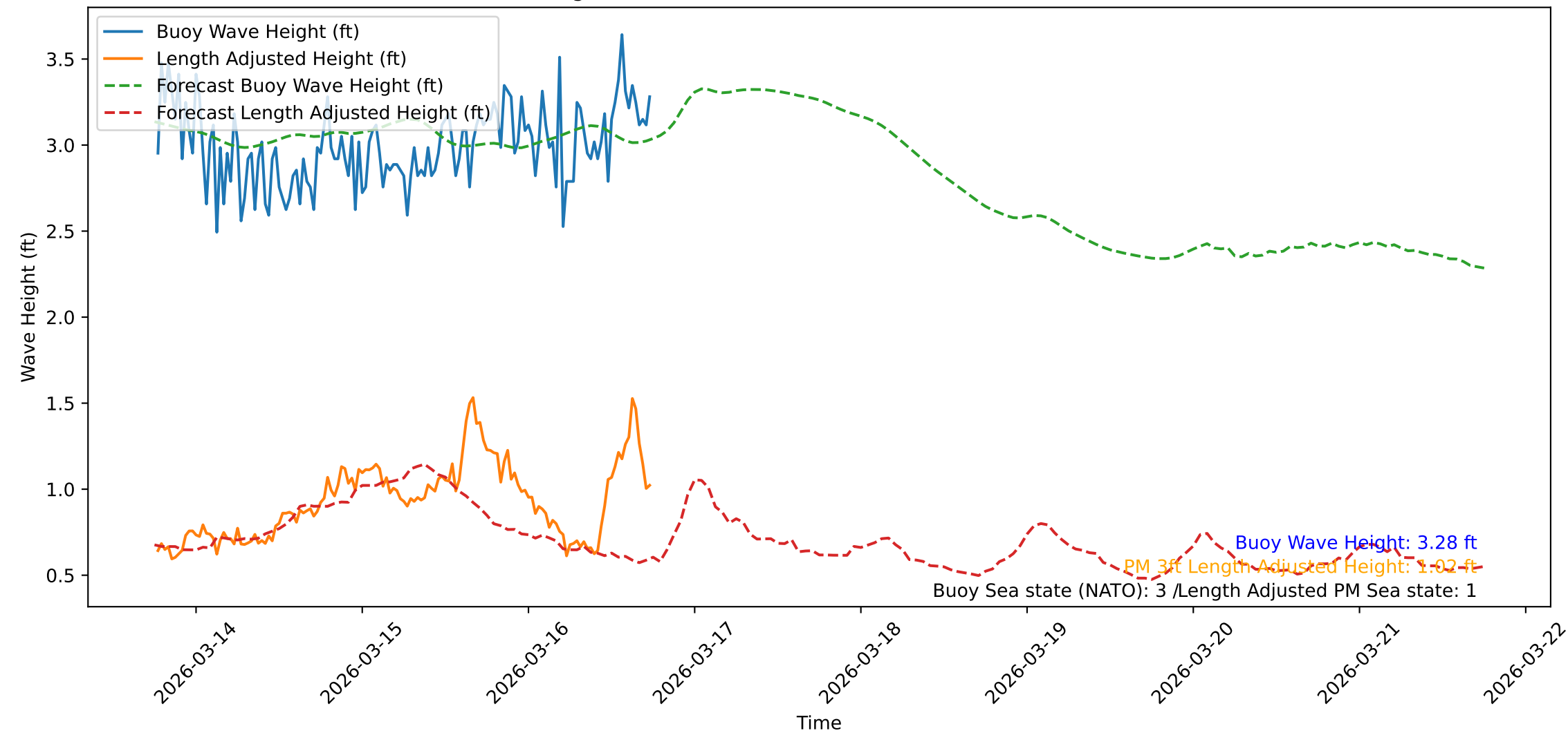
Wave Heights over Time for Red Beach at 2026-03-16 18:11:04
