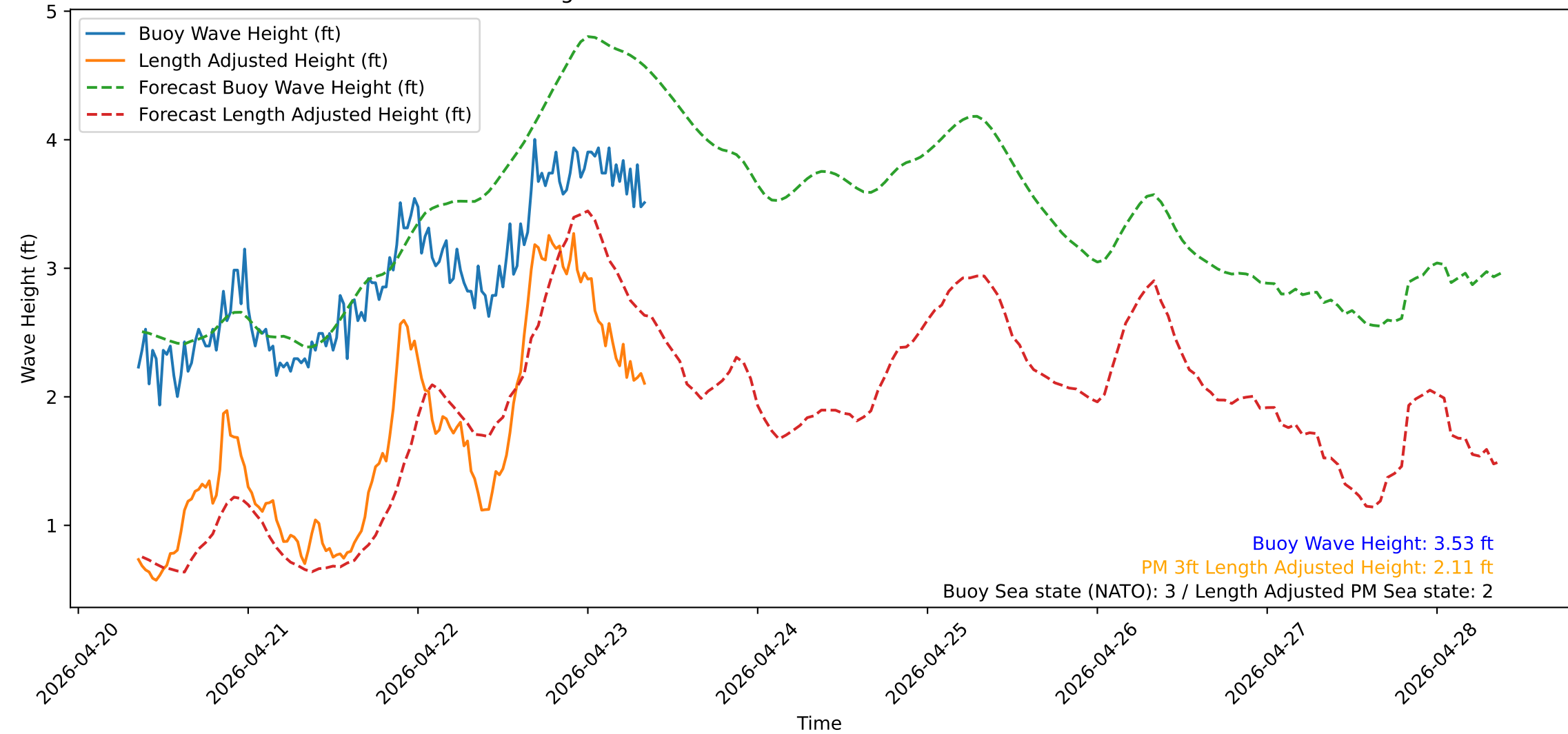
Wave Heights over Time for Green Beach at 2026-04-23 08:41:13
