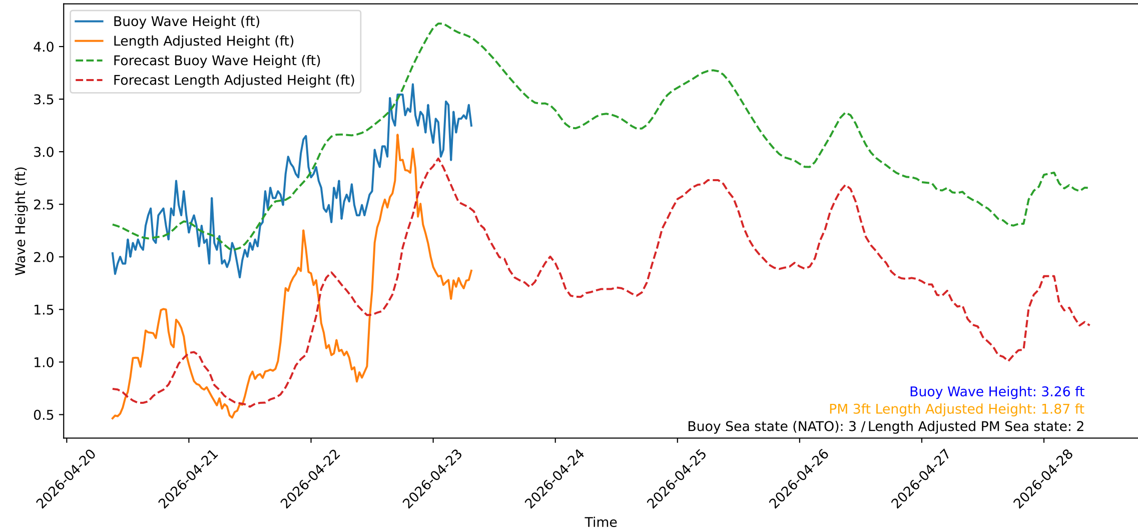
Wave Heights over Time for Red Beach at 2026-04-23 08:40:50
