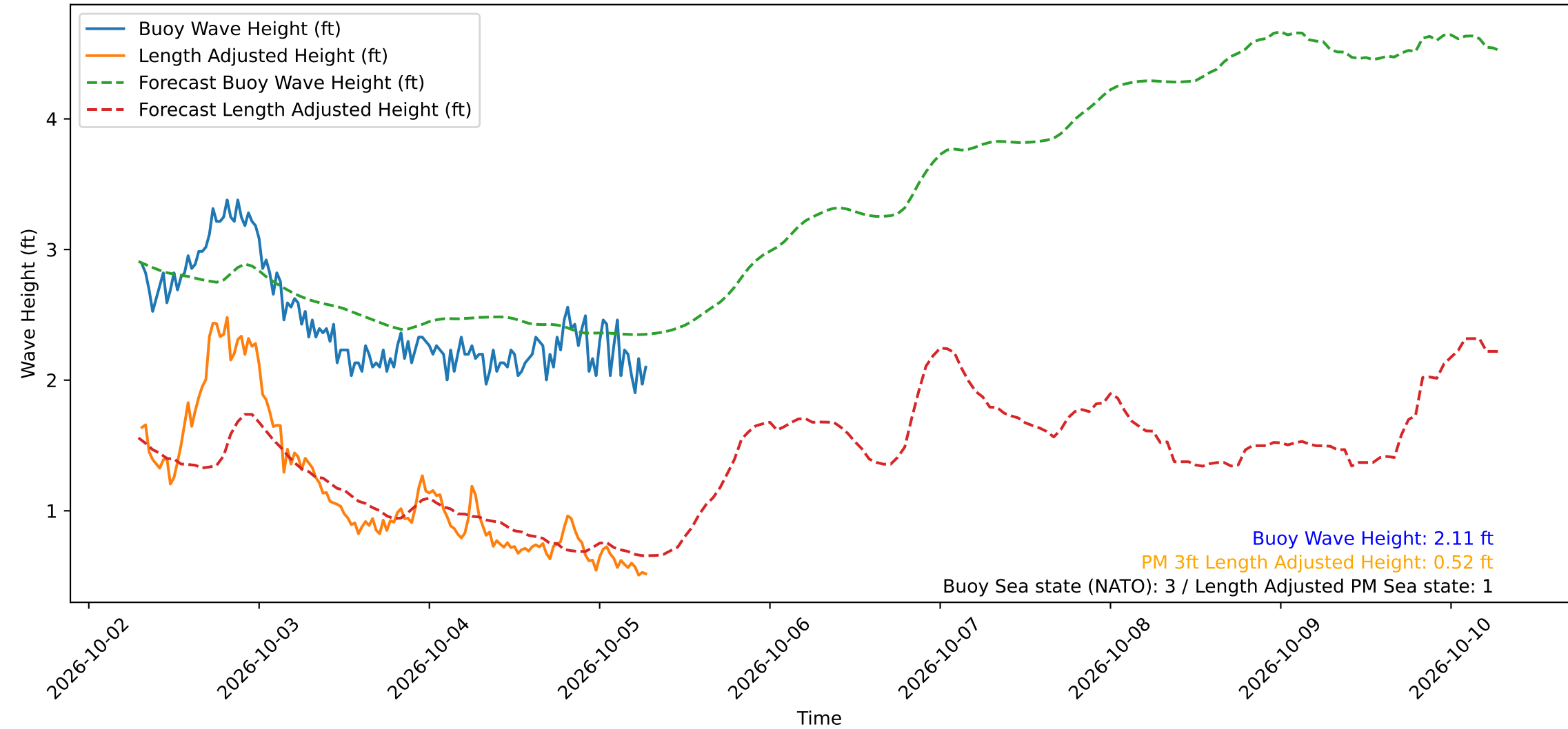
Wave Heights over Time for Green Beach at 2026-10-05 07:21:14
