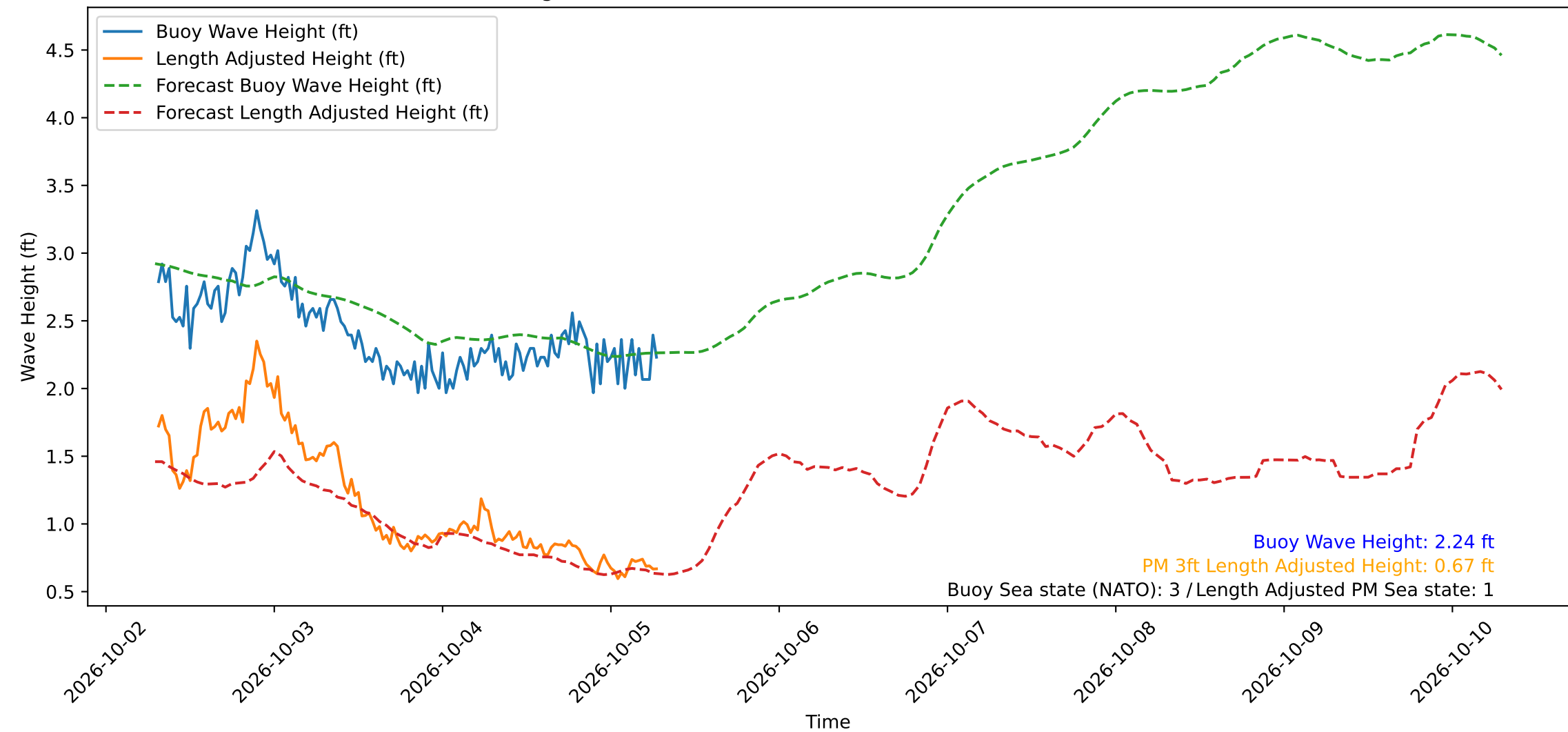
Wave Heights over Time for Oceanside Harbor at 2026-10-05 07:20:30
