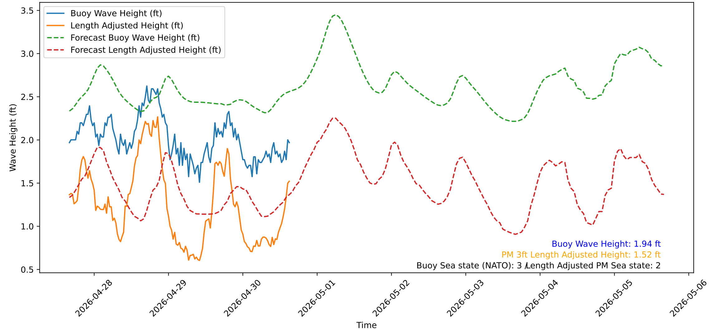
Wave Heights over Time for Red Beach at 2026-04-30 15:50:52
