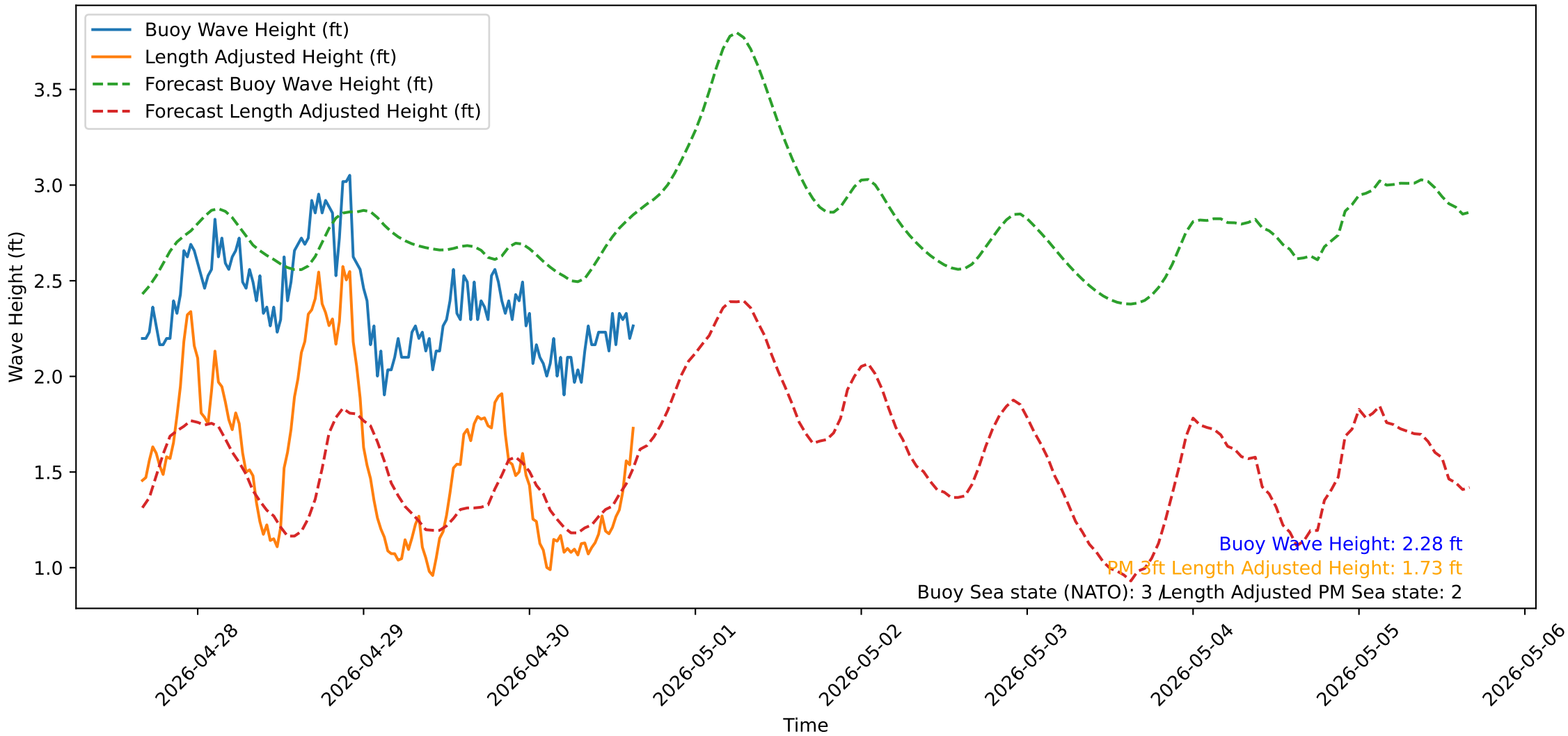
Wave Heights over Time for Oceanside Harbor at 2026-04-30 15:50:31
