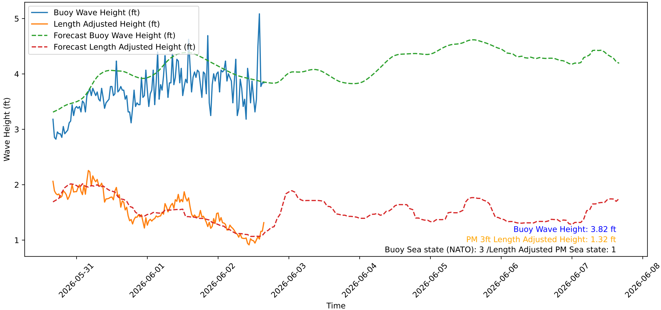
Wave Heights over Time for Oceanside Harbor at 2026-06-02 16:10:26
