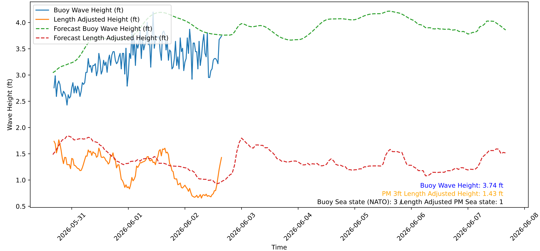
Wave Heights over Time for Red Beach at 2026-06-02 16:10:45
