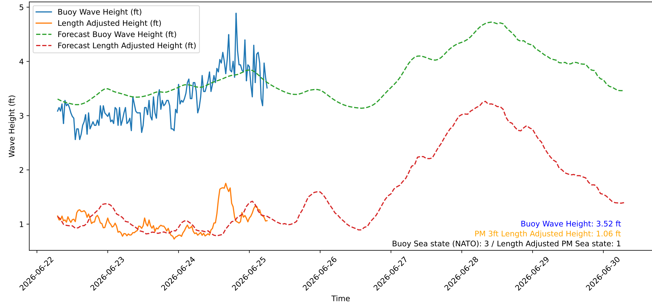
Wave Heights over Time for Oceanside Harbor at 2026-06-25 07:00:26
