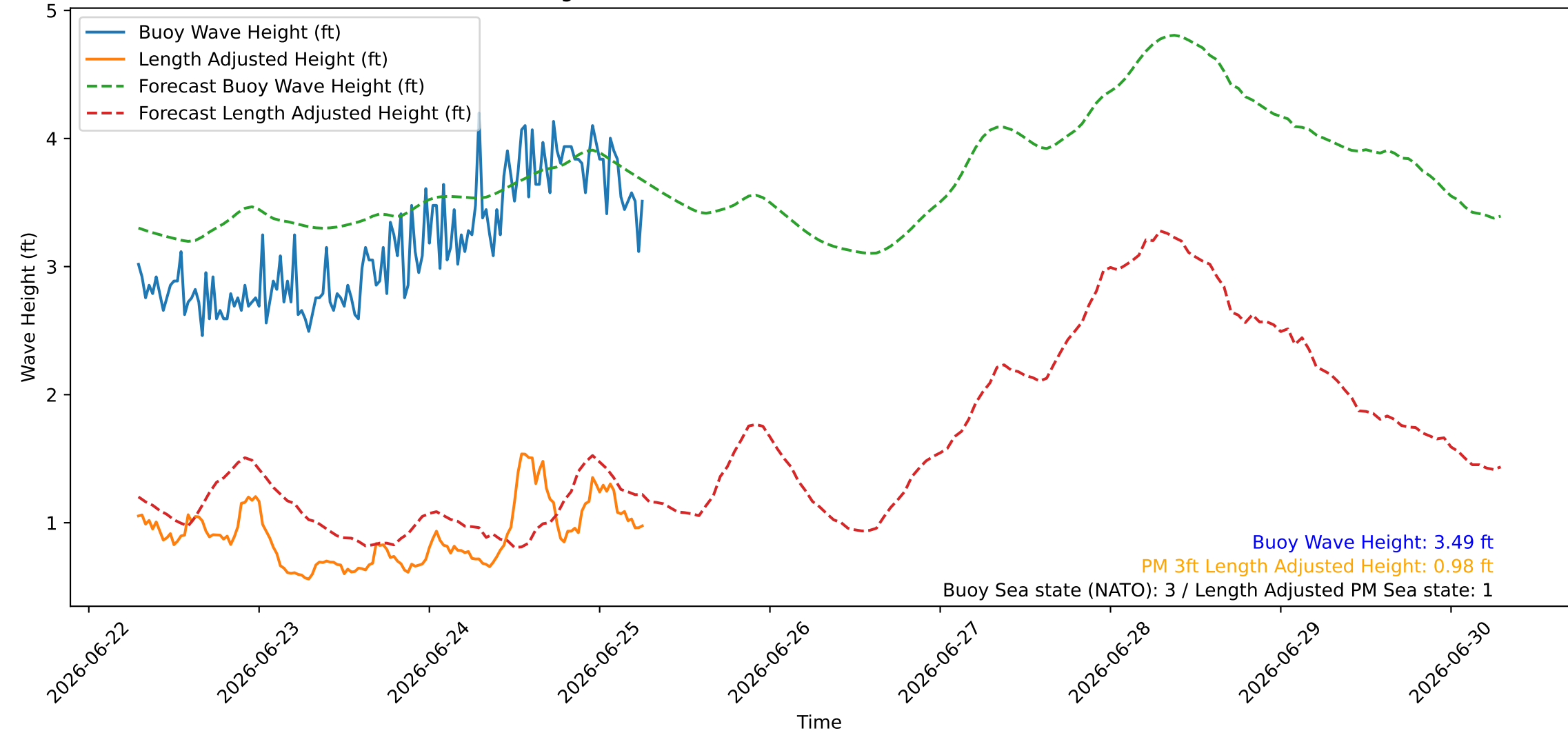
Wave Heights over Time for Green Beach at 2026-06-25 07:01:07
