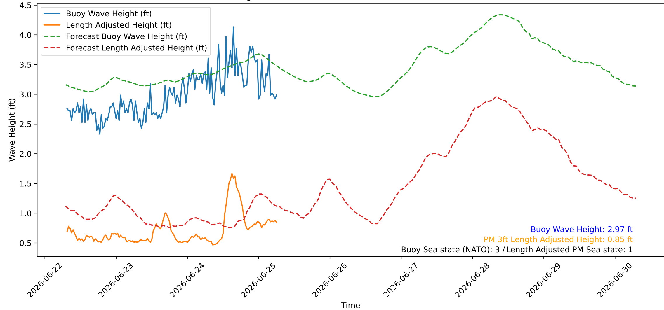
Wave Heights over Time for Red Beach at 2026-06-25 07:00:45
