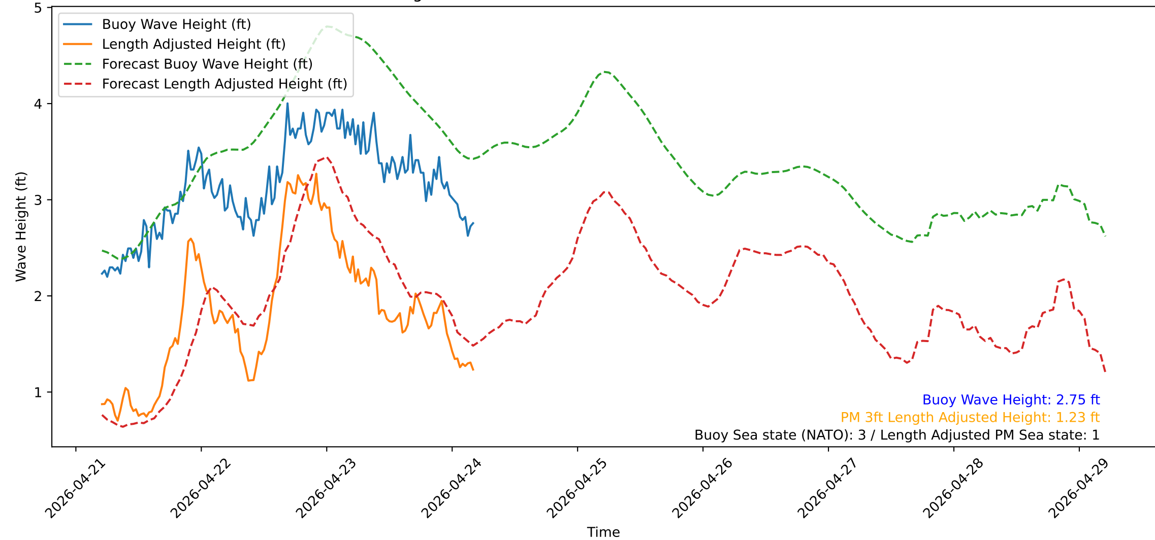
Wave Heights over Time for Green Beach at 2026-04-24 04:51:14
