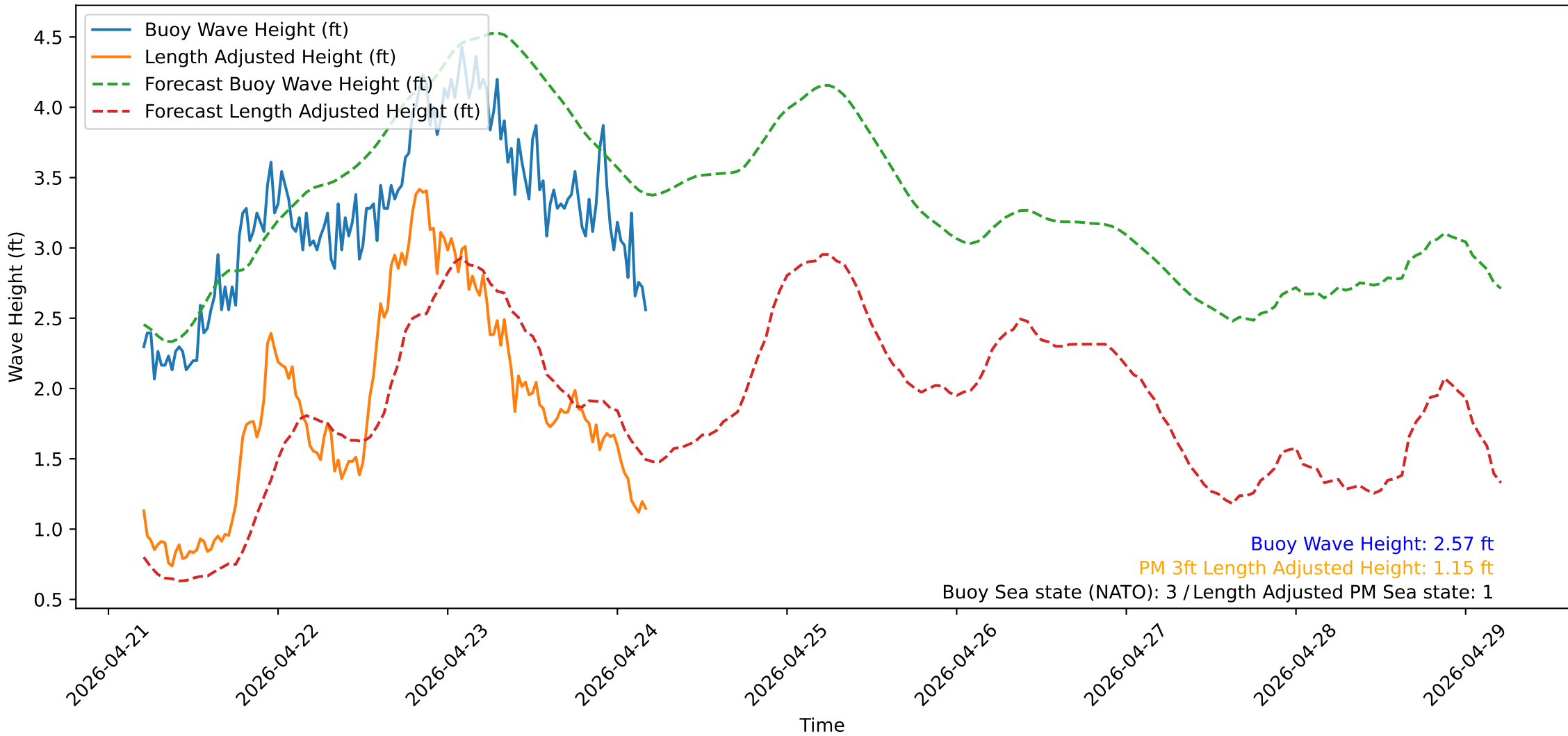
Wave Heights over Time for Oceanside Harbor at 2026-04-24 04:50:31
