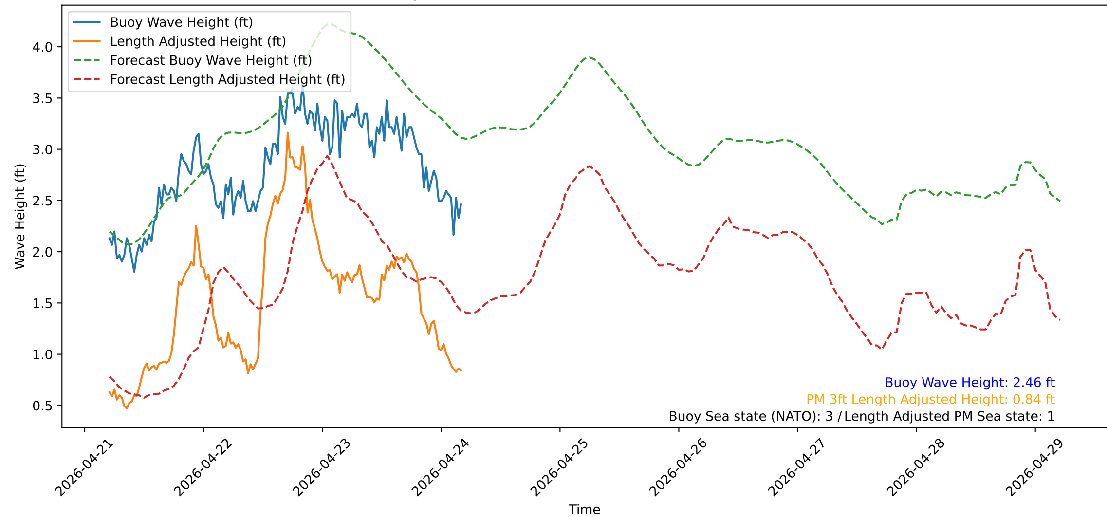
Wave Heights over Time for Red Beach at 2026-04-24 04:50:52
