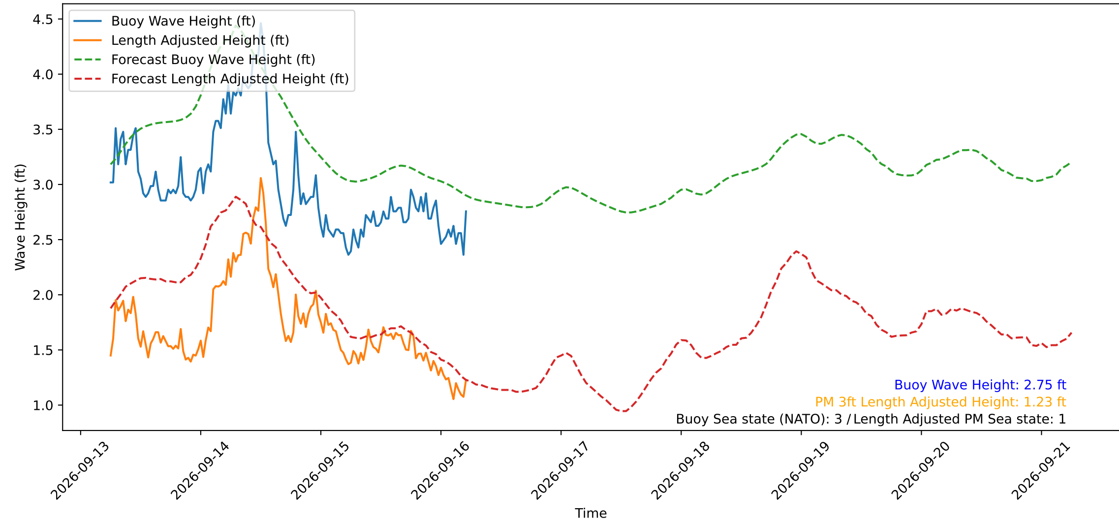
Wave Heights over Time for Oceanside Harbor at 2026-09-16 05:50:29
