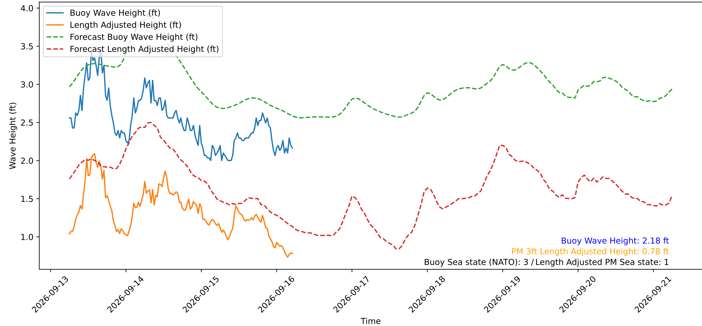
Wave Heights over Time for Red Beach at 2026-09-16 05:50:51
