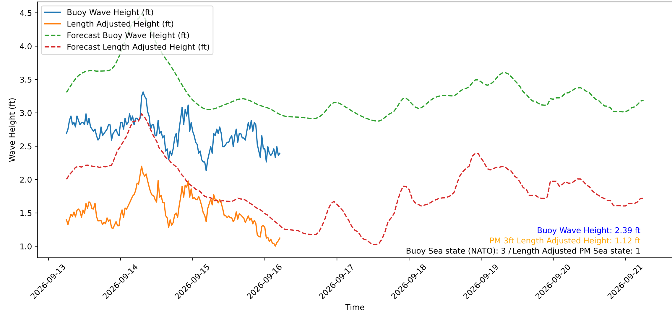
Wave Heights over Time for Green Beach at 2026-09-16 05:51:14
