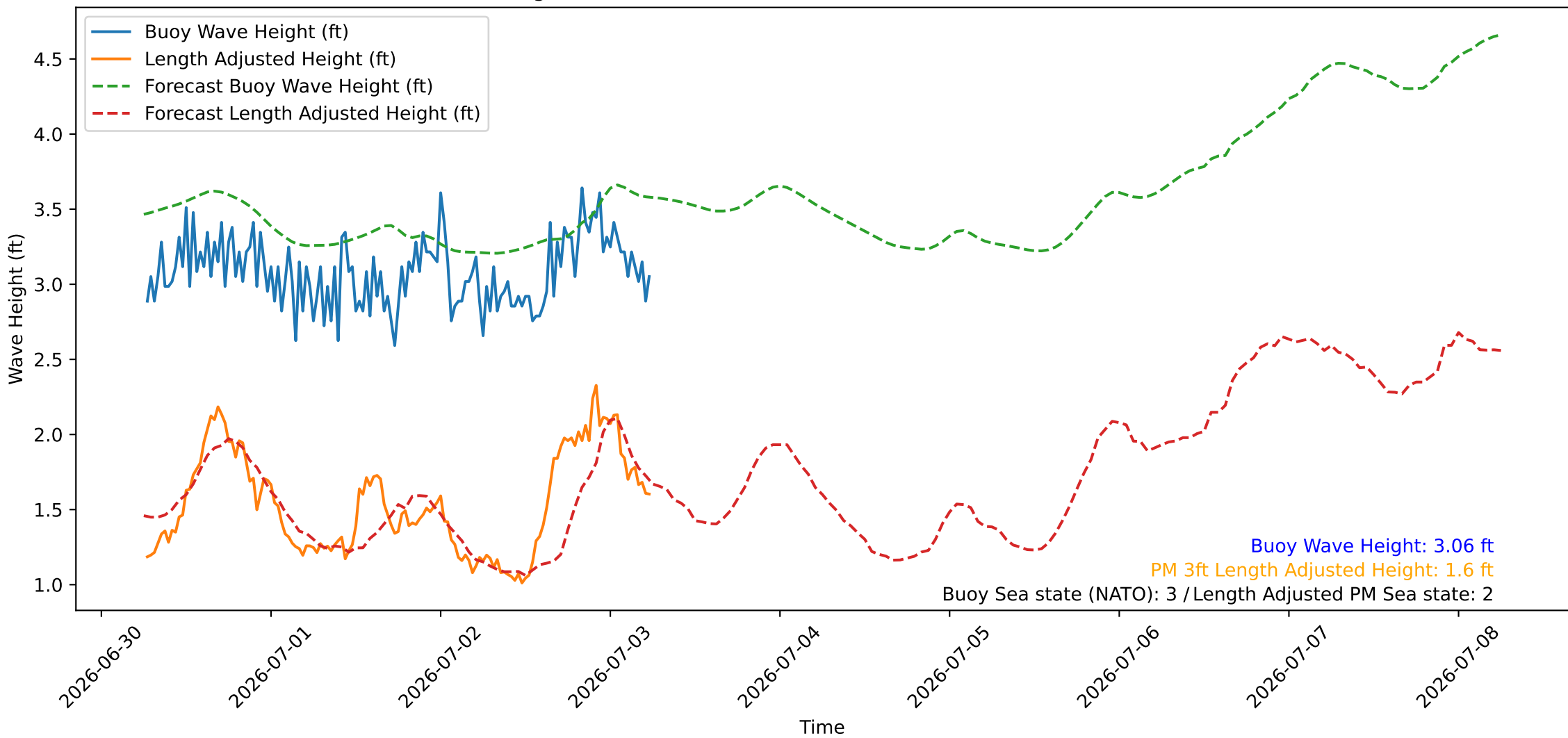
Wave Heights over Time for Oceanside Harbor at 2026-07-03 06:20:26
