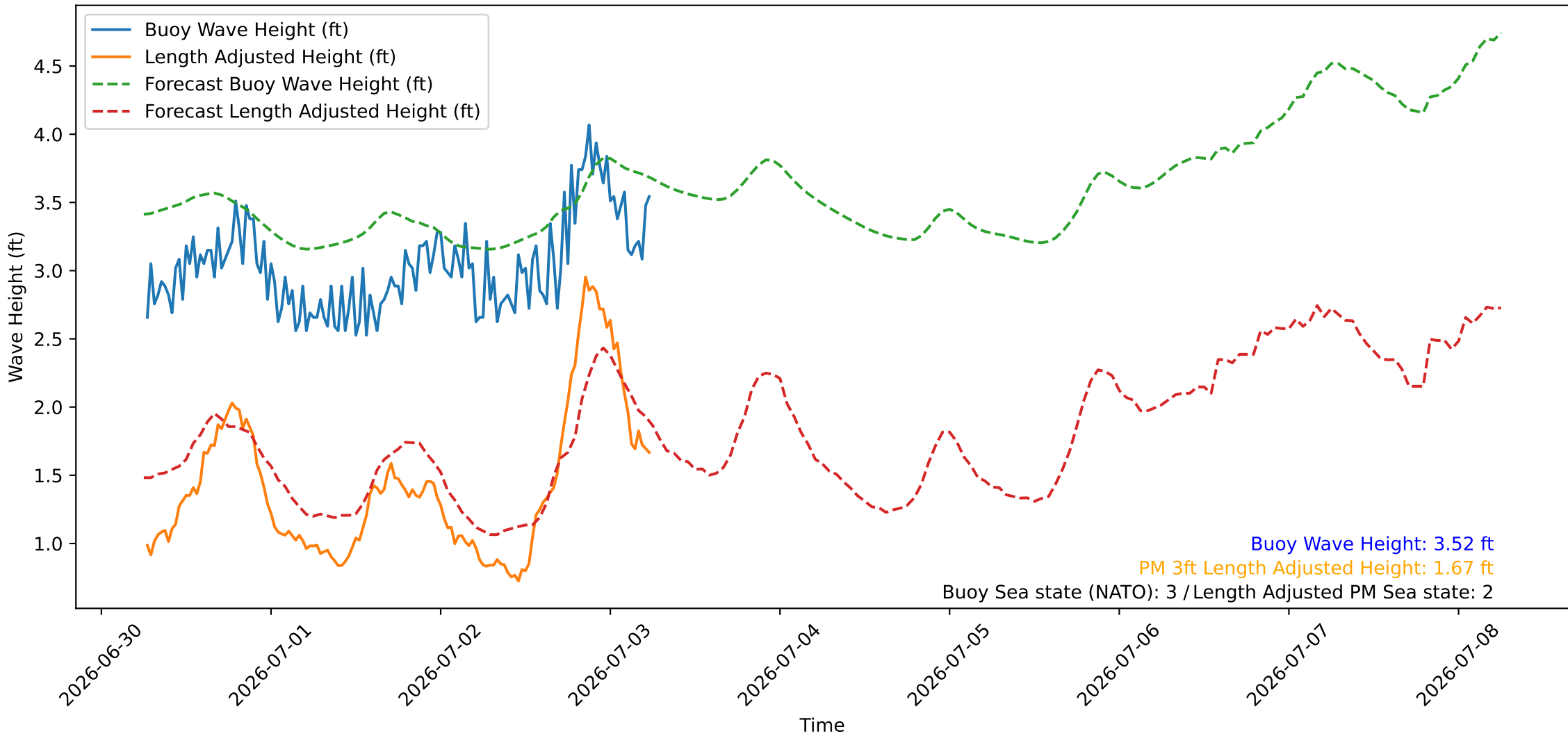
Wave Heights over Time for Green Beach at 2026-07-03 06:21:08
