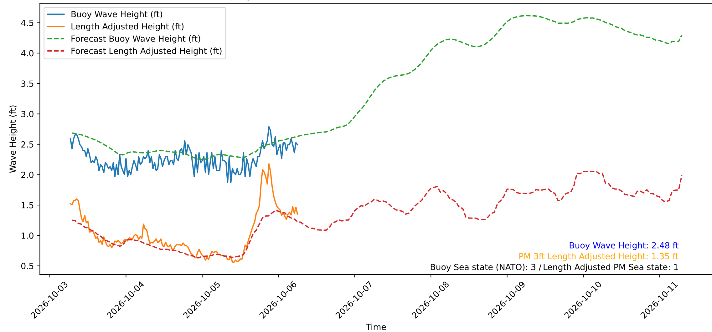
Wave Heights over Time for Oceanside Harbor at 2026-10-06 06:30:30
