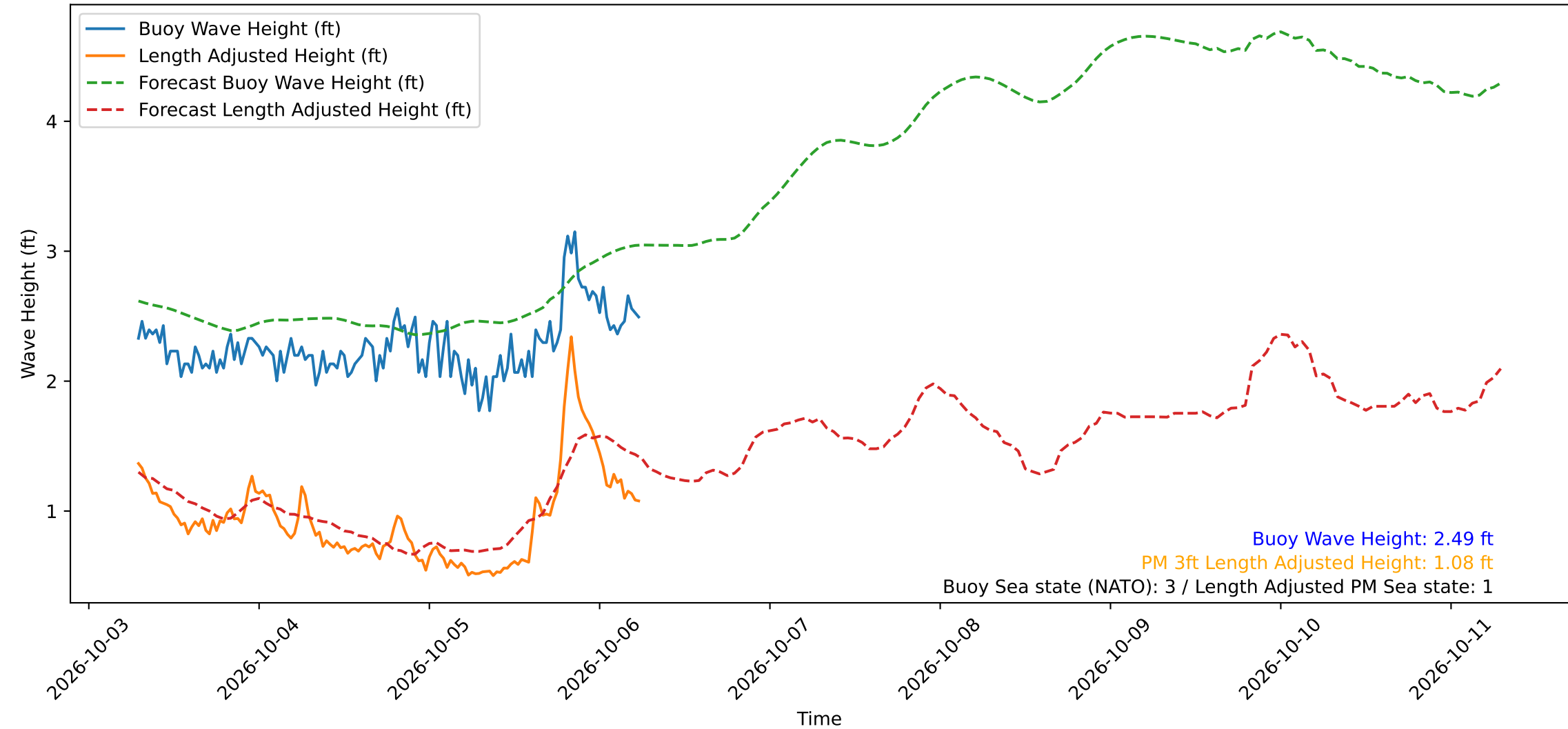
Wave Heights over Time for Green Beach at 2026-10-06 06:31:11
