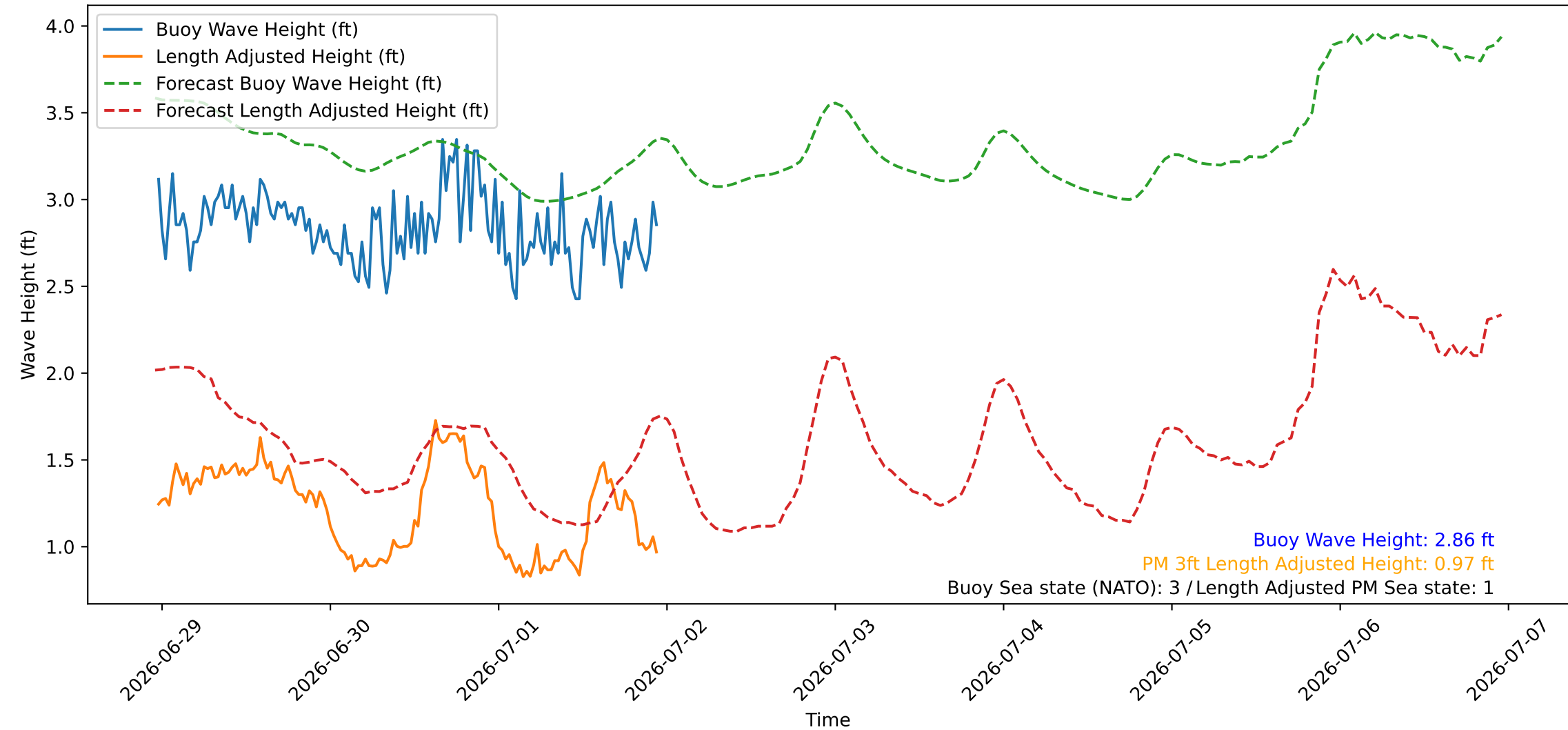
Wave Heights over Time for Red Beach at 2026-07-01 23:10:45
