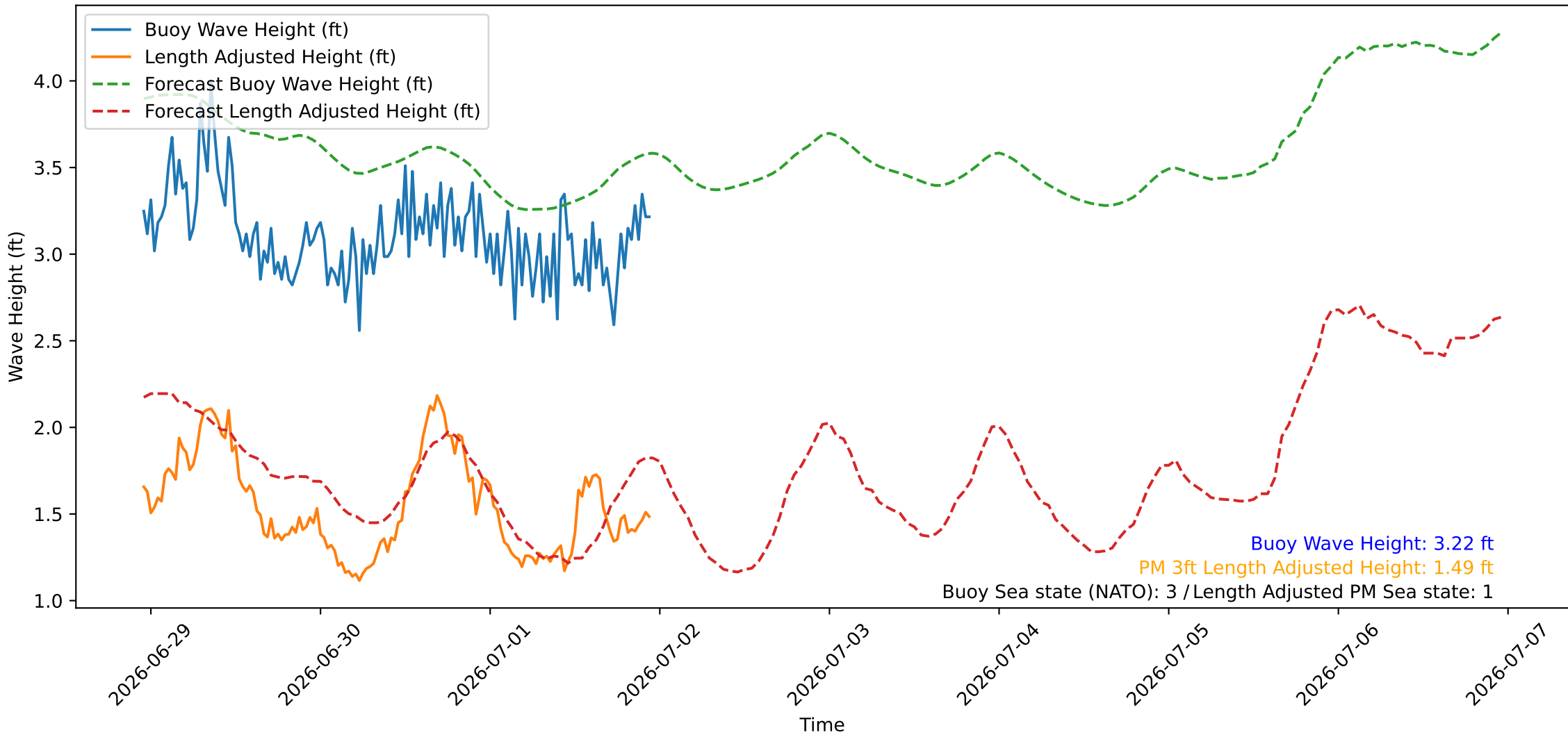
Wave Heights over Time for Oceanside Harbor at 2026-07-01 23:10:26
